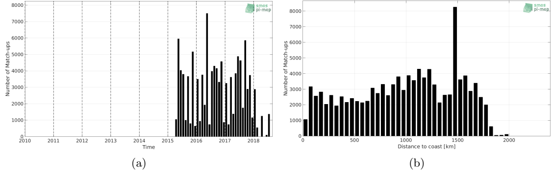
Figure 1: Number of match-ups between TSG-LEGOS-DM and SMAP-L3-RSS-V3-8DAY-RUNNING-40KM SSS as a function of time (a) and as function of the distance to coast (b) over the Amazon and Orinoco river plumes Pi-MEP region and for the full satellite product period.
