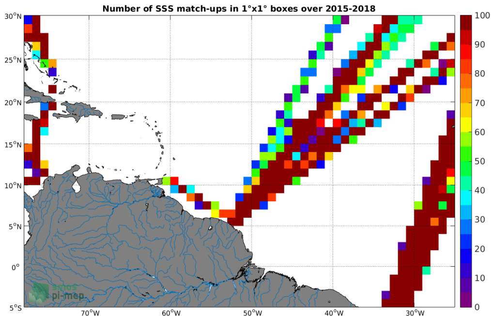
Figure 4: Number of SSS match-ups between TSG-LEGOS-DM SSS and the SMAP-L3-RSS-V3-8DAY-RUNNING-40KM SSS product for the Amazon and Orinoco river plumes Pi-MEP region over 1^\circ \times 1^\circ boxes and for the full satellite product period.
