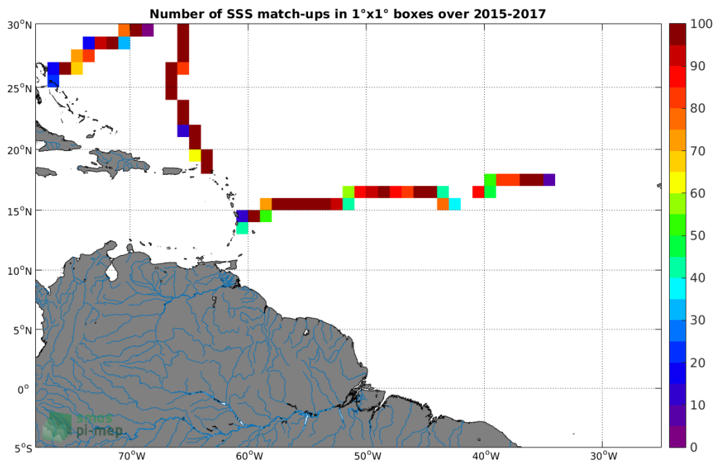
Figure 4: Number of SSS match-ups between TSG-GOSUD-Sailing-ship SSS and the SMAP-L3-RSS-V3-8DAY-RUNNING-40KM SSS product for the Amazon and Orinoco river plumes Pi-MEP region over 1°x1° boxes and for the full satellite product period.
