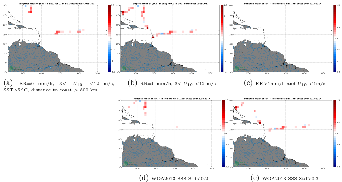
Figure 12: Temporal mean gridded over spatial boxes of size 1^\circ \times 1^\circ of \Delta SSS (SMAP-L3-RSS-V3-8DAY-RUNNING-40KM - TSG-GOSUD-Sailing-ship) for 5 different subdatasets corresponding to:RR=0 mm/h, 3 < U_{10} < 12 m/s, SST >5^\circ\text{C} , distance to coast > 800 km (a), RR=0 mm/h, 3 < U_{10} < 12 m/s (b), RR >1 mm/h and U_{10} < 4 m/s (c), WOA2013 SSS Std <0.2 (d), WOA2013 SSS Std >0.2 (e).
