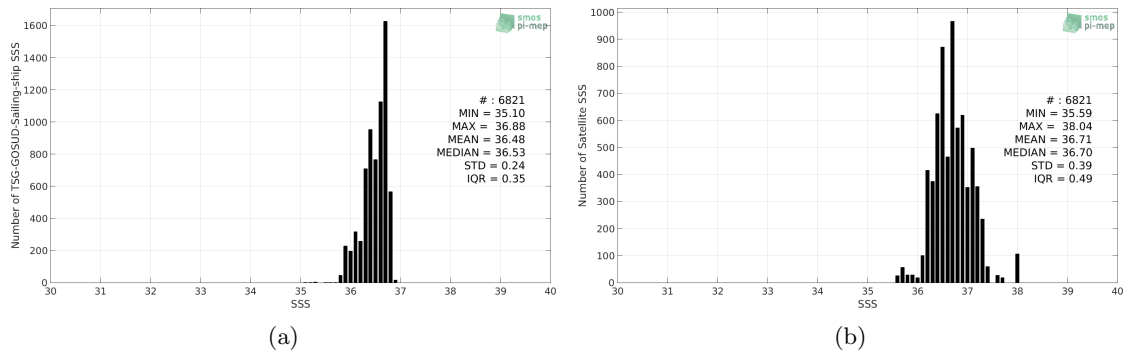
Figure 2: Histograms of SSS from TSG-GOSUD-Sailing-ship (a) and SMAP-L3-RSS-V3-8DAY-RUNNING-40KM (b) considering all match-up pairs per bins of 0.1 over the Amazon and Orinoco river plumes Pi-MEP region and for the full satellite product period.
