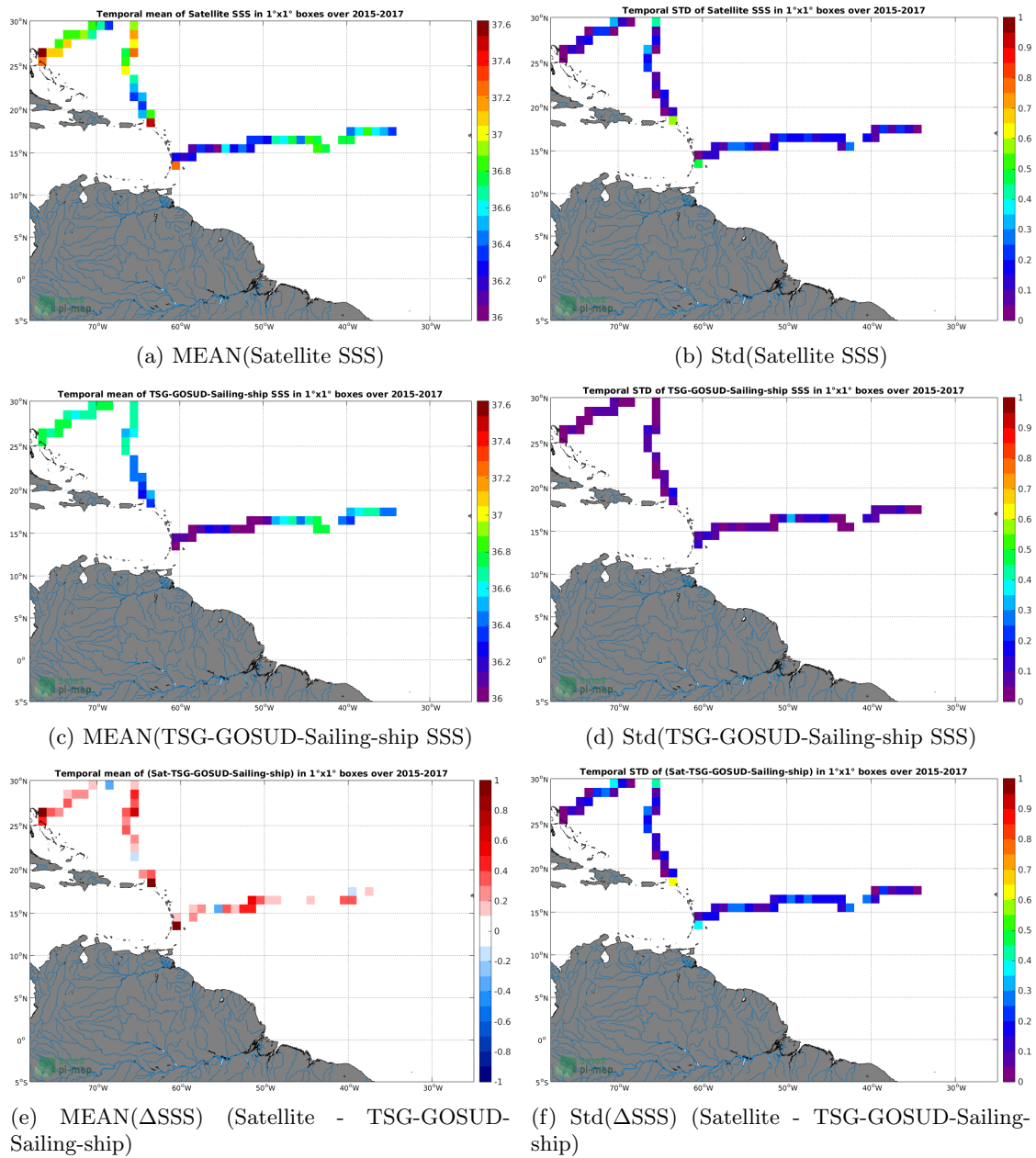
Figure 6: Temporal mean (left) and Std (right) of SSS from SMAP-L3-RSS-V3-8DAY-RUNNING-40KM (top), TSG-GOSUD-Sailing-ship (middle), and of \Delta SSS (Satellite - TSG-GOSUD-Sailing-ship). Only match-up pairs are used to generate these maps.
