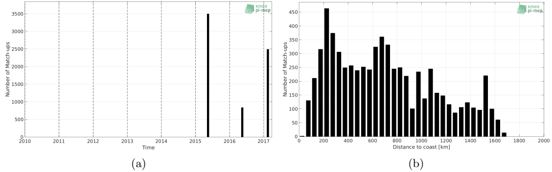
Figure 1: Number of match-ups between TSG-GOSUD-Sailing-ship and SMAP-L3-RSS-V3-8DAY-RUNNING-40KM SSS as a function of time (a) and as function of the distance to coast (b) over the Amazon and Orinoco river plumes Pi-MEP region and for the full satellite product period.
