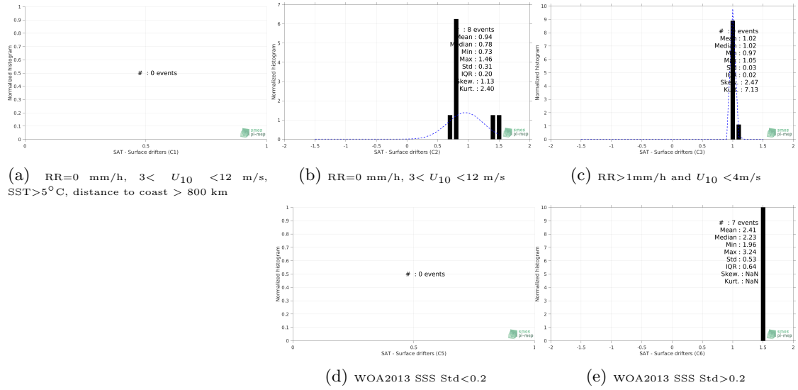
Figure 12: Normalized histogram of \Delta SSS (SMAP-L3-RSS-V3-8DAY-RUNNING-40KM - Surface drifters) for 5 different subdatasets corresponding to: RR=0 mm/h, 3 < U_{10} < 12 m/s, SST>5°C, distance to coast > 800 km (a), RR=0 mm/h, 3 < U_{10} < 12 m/s (b), RR>1mm/h and U_{10} < 4 m/s (c), WOA2013 SSS Std<0.2 (d), WOA2013 SSS Std>0.2 (e).
