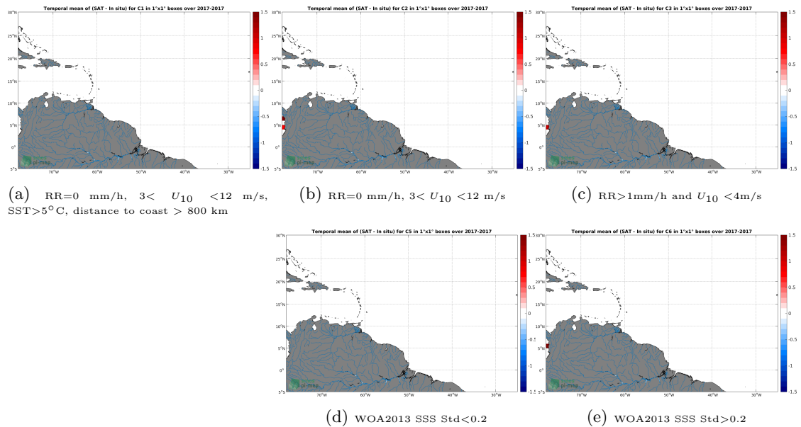
Figure 11: Temporal mean gridded over spatial boxes of size 1^\circ \times 1^\circ of \Delta SSS (SMAP-L3-RSS-V3-8DAY-RUNNING-40KM - Surface drifters) for 5 different subdatasets corresponding to:RR=0 mm/h, 3 < U_{10} < 12 m/s, SST >5^\circ\text{C} , distance to coast > 800 km (a), RR=0 mm/h, 3 < U_{10} < 12 m/s (b), RR >1 mm/h and U_{10} < 4 m/s (c), WOA2013 SSS Std <0.2 (d), WOA2013 SSS Std >0.2 (e).
