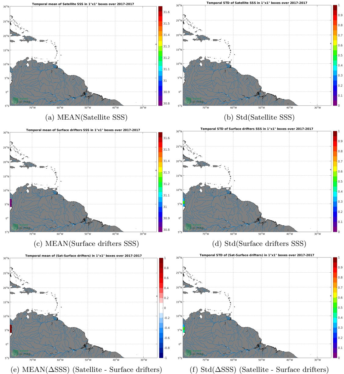
Figure 5: Temporal mean (left) and Std (right) of SSS from SMAP-L3-RSS-V3-8DAY-RUNNING-40KM (top), Surface drifters (middle), and of \Delta SSS (Satellite - Surface drifters). Only match-up pairs are used to generate these maps.
