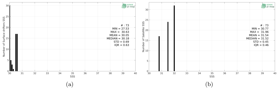
Figure 2: Histograms of SSS from Surface drifters (a) and SMAP-L3-RSS-V3-8DAY-RUNNING-40KM (b) considering all match-up pairs per bins of 0.1 over the Amazon and Orinoco river plumes Pi-MEP region and for the full satellite product period.
