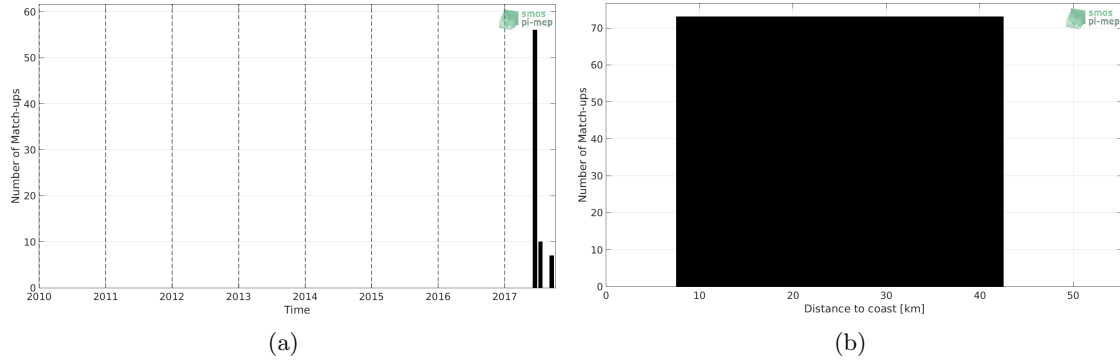
Figure 1: Number of match-ups between Surface drifters and SMAP-L3-RSS-V3-8DAY-RUNNING-40KM SSS as a function of time (a) and as function of the distance to coast (b) over the Amazon and Orinoco river plumes Pi-MEP region and for the full satellite product period.
