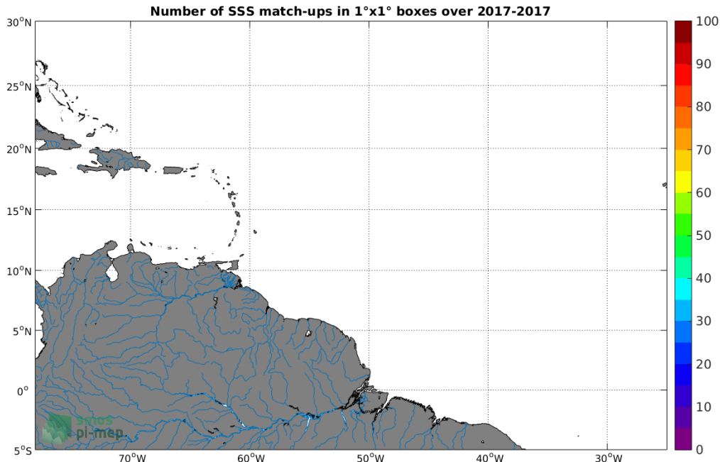
Figure 3: Number of SSS match-ups between Surface drifters SSS and the SMAP-L3-RSS-V3-8DAY-RUNNING-40KM SSS product for the Amazon and Orinoco river plumes Pi-MEP region over 1°x1° boxes and for the full satellite product period.
