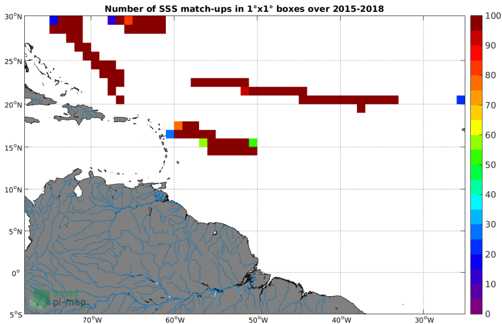
Figure 4: Number of SSS match-ups between TSG-SAMOS SSS and the SMAP-L3-RSS-V3-MONTHLY-70KM SSS product for the Amazon and Orinoco river plumes Pi-MEP region over 1^\circ \times 1^\circ boxes and for the full satellite product period.
