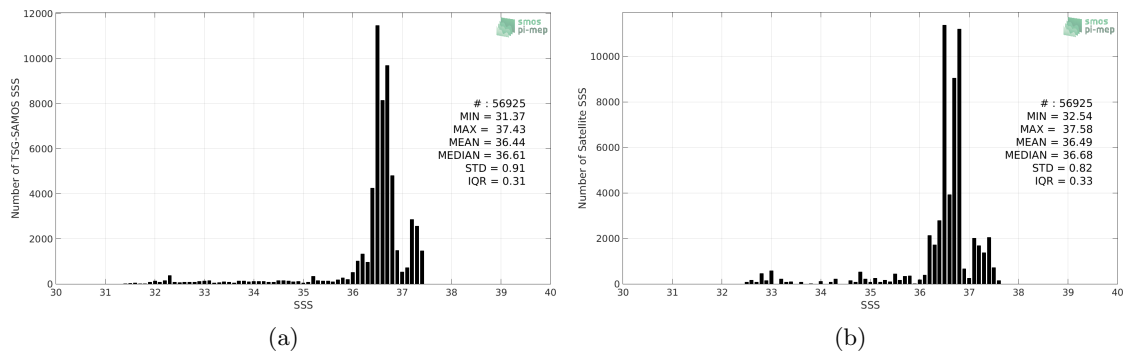
Figure 2: Histograms of SSS from TSG-SAMOS (a) and SMAP-L3-RSS-V3-MONTHLY-70KM (b) considering all match-up pairs per bins of 0.1 over the Amazon and Orinoco river plumes Pi-MEP region and for the full satellite product period.
