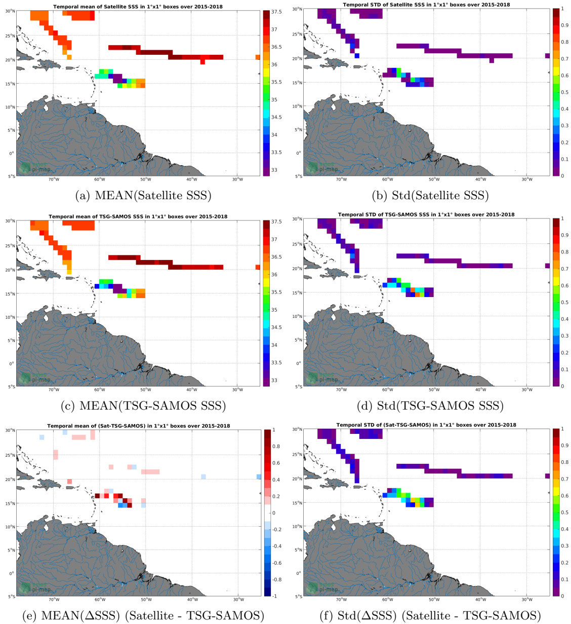
Figure 6: Temporal mean (left) and Std (right) of SSS from SMAP-L3-RSS-V3-MONTHLY-70KM (top), TSG-SAMOS (middle), and of \Delta SSS (Satellite - TSG-SAMOS). Only match-up pairs are used to generate these maps.
