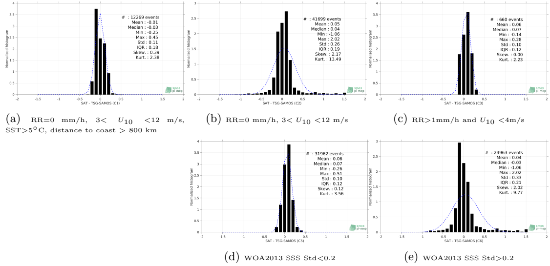
Figure 13: Normalized histogram of \Delta SSS (SMAP-L3-RSS-V3-MONTHLY-70KM - TSG-SAMOS) for 5 different subdatasets corresponding to: RR=0 mm/h, 3 < U_{10} < 12 m/s, SST>5°C, distance to coast > 800 km (a), RR=0 mm/h, 3 < U_{10} < 12 m/s (b), RR>1mm/h and U_{10} < 4 m/s (c), WOA2013 SSS Std<0.2 (d), WOA2013 SSS Std>0.2 (e).
