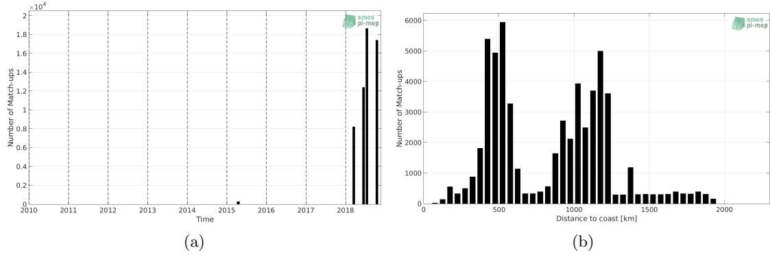
Figure 1: Number of match-ups between TSG-SAMOS and SMAP-L3-RSS-V3-MONTHLY-70KM SSS as a function of time (a) and as function of the distance to coast (b) over the Amazon and Orinoco river plumes Pi-MEP region and for the full satellite product period.
