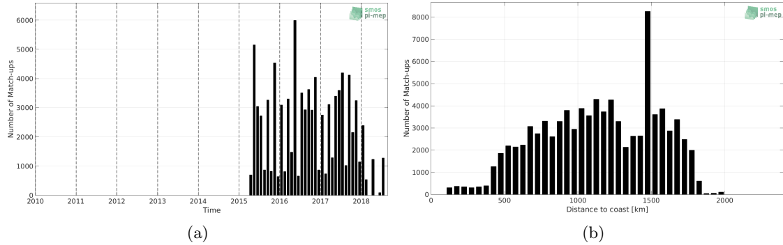
Figure 1: Number of match-ups between TSG-LEGOS-DM and SMAP-L3-RSS-V3-MONTHLY-70KM SSS as a function of time (a) and as function of the distance to coast (b) over the Amazon and Orinoco river plumes Pi-MEP region and for the full satellite product period.
