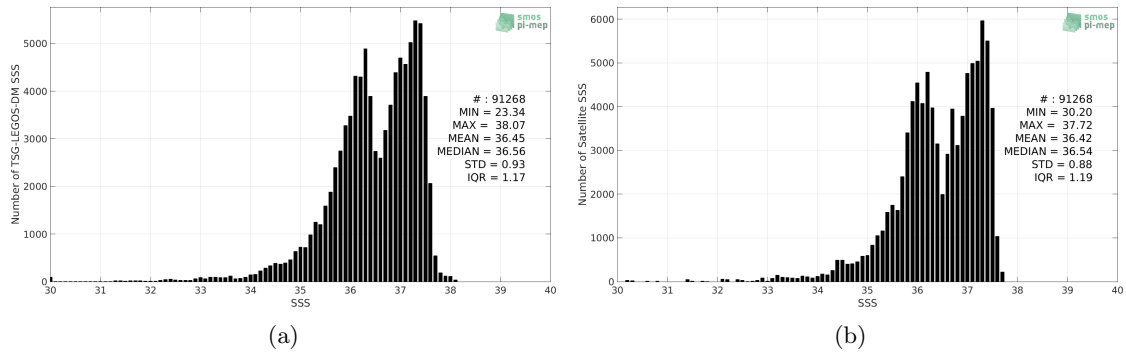
Figure 2: Histograms of SSS from TSG-LEGOS-DM (a) and SMAP-L3-RSS-V3-MONTHLY-70KM (b) considering all match-up pairs per bins of 0.1 over the Amazon and Orinoco river plumes Pi-MEP region and for the full satellite product period.
