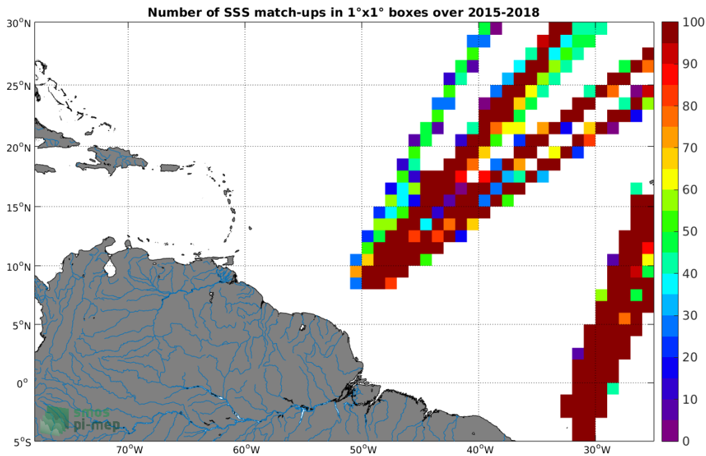
Figure 4: Number of SSS match-ups between TSG-LEGOS-DM SSS and the SMAP-L3-RSS-V3-MONTHLY-70KM SSS product for the Amazon and Orinoco river plumes Pi-MEP region over 1^\circ \times 1^\circ boxes and for the full satellite product period.
