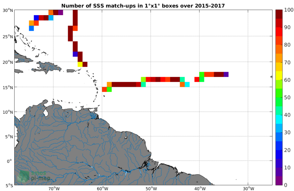
Figure 4: Number of SSS match-ups between TSG-GOSUD-Sailing-ship SSS and the SMAP-L3-RSS-V3-MONTHLY-70KM SSS product for the Amazon and Orinoco river plumes Pi-MEP region over 1°x1° boxes and for the full satellite product period.
