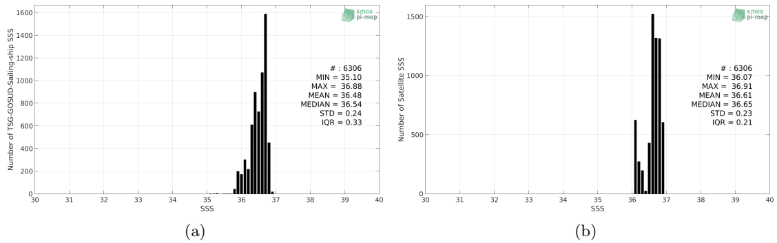
Figure 2: Histograms of SSS from TSG-GOSUD-Sailing-ship (a) and SMAP-L3-RSS-V3-MONTHLY-70KM (b) considering all match-up pairs per bins of 0.1 over the Amazon and Orinoco river plumes Pi-MEP region and for the full satellite product period.
