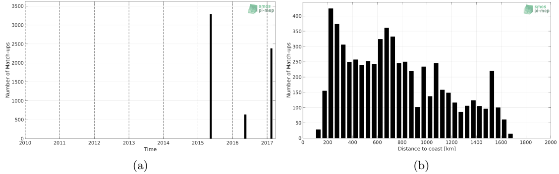
Figure 1: Number of match-ups between TSG-GOSUD-Sailing-ship and SMAP-L3-RSS-V3-MONTHLY-70KM SSS as a function of time (a) and as function of the distance to coast (b) over the Amazon and Orinoco river plumes Pi-MEP region and for the full satellite product period.
