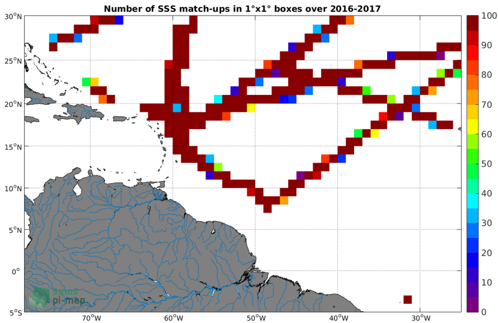
Figure 4: Number of SSS match-ups between TSG-GOSUD-Research-vessel SSS and the SMAP-L3-RSS-V3-MONTHLY-70KM SSS product for the Amazon and Orinoco river plumes Pi-MEP region over 1^\circ \times 1^\circ boxes and for the full satellite product period.
