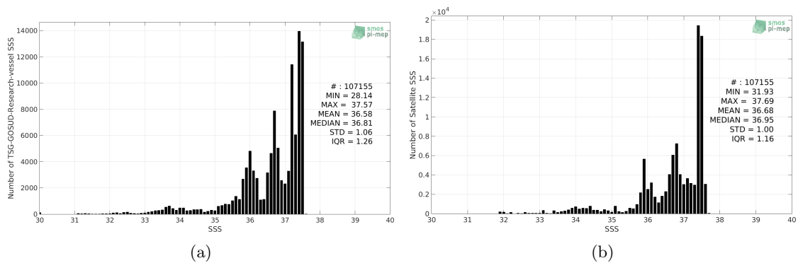
Figure 2: Histograms of SSS from TSG-GOSUD-Research-vessel (a) and SMAP-L3-RSS-V3-MONTHLY-70KM (b) considering all match-up pairs per bins of 0.1 over the Amazon and Orinoco river plumes Pi-MEP region and for the full satellite product period.
