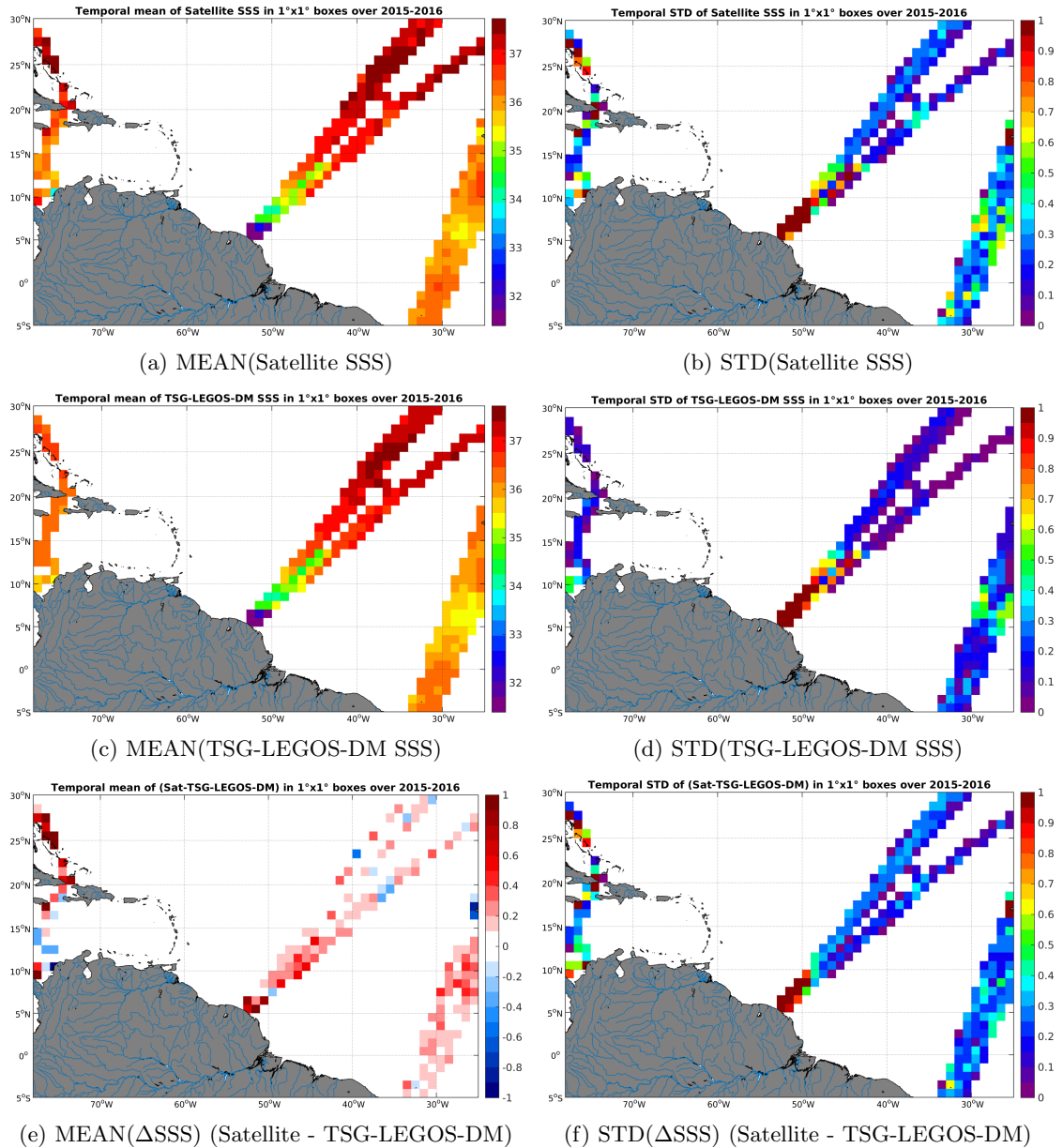
Figure 6: Temporal mean (left) and STD (right) of SSS from SMAP-L3-RSS-V2-8DAY-RUNNING-40KM (top), TSG-LEGOS-DM (middle), and of \Delta SSS (Satellite - TSG-LEGOS-DM). Only match-up pairs are used to generate these maps.
