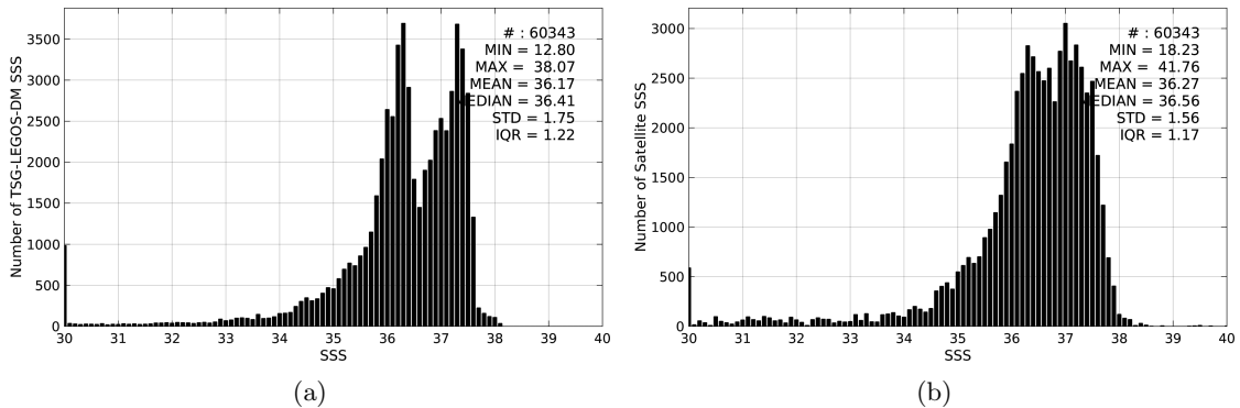
Figure 2: Histograms of SSS from TSG-LEGOS-DM (a) and SMAP-L3-RSS-V2-8DAY-RUNNING-40KM (b) considering all match-up pairs per bins of 0.1 over the Amazon and Orinoco river plumes Pi-MEP region and for the full satellite product period.
