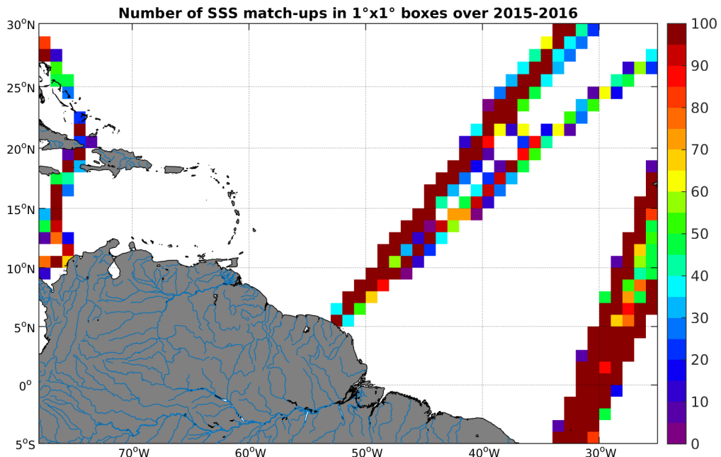
Figure 4: Number of SSS match-ups between TSG-LEGOS-DM SSS and the SMAP-L3-RSS-V2-8DAY-RUNNING-40KM SSS product for the Amazon and Orinoco river plumes Pi-MEP region over 1^\circ \times 1^\circ boxes and for the full satellite product period.
