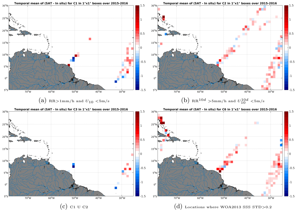
Figure 12: Temporal mean gridded over spatial boxes of size 1^\circ \times 1^\circ of \Delta SSS (SMAP-L3-RSS-V2-8DAY-RUNNING-40KM - TSG-LEGOS-DM) for 4 different subdatasets corresponding to:RR>1mm/h and U_{10} < 5 m/s (a), RR^{10d} > 5 mm/h and U_{10}^{10d} < 5 m/s (b), C1 U C2 (c),Locations where WOA2013 SSS STD>0.2 (d).
