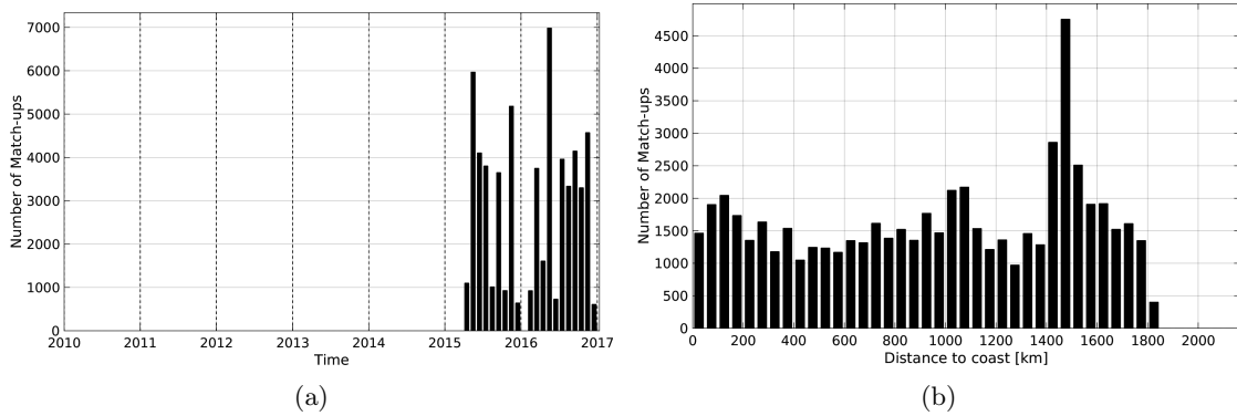
Figure 1: Number of match-ups between TSG-LEGOS-DM and SMAP-L3-RSS-V2-8DAY-RUNNING-40KM SSS as a function of time (a) and as function of the distance to coast (b) over the Amazon and Orinoco river plumes Pi-MEP region and for the full satellite product period.
