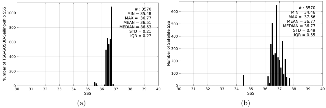
Figure 2: Histograms of SSS from TSG-GOSUD-Sailing-ship (a) and SMAP-L3-RSS-V2-8DAY-RUNNING-40KM (b) considering all match-up pairs per bins of 0.1 over the Amazon and Orinoco river plumes Pi-MEP region and for the full satellite product period.
