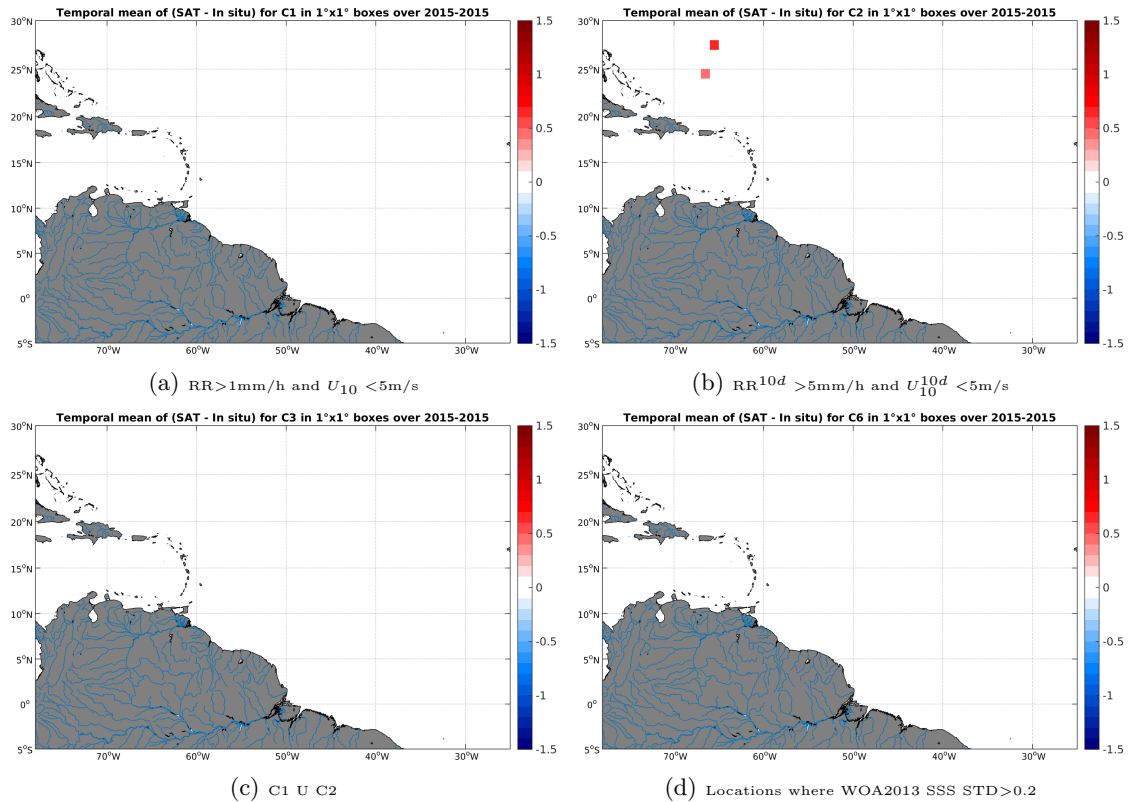
Figure 12: Temporal mean gridded over spatial boxes of size 1^\circ \times 1^\circ of \Delta SSS (SMAP-L3-RSS-V2-8DAY-RUNNING-40KM - TSG-GOSUD-Sailing-ship) for 4 different subdatasets corresponding to: RR > 1\text{mm/h} and U_{10} < 5\text{m/s} (a), RR^{10d} > 5\text{mm/h} and U_{10}^{10d} < 5\text{m/s} (b), C1 U C2 (c), Locations where WOA2013 SSS STD > 0.2 (d).
