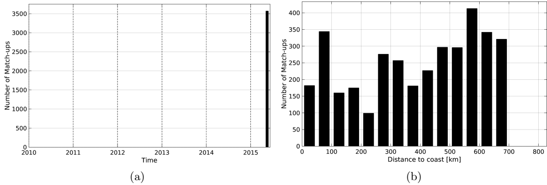
Figure 1: Number of match-ups between TSG-GOSUD-Sailing-ship and SMAP-L3-RSS-V2-8DAY-RUNNING-40KM SSS as a function of time (a) and as function of the distance to coast (b) over the Amazon and Orinoco river plumes Pi-MEP region and for the full satellite product period.
