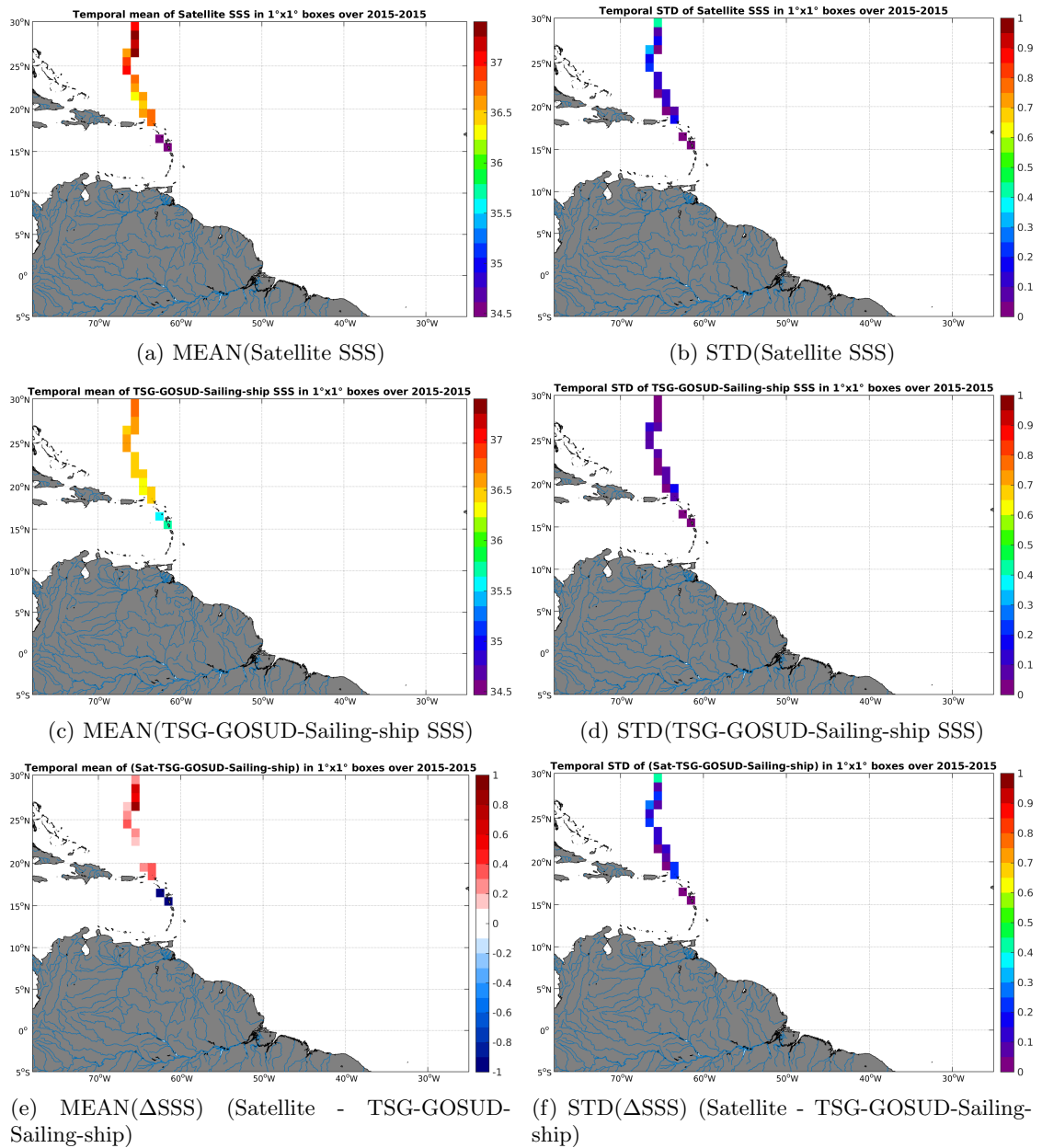
Figure 6: Temporal mean (left) and STD (right) of SSS from SMAP-L3-RSS-V2-8DAY-RUNNING-40KM (top), TSG-GOSUD-Sailing-ship (middle), and of \Delta SSS (Satellite - TSG-GOSUD-Sailing-ship). Only match-up pairs are used to generate these maps.
