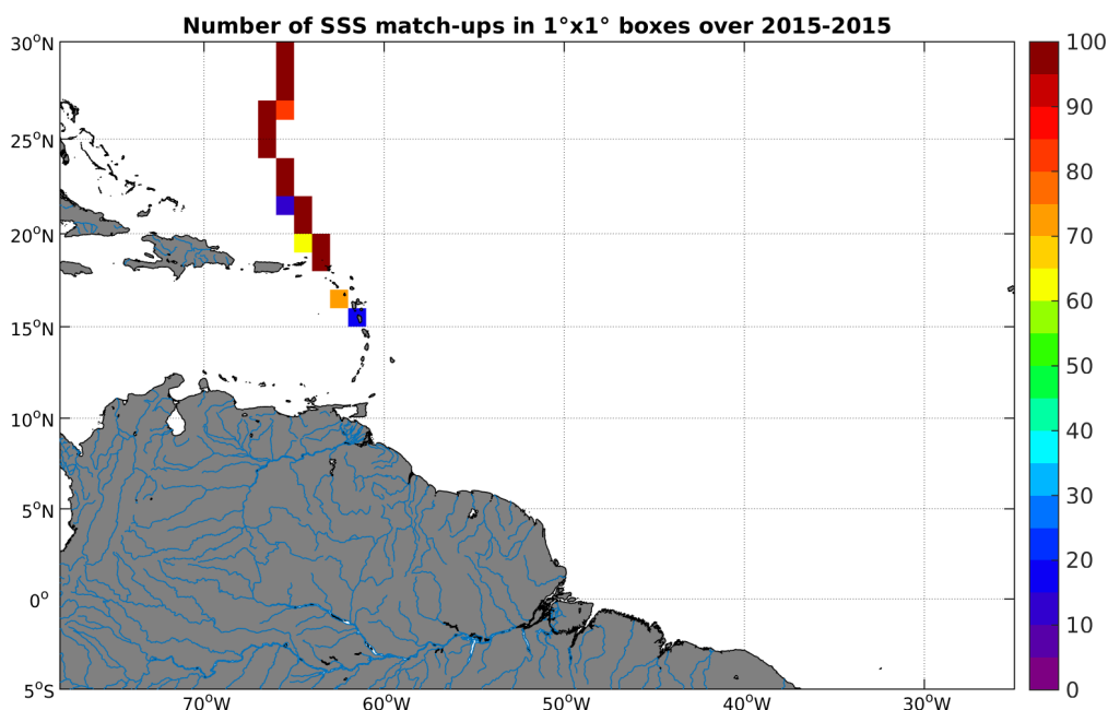
Figure 4: Number of SSS match-ups between TSG-GOSUD-Sailing-ship SSS and the SMAP-L3-RSS-V2-8DAY-RUNNING-40KM SSS product for the Amazon and Orinoco river plumes Pi-MEP region over 1^{\circ} \times 1^{\circ} boxes and for the full satellite product period.
