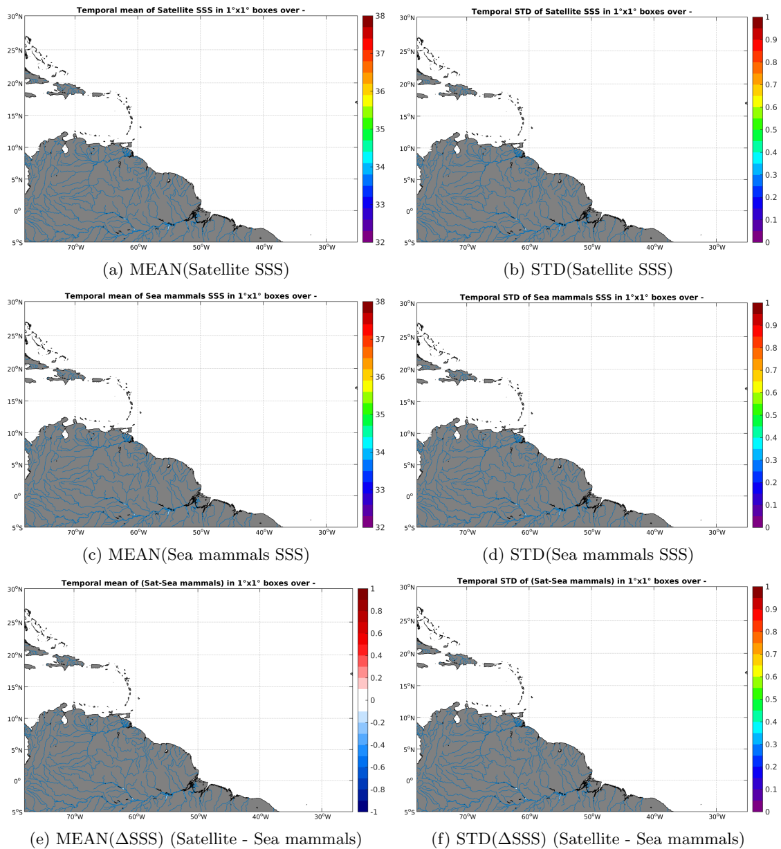
Figure 6: Temporal mean (left) and STD (right) of SSS from SMAP-L3-RSS-V2-8DAY-RUNNING-40KM (top), Sea mammals (middle), and of \Delta SSS (Satellite - Sea mammals). Only match-up pairs are used to generate these maps.
