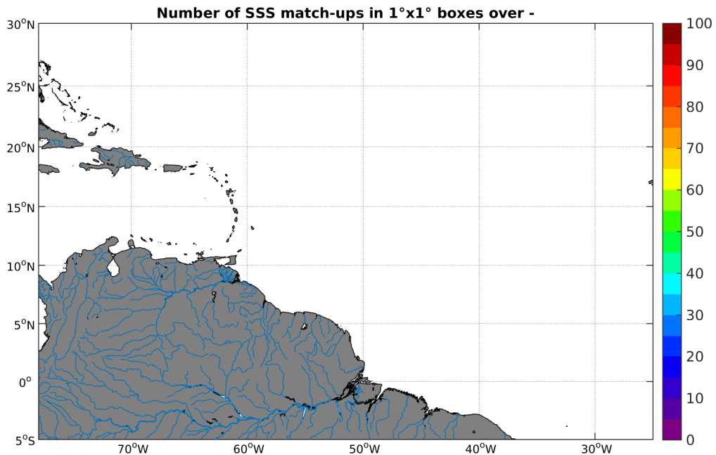
Figure 4: Number of SSS match-ups between Sea mammals SSS and the SMAP-L3-RSS-V2-8DAY-RUNNING-40KM SSS product for the Amazon and Orinoco river plumes Pi-MEP region over 1^\circ \times 1^\circ boxes and for the full satellite product period.
