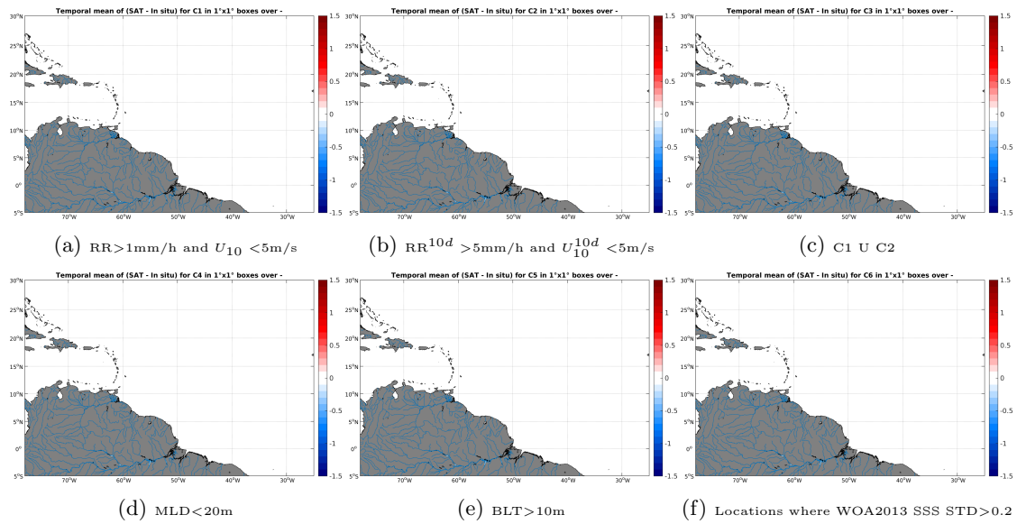
Figure 12: Temporal mean gridded over spatial boxes of size 1^\circ \times 1^\circ of \Delta SSS (SMAP-L3-RSS-V2-8DAY-RUNNING-40KM - Sea mammals) for 6 different subdatasets corresponding to: RR > 1\text{mm/h} and U_{10} < 5\text{m/s} (a), RR^{10d} > 5\text{mm/h} and U_{10}^{10d} < 5\text{m/s} (b), C1 U C2 (c), MLD < 20\text{m} (d), BLT > 10\text{m} (e), Locations where WOA2013 SSS STD > 0.2 (f).
