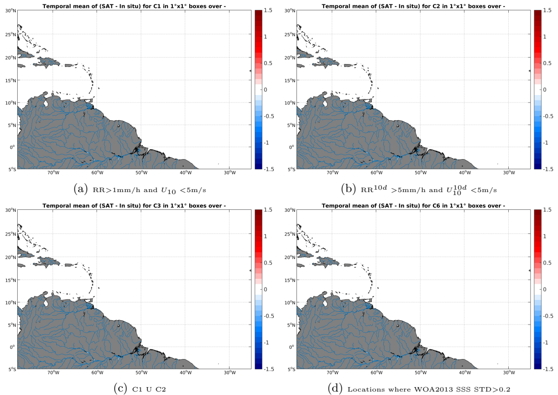
Figure 11: Temporal mean gridded over spatial boxes of size 1^\circ \times 1^\circ of \Delta SSS (SMAP-L3-RSS-V2-8DAY-RUNNING-40KM - Surface drifters) for 4 different subdatasets corresponding to:RR > 1 mm/h and U_{10} < 5 m/s (a), RR^{10d} > 5 mm/h and U_{10}^{10d} < 5 m/s (b), C1 U C2 (c),Locations where WOA2013 SSS STD > 0.2 (d).
