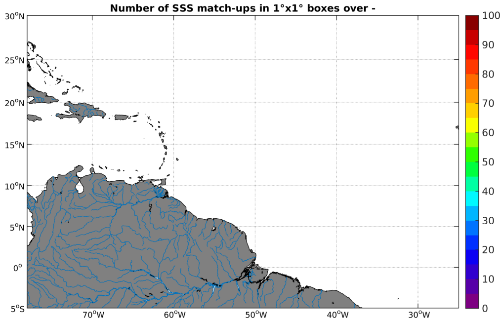
Figure 3: Number of SSS match-ups between Surface drifters SSS and the SMAP-L3-RSS-V2-8DAY-RUNNING-40KM SSS product for the Amazon and Orinoco river plumes Pi-MEP region over 1°x1° boxes and for the full satellite product period.
