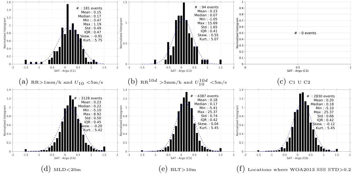
Figure 13: Normalized histogram of \Delta\text{SSS} (SMAP-L3-RSS-V2-8DAY-RUNNING-40KM - Argo) for 6 different subdatasets corresponding to: RR>1mm/h and U_{10} < 5\text{m/s} (a), RR^{10d} > 5\text{mm/h} and U_{10}^{10d} < 5\text{m/s} (b), C1 U C2 (c),MLD<20m (d),BLT>10m (e),Locations where WOA2013 SSS STD>0.2 (f).
