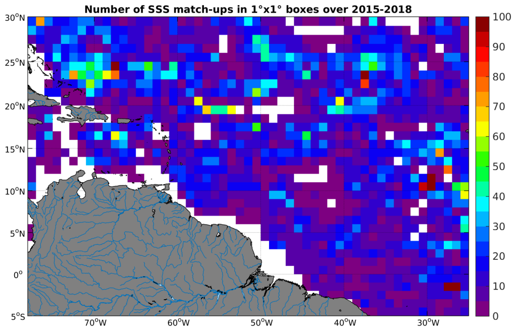
Figure 4: Number of SSS match-ups between Argo SSS and the SMAP-L3-RSS-V2-8DAY-RUNNING-40KM SSS product for the Amazon and Orinoco river plumes Pi-MEP region over 1°x1° boxes and for the full satellite product period.
