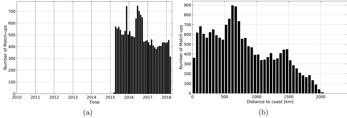
Figure 1: Number of match-ups between Argo and SMAP-L3-RSS-V2-8DAY-RUNNING-40KM SSS as a function of time (a) and as function of the distance to coast (b) over the Amazon and Orinoco river plumes Pi-MEP region and for the full satellite product period.
