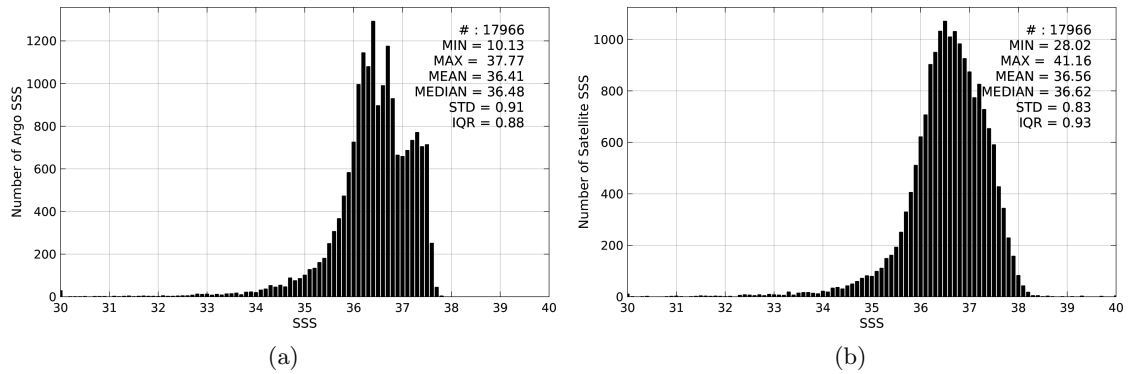
Figure 2: Histograms of SSS from Argo (a) and SMAP-L3-RSS-V2-8DAY-RUNNING-40KM (b) considering all match-up pairs per bins of 0.1 over the Amazon and Orinoco river plumes Pi-MEP region and for the full satellite product period.
