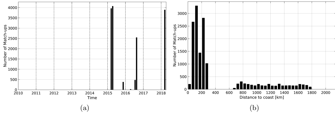
Figure 1: Number of match-ups between TSG-SAMOS and SMAP-L3-RSS-V2-8DAY-RUNNING-70KM SSS as a function of time (a) and as function of the distance to coast (b) over the Amazon and Orinoco river plumes Pi-MEP region and for the full satellite product period.
