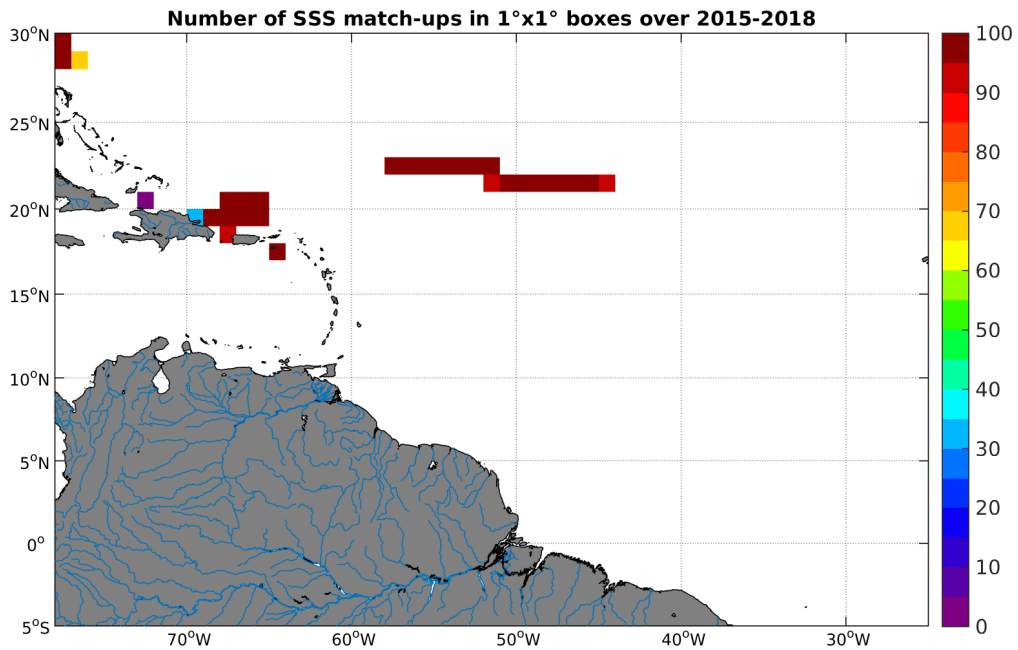
Figure 4: Number of SSS match-ups between TSG-SAMOS SSS and the SMAP-L3-RSS-V2-8DAY-RUNNING-70KM SSS product for the Amazon and Orinoco river plumes Pi-MEP region over 1^\circ \times 1^\circ boxes and for the full satellite product period.
