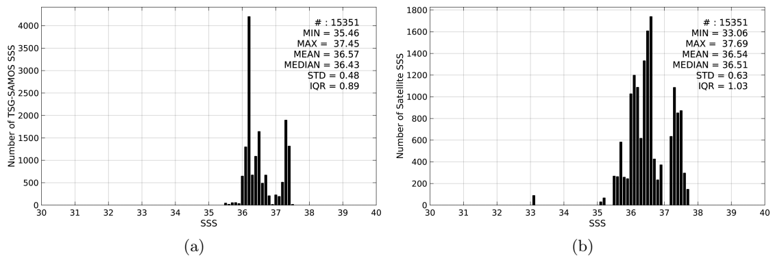
Figure 2: Histograms of SSS from TSG-SAMOS (a) and SMAP-L3-RSS-V2-8DAY-RUNNING-70KM (b) considering all match-up pairs per bins of 0.1 over the Amazon and Orinoco river plumes Pi-MEP region and for the full satellite product period.
