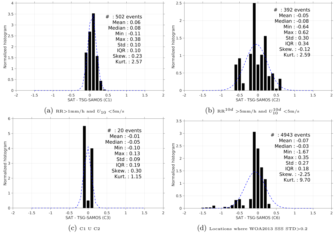
Figure 13: Normalized histogram of \Delta\text{SSS} (SMAP-L3-RSS-V2-8DAY-RUNNING-70KM - TSG-SAMOS) for 6 different subdatasets corresponding to: RR>1mm/h and U_{10} < 5\text{m/s} (a), \text{RR}^{10d} > 5\text{mm/h} and U_{10}^{10d} < 5\text{m/s} (b), C1 U C2 (c), Locations where WOA2013 SSS STD>0.2 (d).
