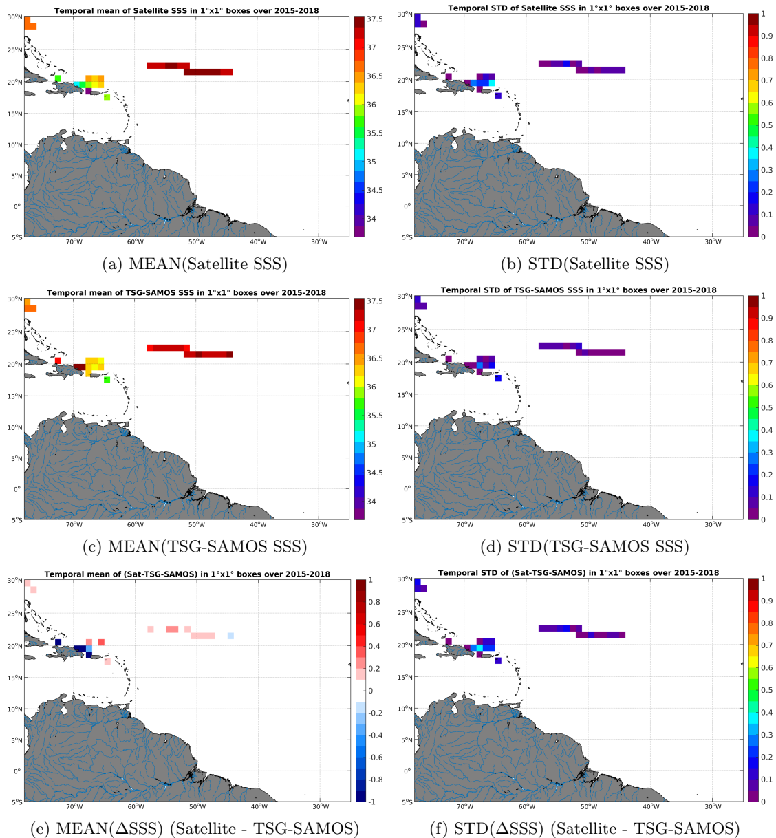
Figure 6: Temporal mean (left) and STD (right) of SSS from SMAP-L3-RSS-V2-8DAY-RUNNING-70KM (top), TSG-SAMOS (middle), and of \Delta SSS (Satellite - TSG-SAMOS). Only match-up pairs are used to generate these maps.
