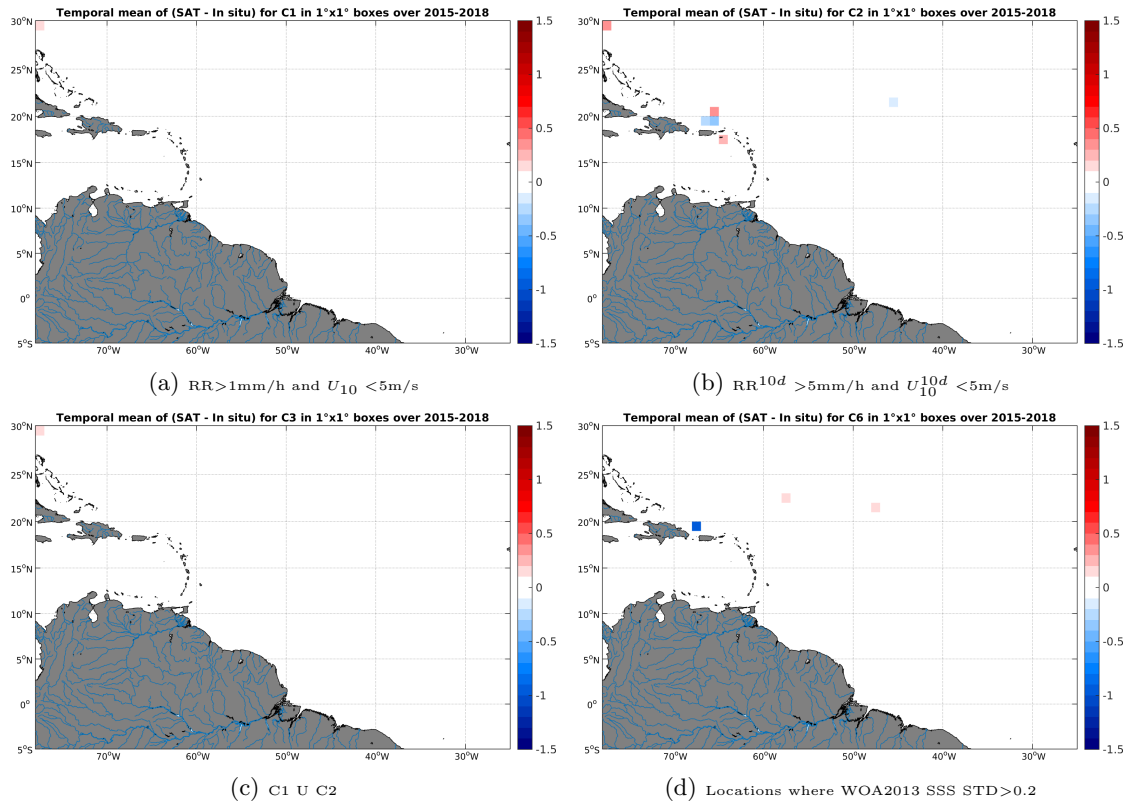
Figure 12: Temporal mean gridded over spatial boxes of size 1^\circ \times 1^\circ of \Delta SSS (SMAP-L3-RSS-V2-8DAY-RUNNING-70KM - TSG-SAMOS) for 4 different subdatasets corresponding to: RR > 1\text{mm/h} and U_{10} < 5\text{m/s} (a), RR^{10d} > 5\text{mm/h} and U_{10}^{10d} < 5\text{m/s} (b), C1 U C2 (c), Locations where WOA2013 SSS STD > 0.2 (d).
