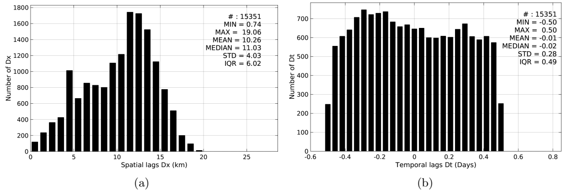
Figure 5: Histograms of the spatial (a) and temporal (b) lags between the time of the TSG-SAMOS measurements and the date of the corresponding SMAP-L3-RSS-V2-8DAY-RUNNING-70KM SSS product.
