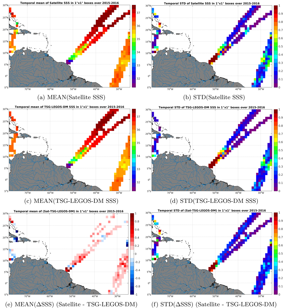
Figure 6: Temporal mean (left) and STD (right) of SSS from SMAP-L3-RSS-V2-8DAY-RUNNING-70KM (top), TSG-LEGOS-DM (middle), and of \Delta SSS (Satellite - TSG-LEGOS-DM). Only match-up pairs are used to generate these maps.
