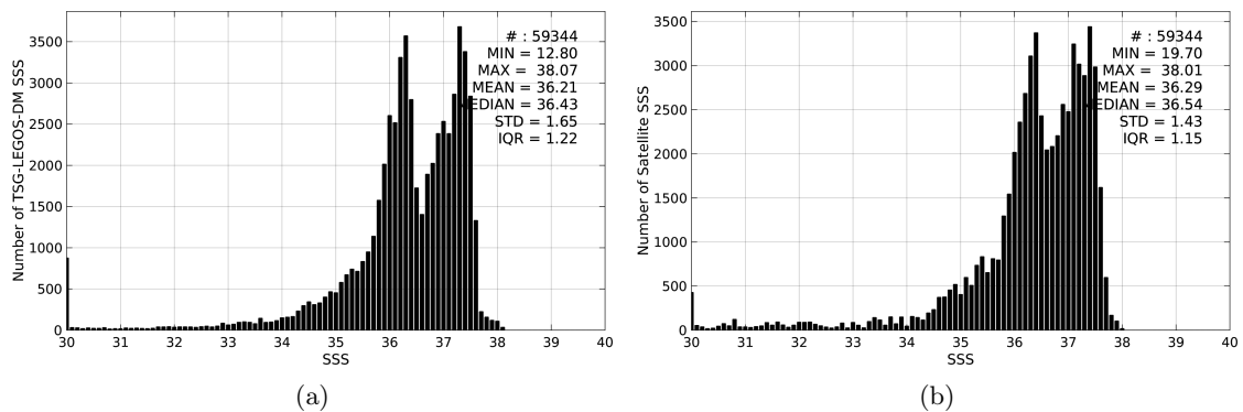
Figure 2: Histograms of SSS from TSG-LEGOS-DM (a) and SMAP-L3-RSS-V2-8DAY-RUNNING-70KM (b) considering all match-up pairs per bins of 0.1 over the Amazon and Orinoco river plumes Pi-MEP region and for the full satellite product period.
