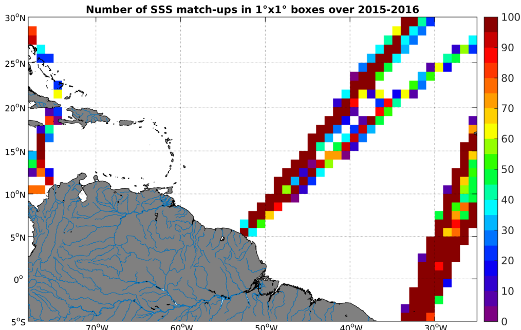
Figure 4: Number of SSS match-ups between TSG-LEGOS-DM SSS and the SMAP-L3-RSS-V2-8DAY-RUNNING-70KM SSS product for the Amazon and Orinoco river plumes Pi-MEP region over 1^\circ \times 1^\circ boxes and for the full satellite product period.
