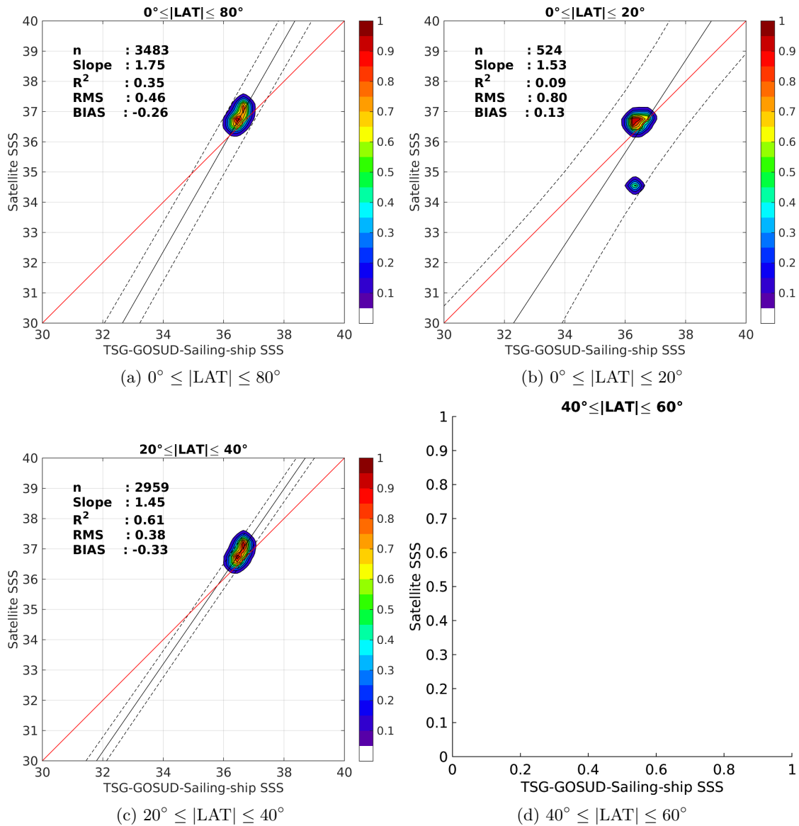
Figure 9: Contour maps of the concentration of SMAP-L3-RSS-V2-8DAY-RUNNING-70KM SSS (y-axis) versus TSG-GOSUD-Sailing-ship SSS (x-axis) at match-up pairs for different latitude bands. For each plot, the red line shows x=y . The black thin and dashed lines indicate a linear fit through the data cloud and the \pm 95\% confidence levels, respectively. The number match-up pairs n , the slope and R^2 coefficient of the linear fit, the root mean square (RMS) and the mean bias between satellite and in situ data are indicated for each latitude band in each plots.
