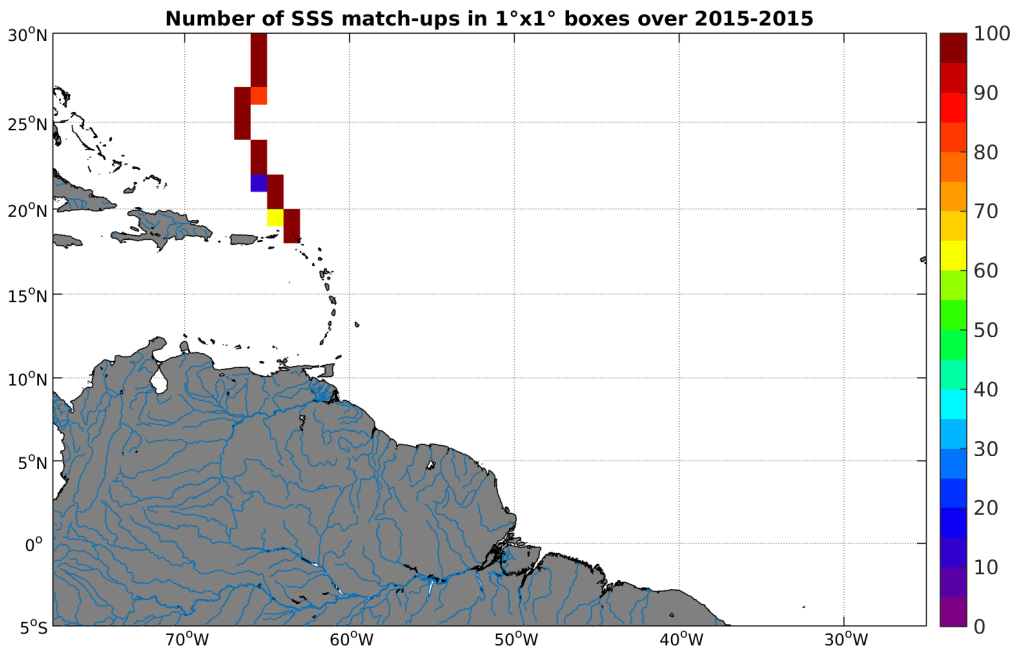
Figure 4: Number of SSS match-ups between TSG-GOSUD-Sailing-ship SSS and the SMAP-L3-RSS-V2-8DAY-RUNNING-70KM SSS product for the Amazon and Orinoco river plumes Pi-MEP region over 1^{\circ} \times 1^{\circ} boxes and for the full satellite product period.
