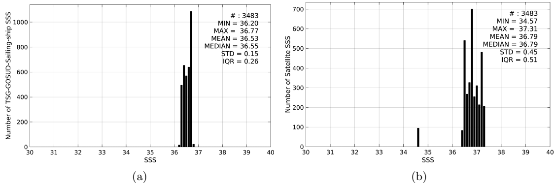
Figure 2: Histograms of SSS from TSG-GOSUD-Sailing-ship (a) and SMAP-L3-RSS-V2-8DAY-RUNNING-70KM (b) considering all match-up pairs per bins of 0.1 over the Amazon and Orinoco river plumes Pi-MEP region and for the full satellite product period.
