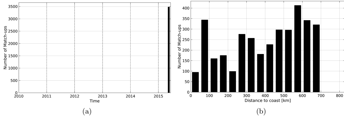
Figure 1: Number of match-ups between TSG-GOSUD-Sailing-ship and SMAP-L3-RSS-V2-8DAY-RUNNING-70KM SSS as a function of time (a) and as function of the distance to coast (b) over the Amazon and Orinoco river plumes Pi-MEP region and for the full satellite product period.
