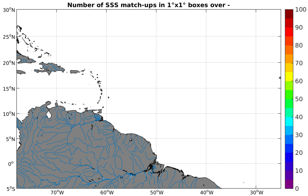
Figure 3: Number of SSS match-ups between Surface drifters SSS and the SMAP-L3-RSS-V2-8DAY-RUNNING-70KM SSS product for the Amazon and Orinoco river plumes Pi-MEP region over 1°x1° boxes and for the full satellite product period.
