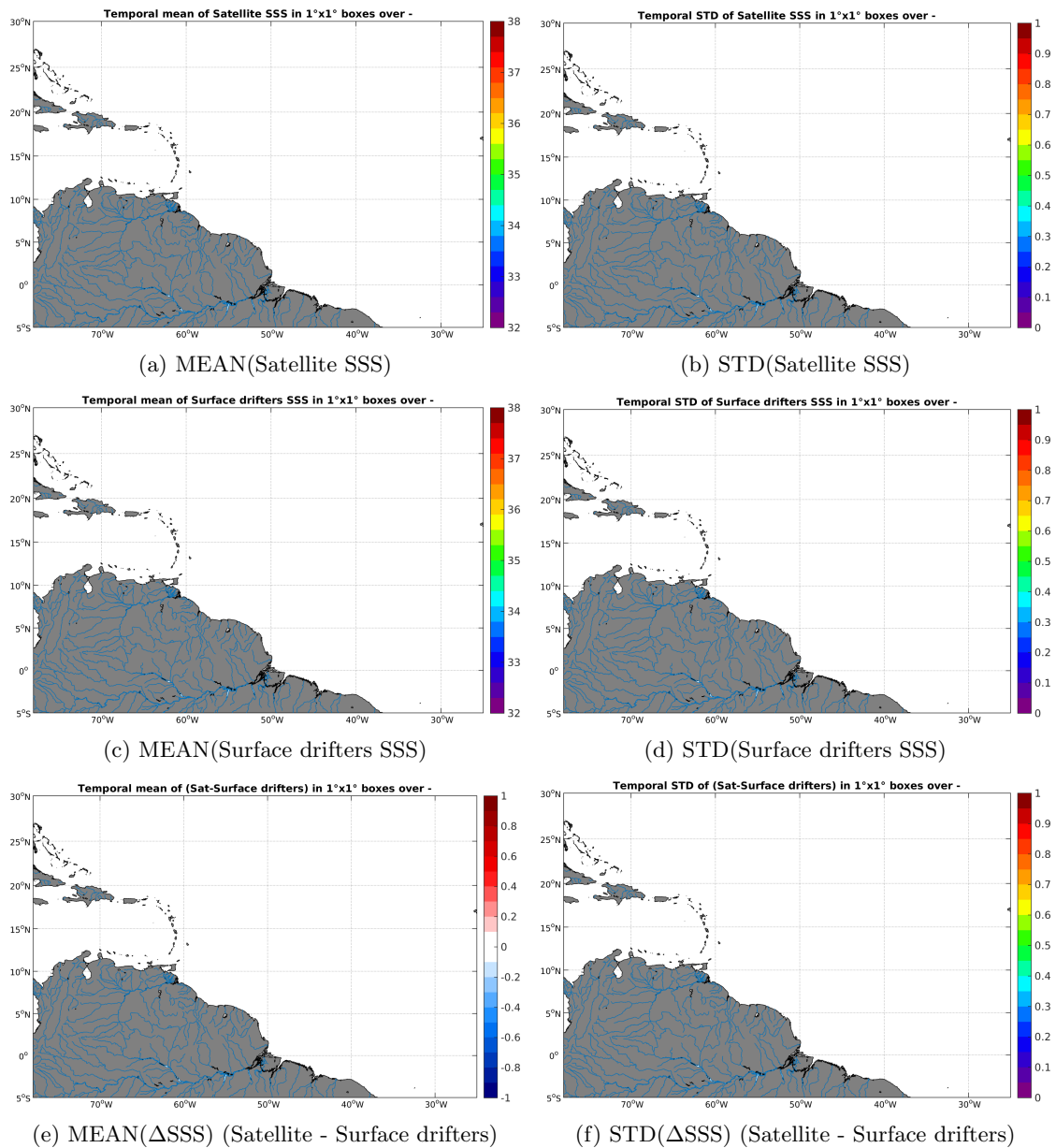
Figure 5: Temporal mean (left) and STD (right) of SSS from SMAP-L3-RSS-V2-8DAY-RUNNING-70KM (top), Surface drifters (middle), and of \Delta SSS (Satellite - Surface drifters). Only match-up pairs are used to generate these maps.
