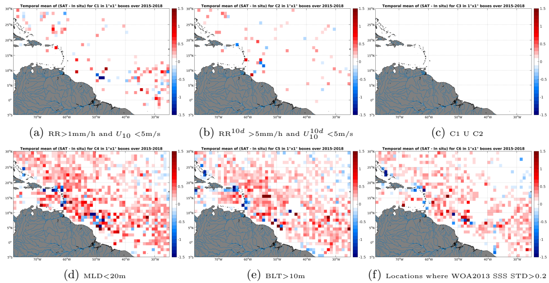
Figure 12: Temporal mean gridded over spatial boxes of size 1^\circ \times 1^\circ of \Delta SSS (SMAP-L3-RSS-V2-8DAY-RUNNING-70KM - Argo) for 6 different subdatasets corresponding to:RR>1mm/h and U_{10} < 5\text{m/s} (a), RR^{10d} > 5\text{mm/h} and U_{10}^{10d} < 5\text{m/s} (b), C1 U C2 (c),MLD<20m (d),BLT>10m (e),Locations where WOA2013 SSS STD>0.2 (f).
