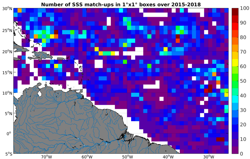
Figure 4: Number of SSS match-ups between Argo SSS and the SMAP-L3-RSS-V2-8DAY-RUNNING-70KM SSS product for the Amazon and Orinoco river plumes Pi-MEP region over 1°x1° boxes and for the full satellite product period.
