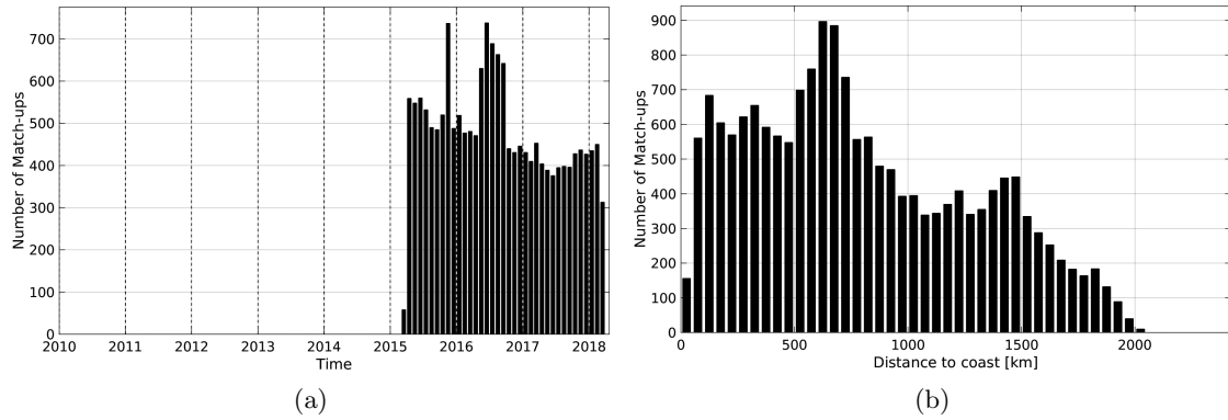
Figure 1: Number of match-ups between Argo and SMAP-L3-RSS-V2-8DAY-RUNNING-70KM SSS as a function of time (a) and as function of the distance to coast (b) over the Amazon and Orinoco river plumes Pi-MEP region and for the full satellite product period.
