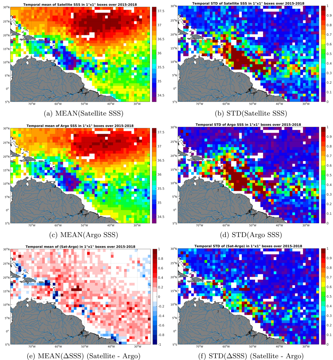
Figure 6: Temporal mean (left) and STD (right) of SSS from SMAP-L3-RSS-V2-8DAY-RUNNING-70KM (top), Argo (middle), and of \Delta SSS (Satellite - Argo). Only match-up pairs are used to generate these maps.
