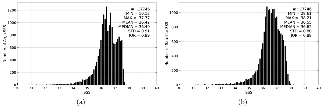
Figure 2: Histograms of SSS from Argo (a) and SMAP-L3-RSS-V2-8DAY-RUNNING-70KM (b) considering all match-up pairs per bins of 0.1 over the Amazon and Orinoco river plumes Pi-MEP region and for the full satellite product period.
