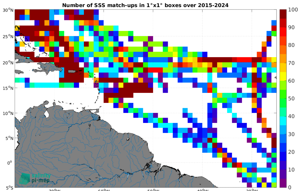
Figure 5: Number of SSS match-ups between TSG (SAMOS) SSS and the SMAP SSS L3 v5.0 - 8-Day running (JPL) SSS product for the Amazon and Orinoco river plumes Pi-MEP region over 1^\circ \times 1^\circ boxes and for the full satellite product period.
