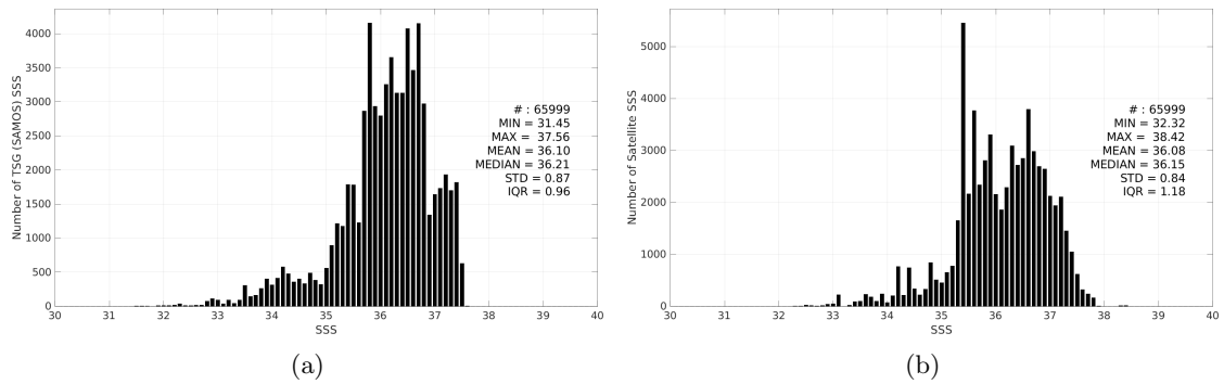
Figure 3: Histograms of SSS from TSG (SAMOS) (a) and SMAP SSS L3 v5.0 - 8-Day running (JPL) (b) considering all match-up pairs per bins of 0.1 over the Amazon and Orinoco river plumes Pi-MEP region and for the full satellite product period.
