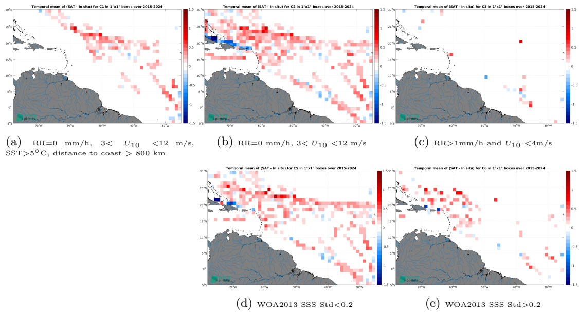
Figure 14: Temporal mean gridded over spatial boxes of size 1^\circ \times 1^\circ of \Delta SSS (SMAP SSS L3 v5.0 - 8-Day running (JPL) - TSG (SAMOS)) for 5 different subdatasets corresponding to:RR=0 mm/h, 3 < U_{10} < 12 m/s, SST >5^\circ\text{C} , distance to coast > 800 km (a), RR=0 mm/h, 3 < U_{10} < 12 m/s (b), RR >1 mm/h and U_{10} < 4 m/s (c), WOA2013 SSS Std <0.2 (d), WOA2013 SSS Std >0.2 (e).
