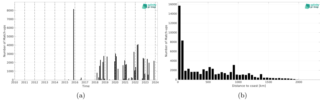
Figure 2: Number of match-ups between TSG (SAMOS) and SMAP SSS L3 v5.0 - 8-Day running (JPL) SSS as a function of time (a) and as function of the distance to coast (b) over the Amazon and Orinoco river plumes Pi-MEP region and for the full satellite product period.
