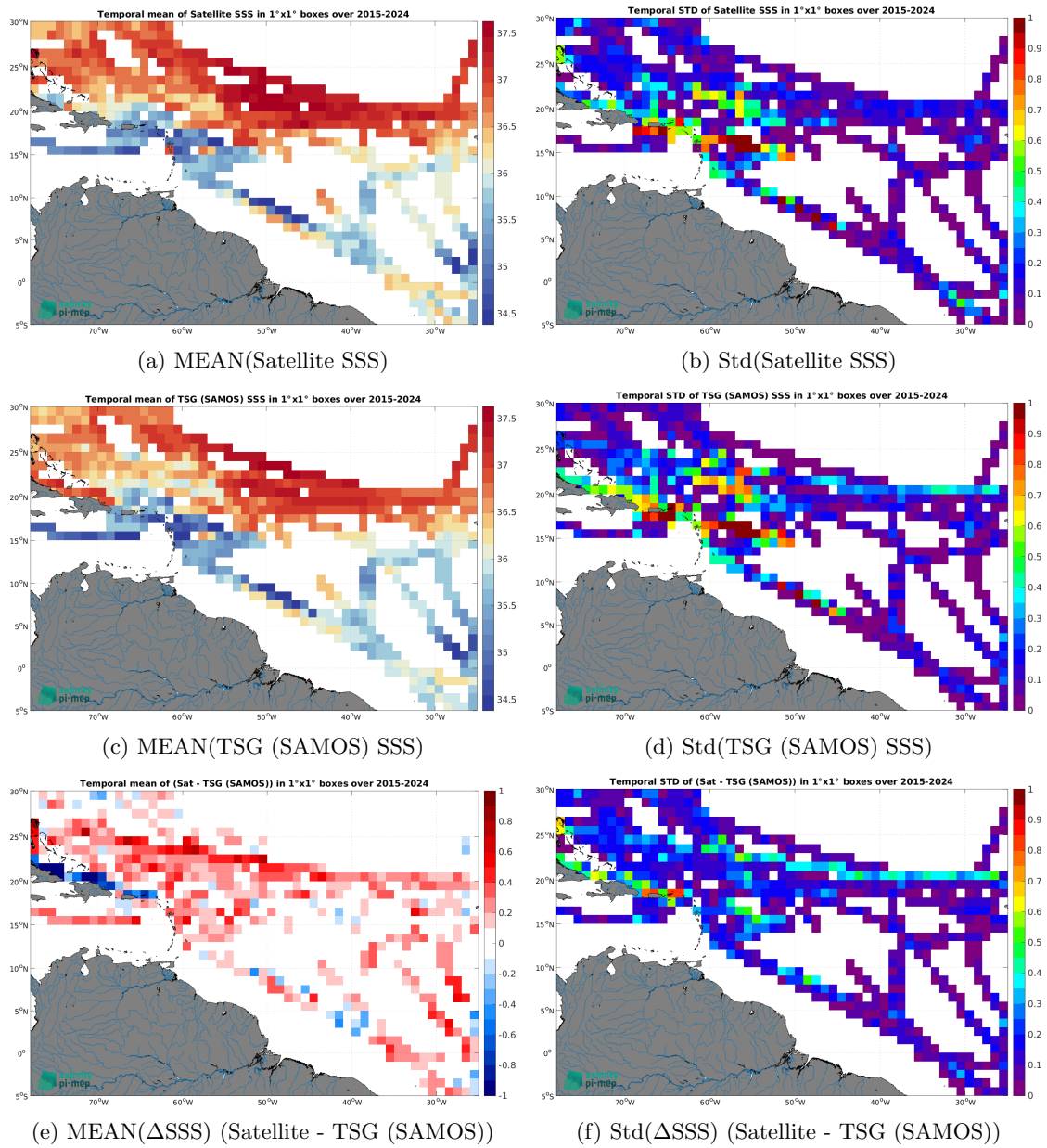
Figure 7: Temporal mean (left) and Std (right) of SSS from SMAP SSS L3 v5.0 - 8-Day running (JPL) (top), TSG (SAMOS) (middle), and of \Delta SSS (Satellite - TSG (SAMOS)). Only match-up pairs are used to generate these maps.
