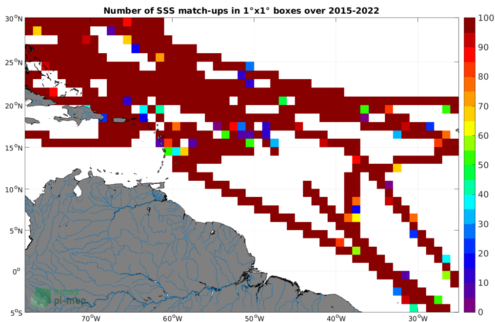
Figure 4: Number of SSS match-ups between TSG (SAMOS) SSS and the SMAP SSS L3 v5.0 - 8-Day running (JPL) SSS product for the Amazon and Orinoco river plumes Pi-MEP region over 1^\circ \times 1^\circ boxes and for the full satellite product period.
