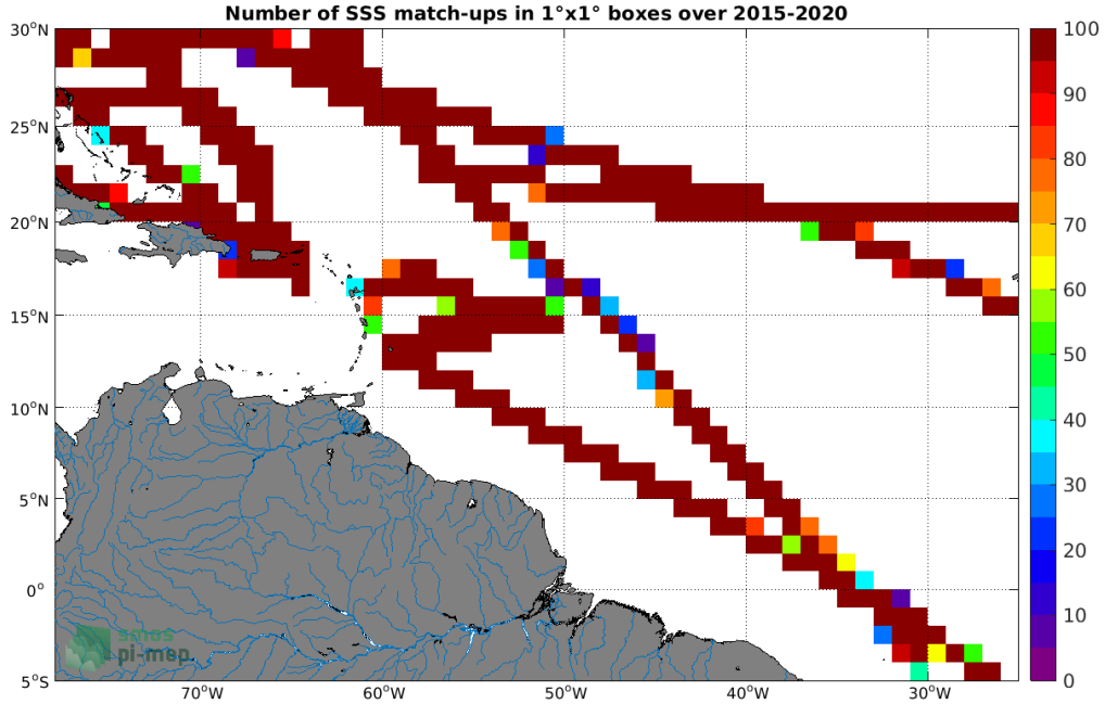
Figure 4: Number of SSS match-ups between TSG (SAMOS) SSS and the SMAP SSS L3 v5.0 - 8-Day running (JPL) SSS product for the Amazon and Orinoco river plumes Pi-MEP region over 1°x1° boxes and for the full satellite product period.
