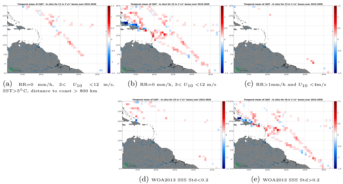
Figure 12: Temporal mean gridded over spatial boxes of size 1°x1° of \Delta SSS (SMAP SSS L3 v5.0 - 8-Day running (JPL) - TSG (SAMOS)) for 5 different subdatasets corresponding to: RR=0 mm/h, 3 < U_{10} < 12 m/s, SST > 5°C, distance to coast > 800 km (a), RR=0 mm/h, 3 < U_{10} < 12 m/s (b), RR > 1mm/h and U_{10} < 4 m/s (c), WOA2013 SSS Std < 0.2 (d), WOA2013 SSS Std > 0.2 (e).
