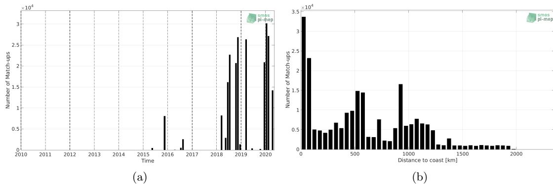
Figure 1: Number of match-ups between TSG (SAMOS) and SMAP SSS L3 v5.0 - 8-Day running (JPL) SSS as a function of time (a) and as function of the distance to coast (b) over the Amazon and Orinoco river plumes Pi-MEP region and for the full satellite product period.
