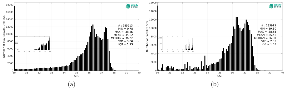
Figure 3: Histograms of SSS from TSG (LEGOS-DM) (a) and SMAP SSS L3 v5.0 - 8-Day running (JPL) (b) considering all match-up pairs per bins of 0.1 over the Amazon and Orinoco river plumes Pi-MEP region and for the full satellite product period.
