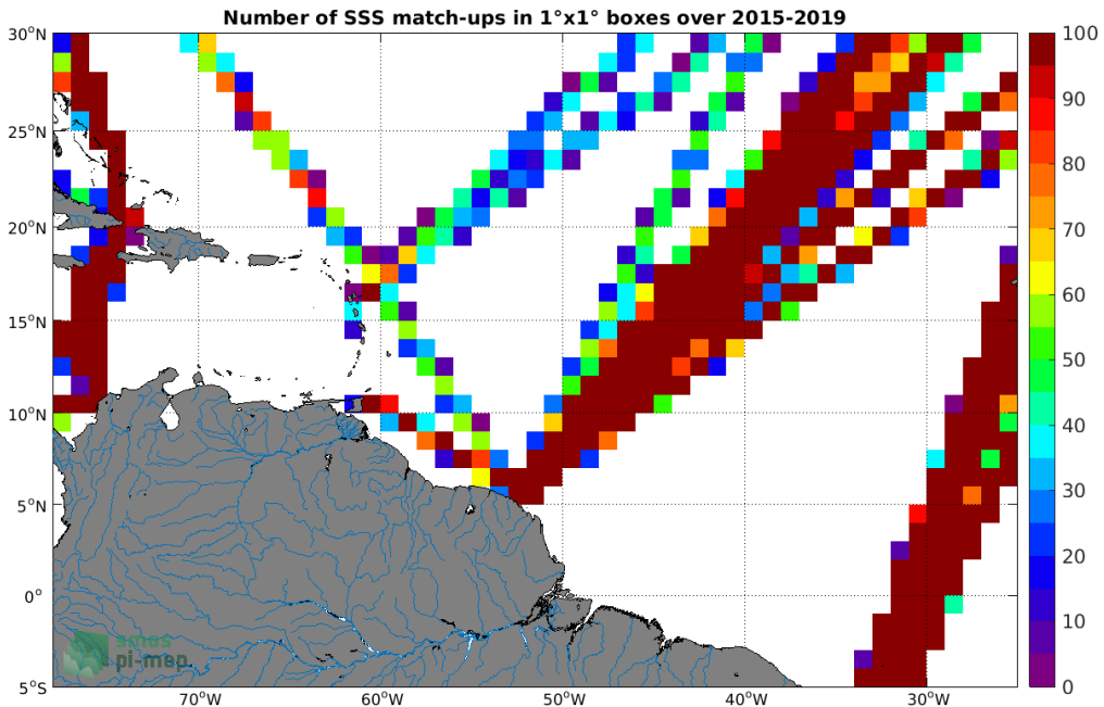
Figure 4: Number of SSS match-ups between TSG (LEGOS-DM) SSS and the SMAP SSS L3 v5.0 - 8-Day running (JPL) SSS product for the Amazon and Orinoco river plumes Pi-MEP region over 1°x1° boxes and for the full satellite product period.
