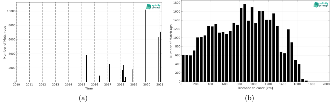
Figure 2: Number of match-ups between TSG (GOSUD-Sailing-ship) and SMAP SSS L3 v5.0 - 8-Day running (JPL) SSS as a function of time (a) and as function of the distance to coast (b) over the Amazon and Orinoco river plumes Pi-MEP region and for the full satellite product period.
