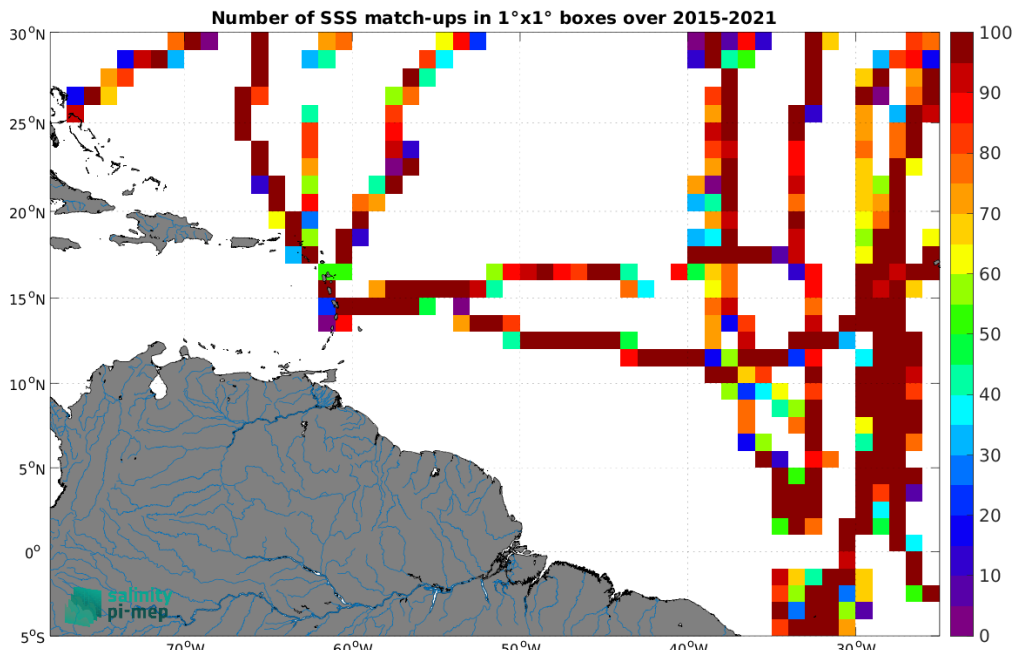
Figure 5: Number of SSS match-ups between TSG (GOSUD-Sailing-ship) SSS and the SMAP SSS L3 v5.0 - 8-Day running (JPL) SSS product for the Amazon and Orinoco river plumes Pi-MEP region over 1^\circ \times 1^\circ boxes and for the full satellite product period.
