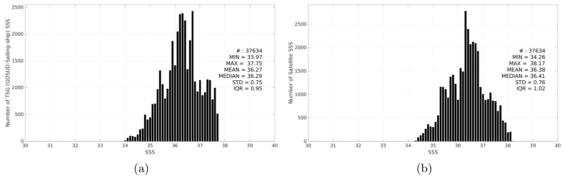
Figure 3: Histograms of SSS from TSG (GOSUD-Sailing-ship) (a) and SMAP SSS L3 v5.0 - 8-Day running (JPL) (b) considering all match-up pairs per bins of 0.1 over the Amazon and Orinoco river plumes Pi-MEP region and for the full satellite product period.
