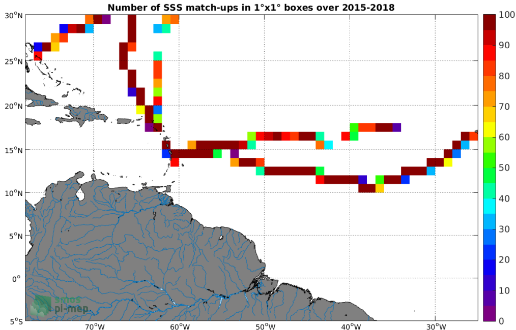
Figure 4: Number of SSS match-ups between TSG (GOSUD-Sailing-ship) SSS and the SMAP SSS L3 v5.0 - 8-Day running (JPL) SSS product for the Amazon and Orinoco river plumes Pi-MEP region over 1°x1° boxes and for the full satellite product period.
