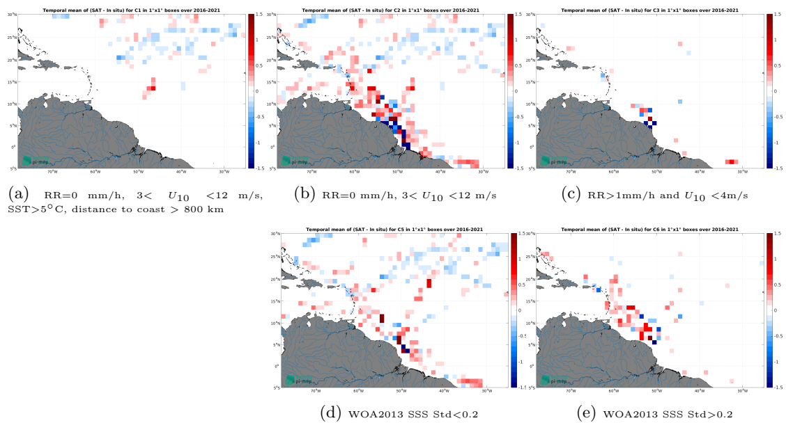
Figure 14: Temporal mean gridded over spatial boxes of size 1^\circ \times 1^\circ of \Delta SSS (SMAP SSS L3 v5.0 - 8-Day running (JPL) - TSG (GOSUD-Research-vessel)) for 5 different subdatasets corresponding to:RR=0 mm/h, 3 < U_{10} < 12 m/s, SST >5^\circ\text{C} , distance to coast > 800 km (a), RR=0 mm/h, 3 < U_{10} < 12 m/s (b), RR >1 mm/h and U_{10} < 4 m/s (c), WOA2013 SSS Std <0.2 (d), WOA2013 SSS Std >0.2 (e).
