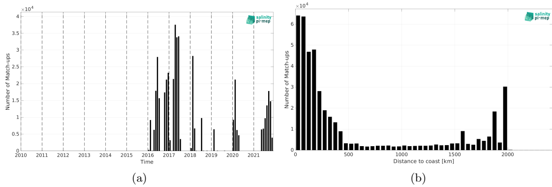
Figure 2: Number of match-ups between TSG (GOSUD-Research-vessel) and SMAP SSS L3 v5.0 - 8-Day running (JPL) SSS as a function of time (a) and as function of the distance to coast (b) over the Amazon and Orinoco river plumes Pi-MEP region and for the full satellite product period.
