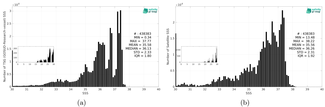
Figure 3: Histograms of SSS from TSG (GOSUD-Research-vessel) (a) and SMAP SSS L3 v5.0 - 8-Day running (JPL) (b) considering all match-up pairs per bins of 0.1 over the Amazon and Orinoco river plumes Pi-MEP region and for the full satellite product period.
