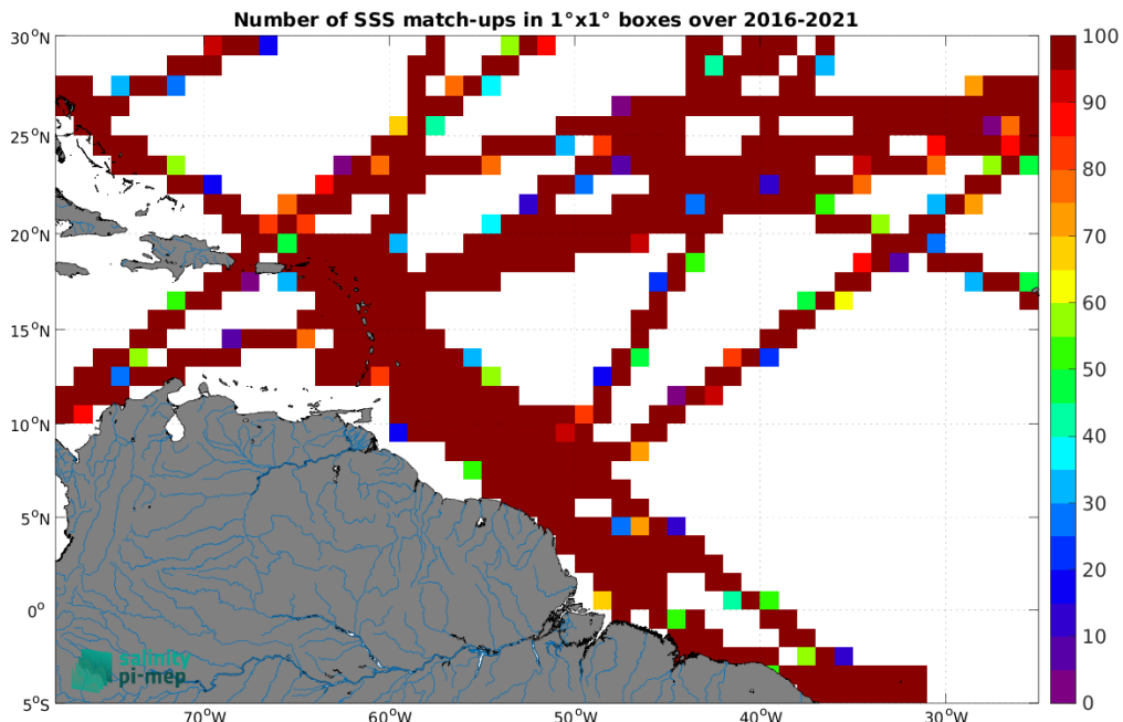
Figure 5: Number of SSS match-ups between TSG (GOSUD-Research-vessel) SSS and the SMAP SSS L3 v5.0 - 8-Day running (JPL) SSS product for the Amazon and Orinoco river plumes Pi-MEP region over 1^\circ \times 1^\circ boxes and for the full satellite product period.
