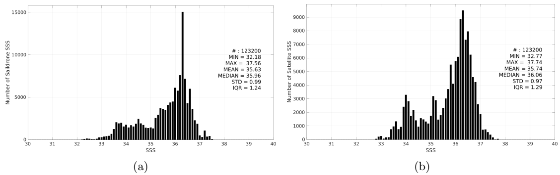
Figure 3: Histograms of SSS from Sairdron (a) and SMAP SSS L3 v5.0 - 8-Day running (JPL) (b) considering all match-up pairs per bins of 0.1 over the Amazon and Orinoco river plumes Pi-MEP region and for the full satellite product period.
