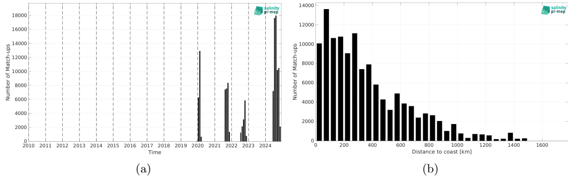
Figure 2: Number of match-ups between Sairdron and SMAP SSS L3 v5.0 - 8-Day running (JPL) SSS as a function of time (a) and as function of the distance to coast (b) over the Amazon and Orinoco river plumes Pi-MEP region and for the full satellite product period.
