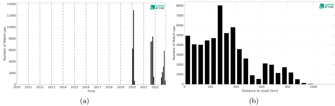
Figure 2: Number of match-ups between Saildrone and SMAP SSS L3 v5.0 - 8-Day running (JPL) SSS as a function of time (a) and as function of the distance to coast (b) over the Amazon and Orinoco river plumes Pi-MEP region and for the full satellite product period.
