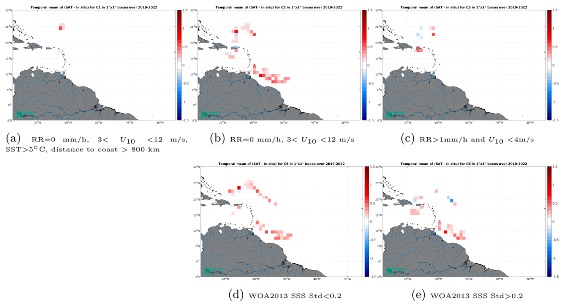
Figure 14: Temporal mean gridded over spatial boxes of size 1^\circ \times 1^\circ of \Delta SSS (SMAP SSS L3 v5.0 - 8-Day running (JPL) - Saildrone) for 5 different subdatasets corresponding to:RR=0 mm/h, 3 < U_{10} < 12 m/s, SST >5^\circ\text{C} , distance to coast > 800 km (a), RR=0 mm/h, 3 < U_{10} < 12 m/s (b), RR >1 mm/h and U_{10} < 4 m/s (c), WOA2013 SSS Std <0.2 (d), WOA2013 SSS Std >0.2 (e).
