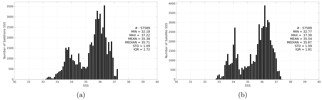
Figure 3: Histograms of SSS from Saildrone (a) and SMAP SSS L3 v5.0 - 8-Day running (JPL) (b) considering all match-up pairs per bins of 0.1 over the Amazon and Orinoco river plumes Pi-MEP region and for the full satellite product period.
