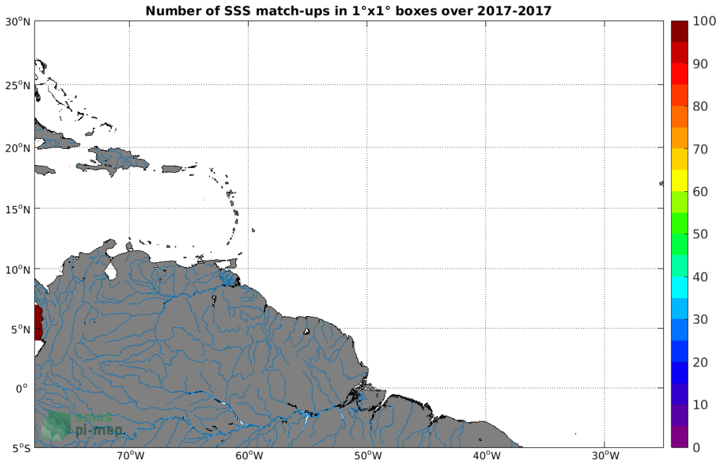
Figure 3: Number of SSS match-ups between Surface drifters SSS and the SMAP SSS L3 v5.0 - 8-Day running (JPL) SSS product for the Amazon and Orinoco river plumes Pi-MEP region over 1^{\circ} \times 1^{\circ} boxes and for the full satellite product period.
