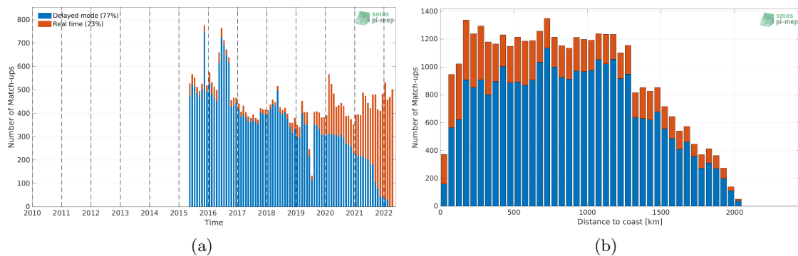
Figure 1: Number of match-ups between Argo and SMAP SSS L3 v5.0 - 8-Day running (JPL) SSS as a function of time (a) and as function of the distance to coast (b) over the Amazon and Orinoco river plumes Pi-MEP region and for the full satellite product period.
