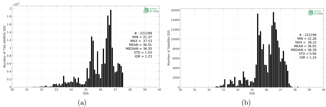
Figure 2: Histograms of SSS from TSG-SAMOS (a) and SMAP-L3-JPL-V4.3-8DAY-RUNNING-60KM (b) considering all match-up pairs per bins of 0.1 over the Amazon and Orinoco river plumes Pi-MEP region and for the full satellite product period.
