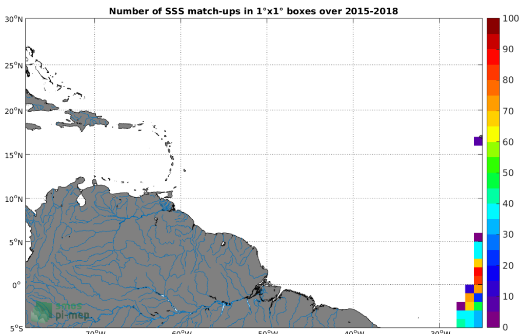
Figure 4: Number of SSS match-ups between TSG-POLARSTERN SSS and the SMAP-L3-JPL-V4.3-8DAY-RUNNING-60KM SSS product for the Amazon and Orinoco river plumes Pi-MEP region over 1°x1° boxes and for the full satellite product period.
