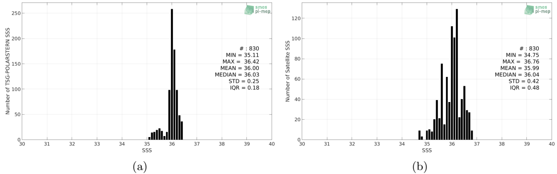
Figure 2: Histograms of SSS from TSG-POLARSTERN (a) and SMAP-L3-JPL-V4.3-8DAY-RUNNING-60KM (b) considering all match-up pairs per bins of 0.1 over the Amazon and Orinoco river plumes Pi-MEP region and for the full satellite product period.
