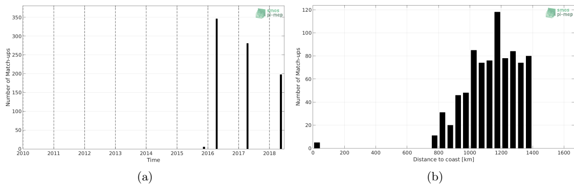
Figure 1: Number of match-ups between TSG-POLARSTERN and SMAP-L3-JPL-V4.3-8DAY-RUNNING-60KM SSS as a function of time (a) and as function of the distance to coast (b) over the Amazon and Orinoco river plumes Pi-MEP region and for the full satellite product period.
