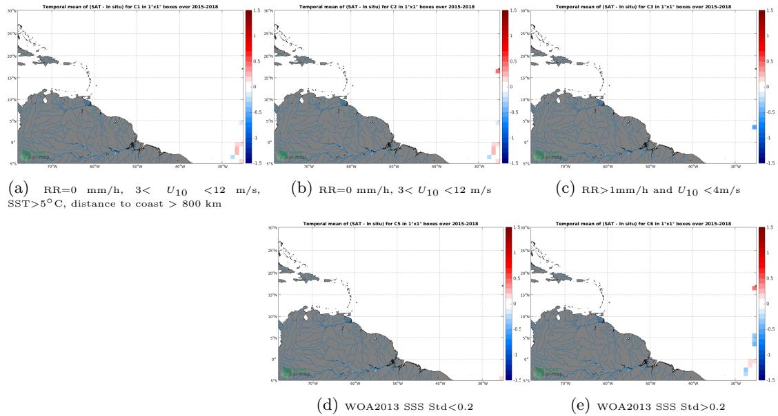
Figure 12: Temporal mean gridded over spatial boxes of size 1^\circ \times 1^\circ of \Delta SSS (SMAP-L3-JPL-V4.3-8DAY-RUNNING-60KM - TSG-POLARSTERN) for 5 different subdatasets corresponding to:RR=0 mm/h, 3 < U_{10} < 12 m/s, SST >5^\circ C, distance to coast > 800 km (a), RR=0 mm/h, 3 < U_{10} < 12 m/s (b), RR >1 mm/h and U_{10} < 4 m/s (c), WOA2013 SSS Std <0.2 (d), WOA2013 SSS Std >0.2 (e).
