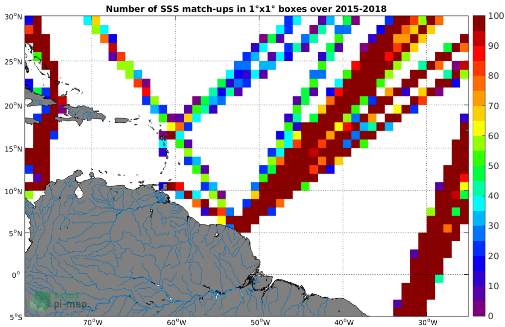
Figure 4: Number of SSS match-ups between TSG-LEGOS-DM SSS and the SMAP-L3-JPL-V4.3-8DAY-RUNNING-60KM SSS product for the Amazon and Orinoco river plumes Pi-MEP region over 1°x1° boxes and for the full satellite product period.
