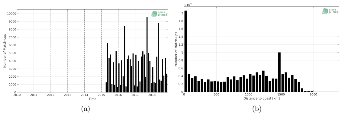
Figure 1: Number of match-ups between TSG-LEGOS-DM and SMAP-L3-JPL-V4.3-8DAY-RUNNING-60KM SSS as a function of time (a) and as function of the distance to coast (b) over the Amazon and Orinoco river plumes Pi-MEP region and for the full satellite product period.
