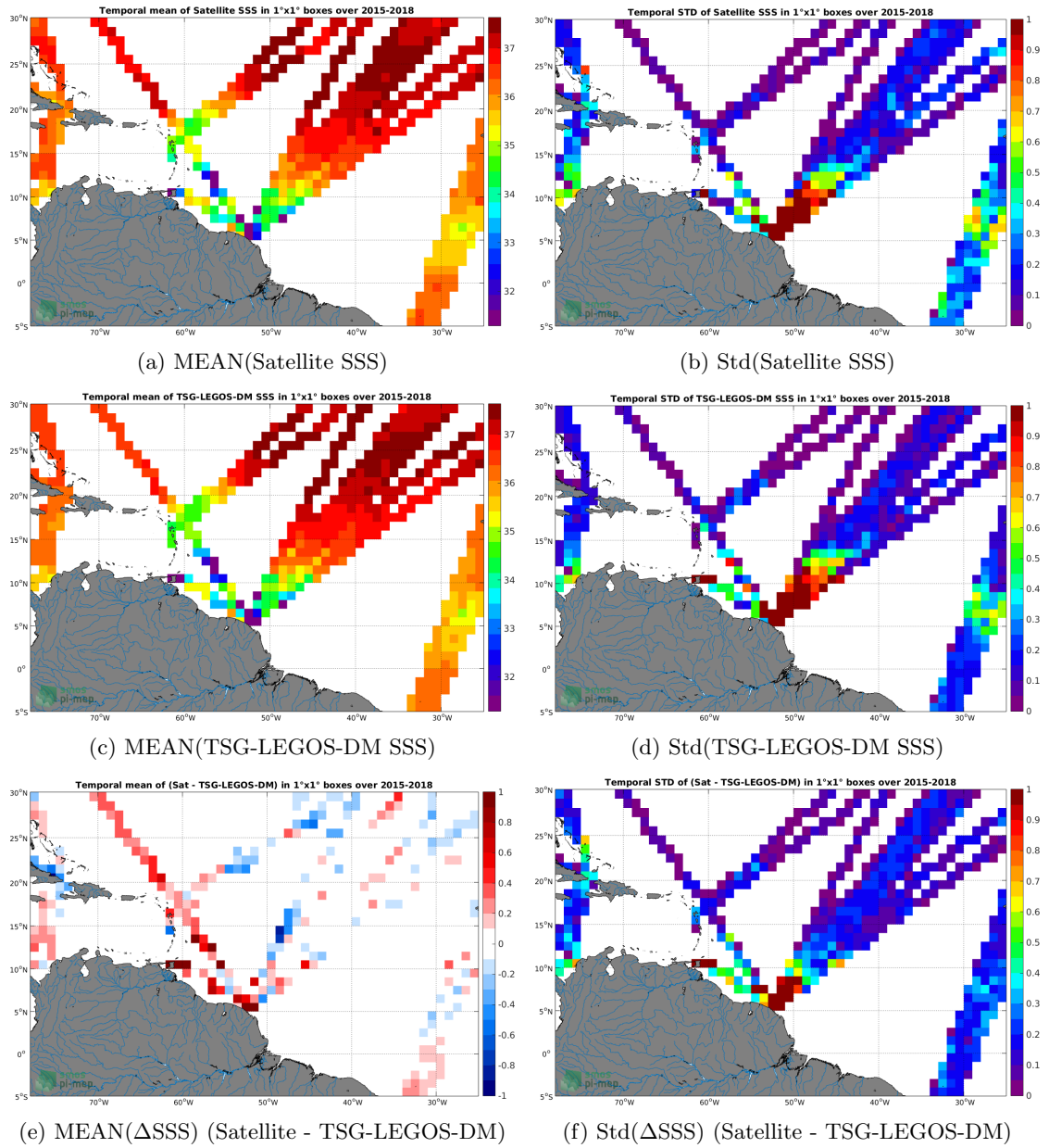
Figure 6: Temporal mean (left) and Std (right) of SSS from SMAP-L3-JPL-V4.3-8DAY-RUNNING-60KM (top), TSG-LEGOS-DM (middle), and of \Delta SSS (Satellite - TSG-LEGOS-DM). Only match-up pairs are used to generate these maps.
