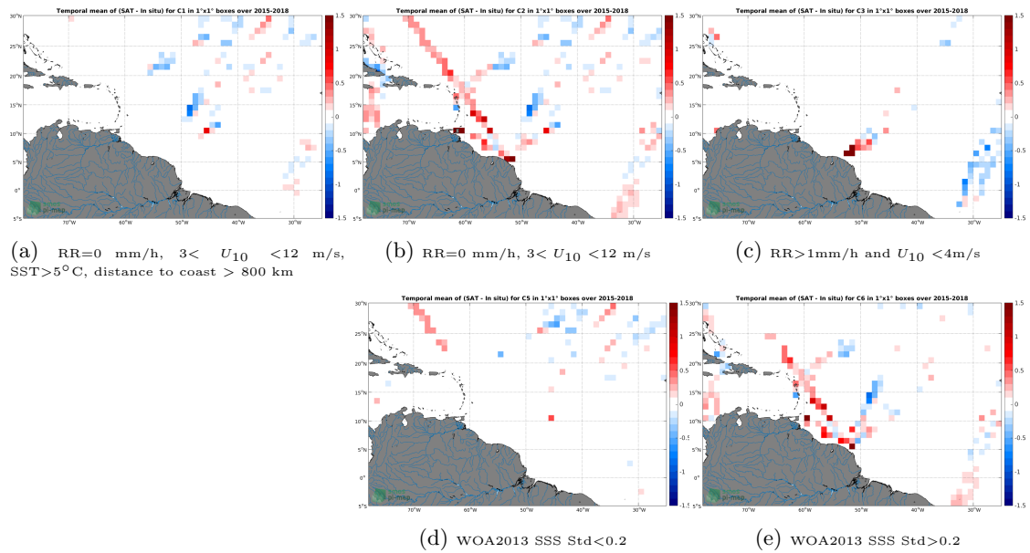
Figure 12: Temporal mean gridded over spatial boxes of size 1^\circ \times 1^\circ of \Delta SSS (SMAP-L3-JPL-V4.3-8DAY-RUNNING-60KM - TSG-LEGOS-DM) for 5 different subdatasets corresponding to:RR=0 mm/h, 3 < U_{10} < 12 m/s, SST > 5^\circ\text{C} , distance to coast > 800 km (a), RR=0 mm/h, 3 < U_{10} < 12 m/s (b), RR > 1 mm/h and U_{10} < 4 m/s (c), WOA2013 SSS Std < 0.2 (d), WOA2013 SSS Std > 0.2 (e).
