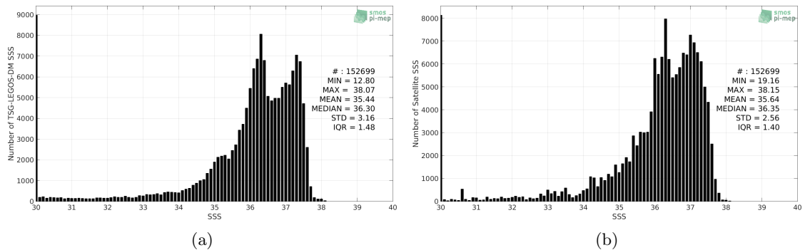
Figure 2: Histograms of SSS from TSG-LEGOS-DM (a) and SMAP-L3-JPL-V4.3-8DAY-RUNNING-60KM (b) considering all match-up pairs per bins of 0.1 over the Amazon and Orinoco river plumes Pi-MEP region and for the full satellite product period.
