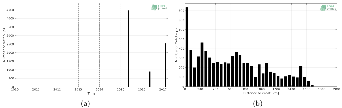
Figure 1: Number of match-ups between TSG-GOSUD-Sailing-ship and SMAP-L3-JPL-V4.3-8DAY-RUNNING-60KM SSS as a function of time (a) and as function of the distance to coast (b) over the Amazon and Orinoco river plumes Pi-MEP region and for the full satellite product period.
