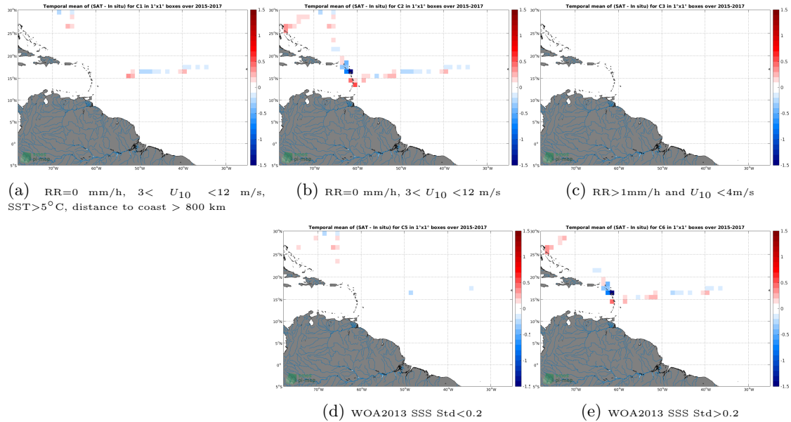
Figure 12: Temporal mean gridded over spatial boxes of size 1^{\circ}\times 1^{\circ} of \Delta SSS (SMAP-L3-JPL-V4.3-8DAY-RUNNING-60KM - TSG-GOSUD-Sailing-ship) for 5 different subdatasets corresponding to:RR=0 mm/h, 3 < U_{10} < 12 m/s, SST >5^{\circ}\text{C} , distance to coast > 800 km (a), RR=0 mm/h, 3 < U_{10} < 12 m/s (b), RR >1 mm/h and U_{10} < 4 m/s (c), WOA2013 SSS Std <0.2 (d), WOA2013 SSS Std >0.2 (e).
