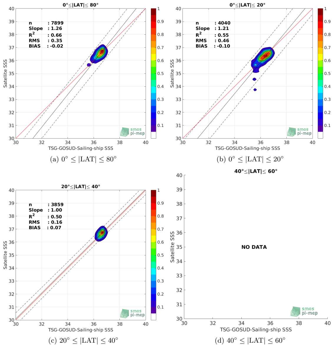
Figure 9: Contour maps of the concentration of SMAP-L3-JPL-V4.3-8DAY-RUNNING-60KM SSS (y-axis) versus TSG-GOSUD-Sailing-ship SSS (x-axis) at match-up pairs for different latitude bands. For each plot, the red line shows x=y . The black thin and dashed lines indicate a linear fit through the data cloud and the \pm 95\% confidence levels, respectively. The number match-up pairs n , the slope and R^2 coefficient of the linear fit, the root mean square (RMS) and the mean bias between satellite and in situ data are indicated for each latitude band in each plots.
