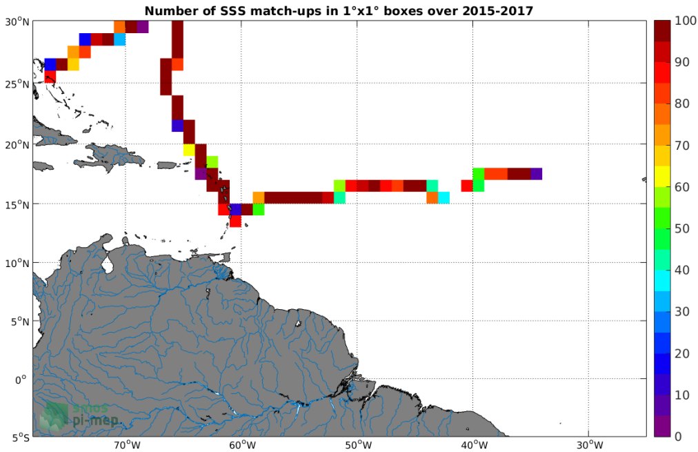
Figure 4: Number of SSS match-ups between TSG-GOSUD-Sailing-ship SSS and the SMAP-L3-JPL-V4.3-8DAY-RUNNING-60KM SSS product for the Amazon and Orinoco river plumes Pi-MEP region over 1°x1° boxes and for the full satellite product period.
