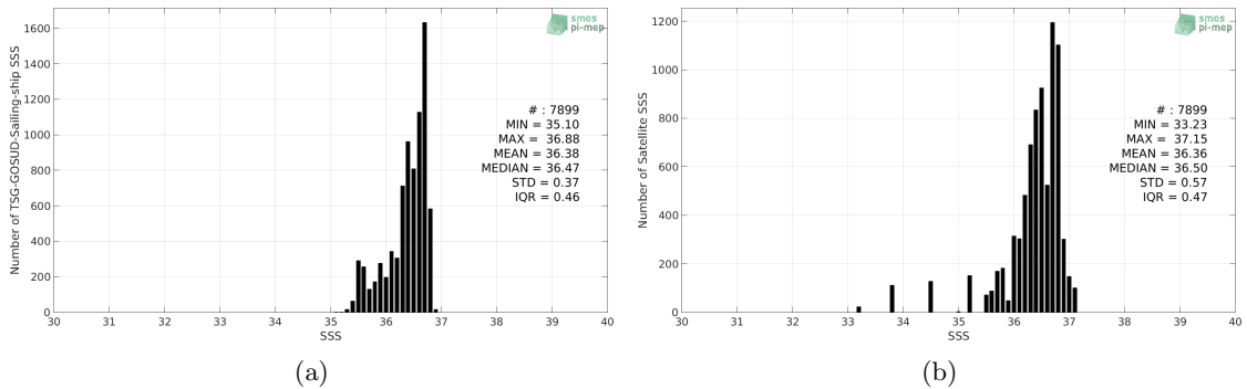
Figure 2: Histograms of SSS from TSG-GOSUD-Sailing-ship (a) and SMAP-L3-JPL-V4.3-8DAY-RUNNING-60KM (b) considering all match-up pairs per bins of 0.1 over the Amazon and Orinoco river plumes Pi-MEP region and for the full satellite product period.
