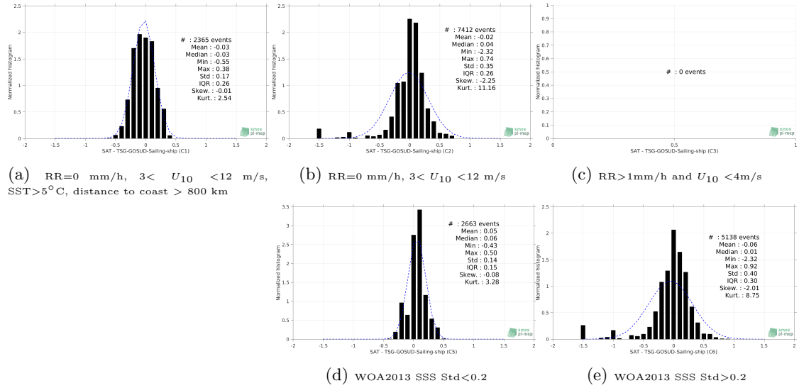
Figure 13: Normalized histogram of \Delta SSS (SMAP-L3-JPL-V4.3-8DAY-RUNNING-60KM - TSG-GOSUD-Sailing-ship) for 5 different subdatasets corresponding to: RR=0 mm/h, 3 < U_{10} < 12 m/s, SST > 5°C, distance to coast > 800 km (a), RR=0 mm/h, 3 < U_{10} < 12 m/s (b), RR > 1mm/h and U_{10} < 4 m/s (c), WOA2013 SSS Std < 0.2 (d), WOA2013 SSS Std > 0.2 (e).
