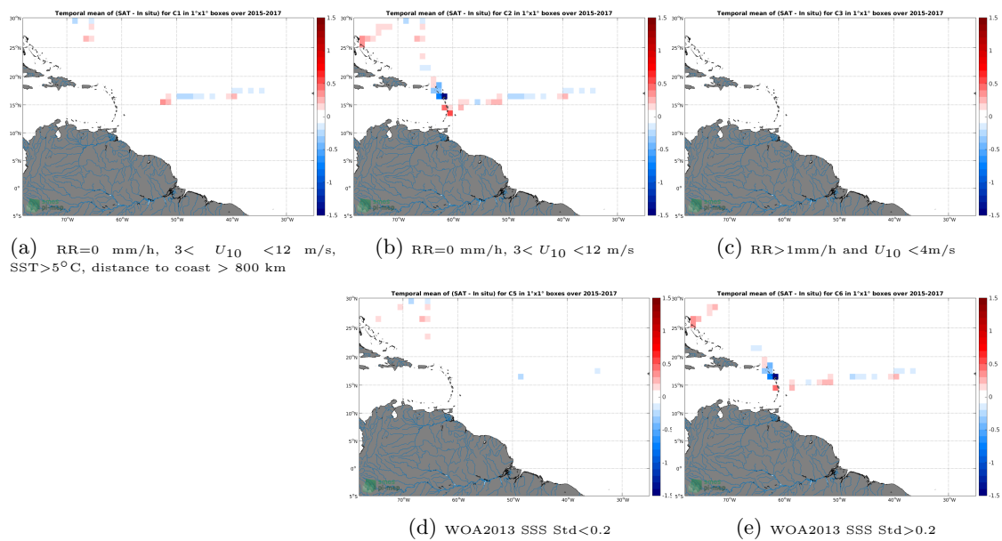
Figure 12: Temporal mean gridded over spatial boxes of size 1^\circ \times 1^\circ of \Delta SSS (SMAP-L3-JPL-V4.3-8DAY-RUNNING-60KM - TSG-GOSUD-Sailing-ship) for 5 different subdatasets corresponding to:RR=0 mm/h, 3 < U_{10} < 12 m/s, SST >5^\circ\text{C} , distance to coast > 800 km (a), RR=0 mm/h, 3 < U_{10} < 12 m/s (b), RR >1 mm/h and U_{10} < 4 m/s (c), WOA2013 SSS Std <0.2 (d), WOA2013 SSS Std >0.2 (e).
