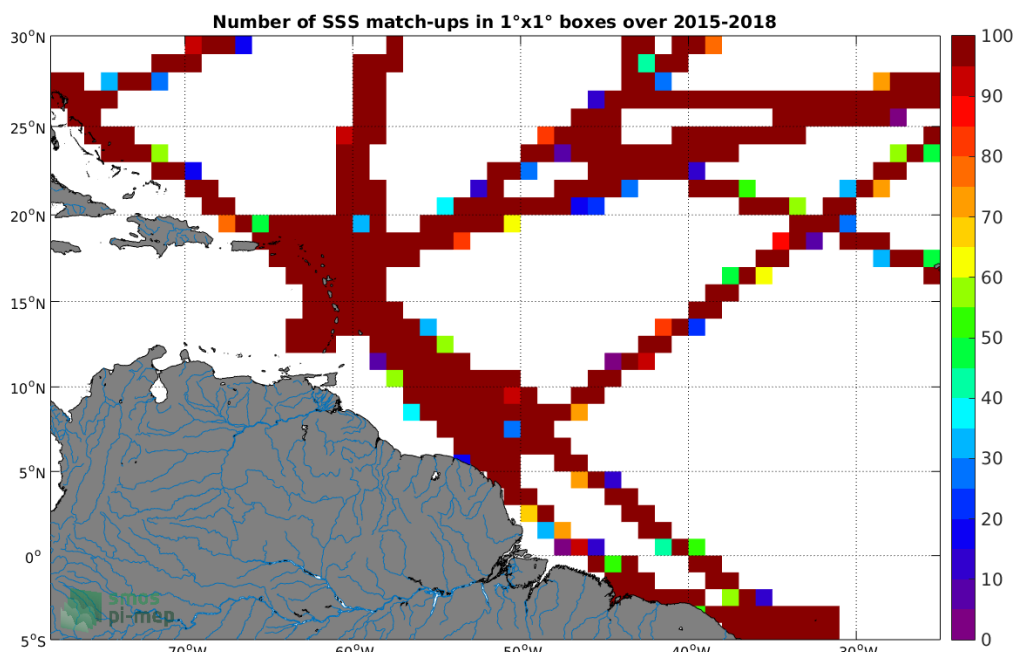
Figure 4: Number of SSS match-ups between TSG-GOSUD-Research-vessel SSS and the SMAP-L3-JPL-V4.3-8DAY-RUNNING-60KM SSS product for the Amazon and Orinoco river plumes Pi-MEP region over 1^\circ \times 1^\circ boxes and for the full satellite product period.
