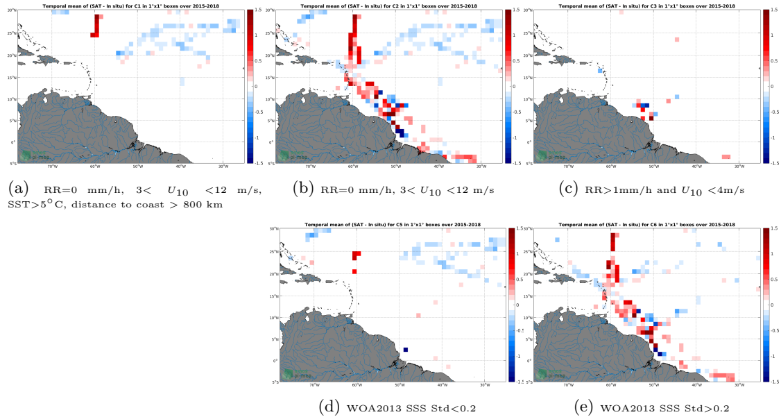
Figure 12: Temporal mean gridded over spatial boxes of size 1^{\circ}\times 1^{\circ} of \Delta SSS (SMAP-L3-JPL-V4.3-8DAY-RUNNING-60KM - TSG-GOSUD-Research-vessel) for 5 different subdatasets corresponding to:RR=0 mm/h, 3 < U_{10} < 12 m/s, SST >5^{\circ}\text{C} , distance to coast > 800 km (a), RR=0 mm/h, 3 < U_{10} < 12 m/s (b), RR >1 mm/h and U_{10} < 4 m/s (c), WOA2013 SSS Std <0.2 (d), WOA2013 SSS Std >0.2 (e).
