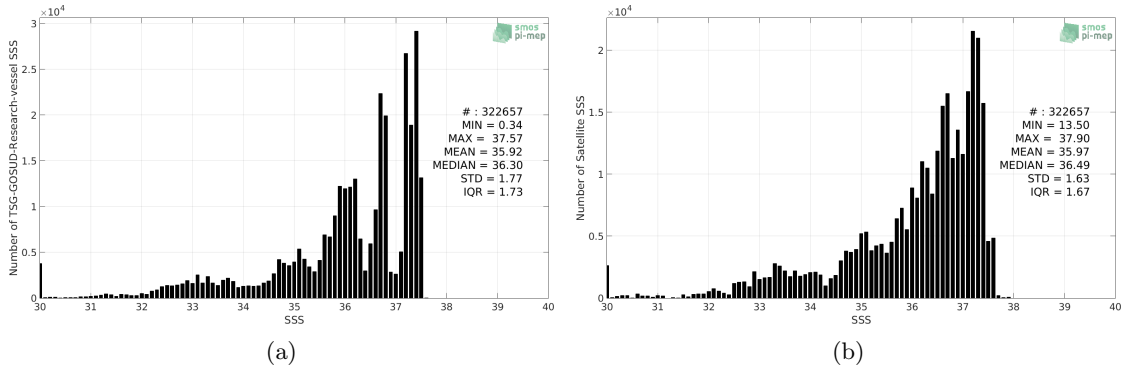
Figure 2: Histograms of SSS from TSG-GOSUD-Research-vessel (a) and SMAP-L3-JPL-V4.3-8DAY-RUNNING-60KM (b) considering all match-up pairs per bins of 0.1 over the Amazon and Orinoco river plumes Pi-MEP region and for the full satellite product period.
