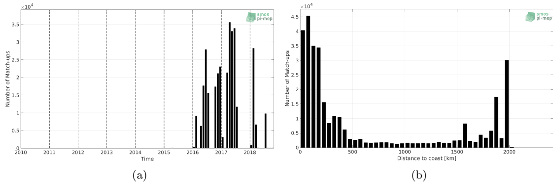
Figure 1: Number of match-ups between TSG-GOSUD-Research-vessel and SMAP-L3-JPL-V4.3-8DAY-RUNNING-60KM SSS as a function of time (a) and as function of the distance to coast (b) over the Amazon and Orinoco river plumes Pi-MEP region and for the full satellite product period.
