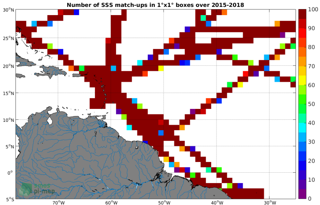
Figure 4: Number of SSS match-ups between TSG-GOSUD-Research-vessel SSS and the SMAP-L3-JPL-V4.3-8DAY-RUNNING-60KM SSS product for the Amazon and Orinoco river plumes Pi-MEP region over 1^{\circ} \times 1^{\circ} boxes and for the full satellite product period.
