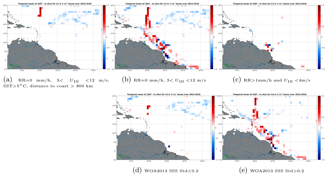
Figure 12: Temporal mean gridded over spatial boxes of size 1^\circ \times 1^\circ of \Delta SSS (SMAP-L3-JPL-V4.3-8DAY-RUNNING-60KM - TSG-GOSUD-Research-vessel) for 5 different subdatasets corresponding to: RR=0 mm/h, 3 < U_{10} < 12 m/s, SST > 5°C, distance to coast > 800 km (a), RR=0 mm/h, 3 < U_{10} < 12 m/s (b), RR > 1mm/h and U_{10} < 4 m/s (c), WOA2013 SSS Std < 0.2 (d), WOA2013 SSS Std > 0.2 (e).
