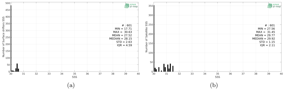
Figure 2: Histograms of SSS from Surface drifters (a) and SMAP-L3-JPL-V4.3-8DAY-RUNNING-60KM (b) considering all match-up pairs per bins of 0.1 over the Amazon and Orinoco river plumes Pi-MEP region and for the full satellite product period.
