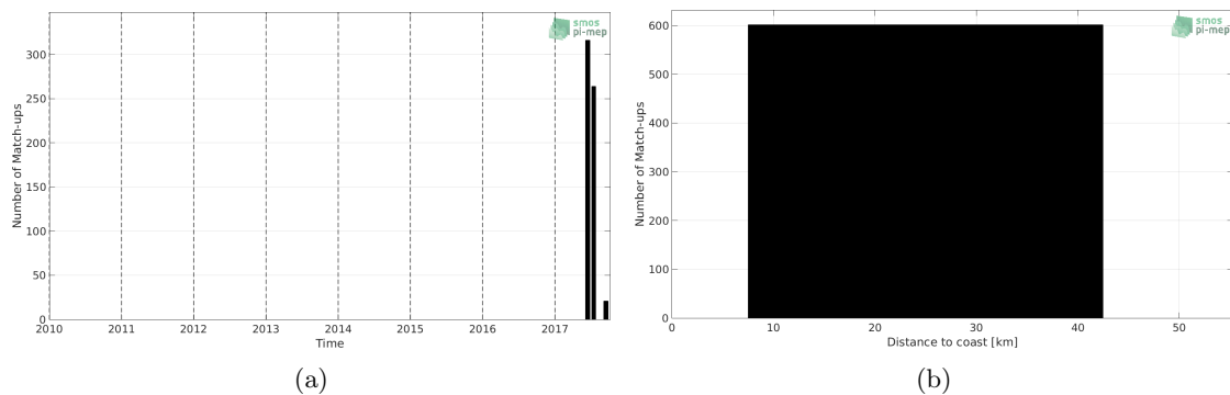
Figure 1: Number of match-ups between Surface drifters and SMAP-L3-JPL-V4.3-8DAY-RUNNING-60KM SSS as a function of time (a) and as function of the distance to coast (b) over the Amazon and Orinoco river plumes Pi-MEP region and for the full satellite product period.
