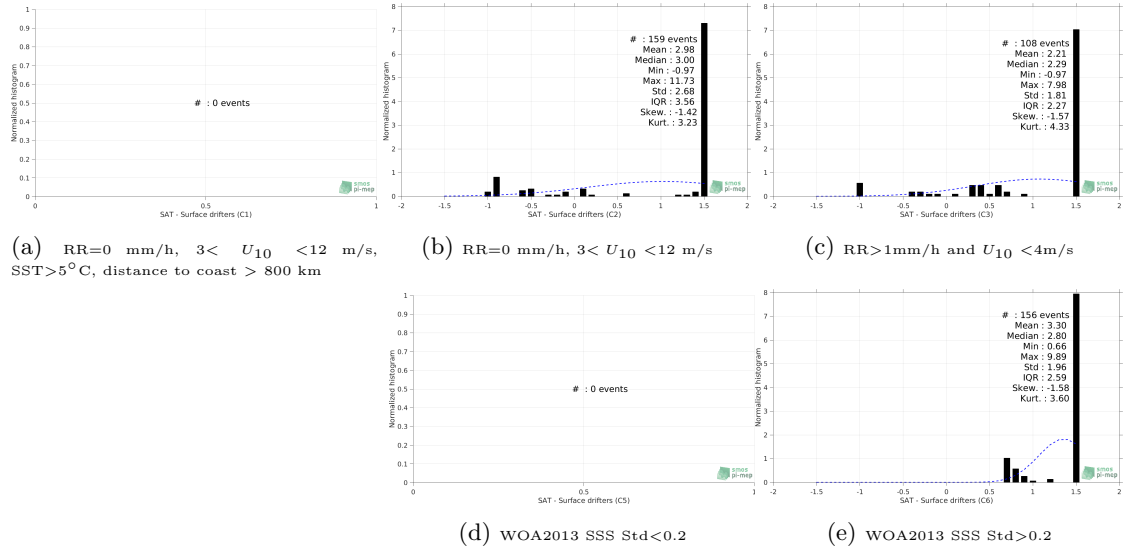
Figure 12: Normalized histogram of \Delta SSS (SMAP-L3-JPL-V4.3-8DAY-RUNNING-60KM - Surface drifters) for 5 different subdatasets corresponding to: RR=0 mm/h, 3 < U_{10} < 12 m/s, SST>5°C, distance to coast > 800 km (a), RR=0 mm/h, 3 < U_{10} < 12 m/s (b), RR>1mm/h and U_{10} < 4 m/s (c), WOA2013 SSS Std<0.2 (d), WOA2013 SSS Std>0.2 (e).
