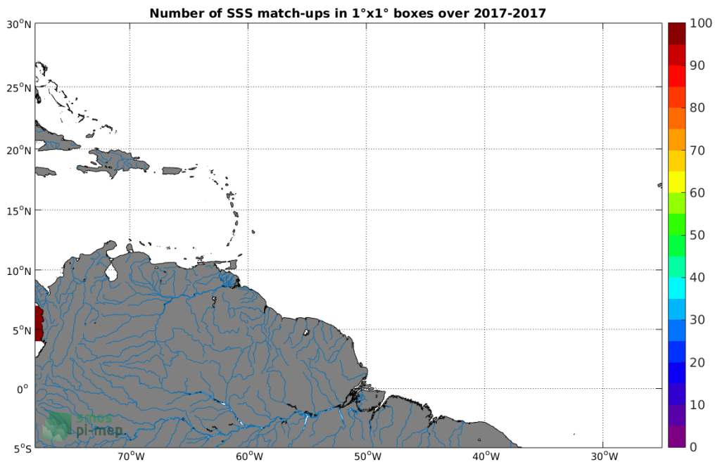
Figure 3: Number of SSS match-ups between Surface drifters SSS and the SMAP-L3-JPL-V4.3-8DAY-RUNNING-60KM SSS product for the Amazon and Orinoco river plumes Pi-MEP region over 1°x1° boxes and for the full satellite product period.
