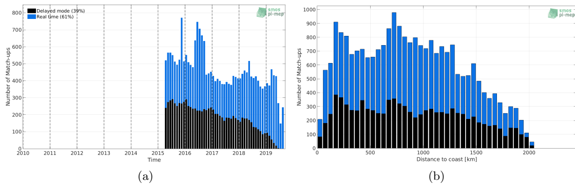
Figure 1: Number of match-ups between Argo and SMAP-L3-JPL-V4.3-8DAY-RUNNING-60KM SSS as a function of time (a) and as function of the distance to coast (b) over the Amazon and Orinoco river plumes Pi-MEP region and for the full satellite product period.
