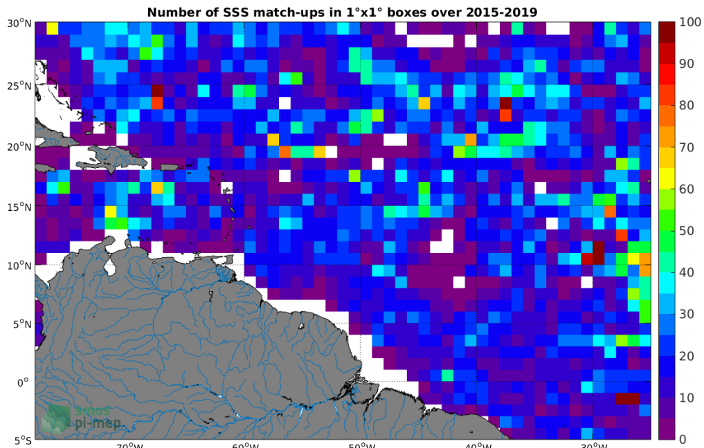
Figure 4: Number of SSS match-ups between Argo SSS and the SMAP-L3-JPL-V4.3-8DAY-RUNNING-60KM SSS product for the Amazon and Orinoco river plumes Pi-MEP region over 1°x1° boxes and for the full satellite product period.
