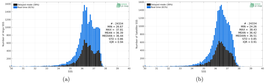
Figure 2: Histograms of SSS from Argo (a) and SMAP-L3-JPL-V4.3-8DAY-RUNNING-60KM (b) considering all match-up pairs per bins of 0.1 over the Amazon and Orinoco river plumes Pi-MEP region and for the full satellite product period.
