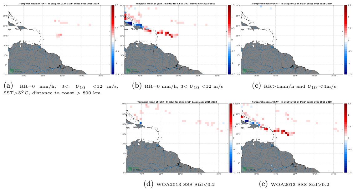
Figure 12: Temporal mean gridded over spatial boxes of size 1^\circ \times 1^\circ of \Delta SSS (SMAP-L3-JPL-V4.2-MONTHLY-60KM - TSG-SAMOS) for 5 different subdatasets corresponding to:RR=0 mm/h, 3 < U_{10} < 12 m/s, SST >5^\circ\text{C} , distance to coast > 800 km (a), RR=0 mm/h, 3 < U_{10} < 12 m/s (b), RR >1 mm/h and U_{10} < 4 m/s (c), WOA2013 SSS Std <0.2 (d), WOA2013 SSS Std >0.2 (e).
