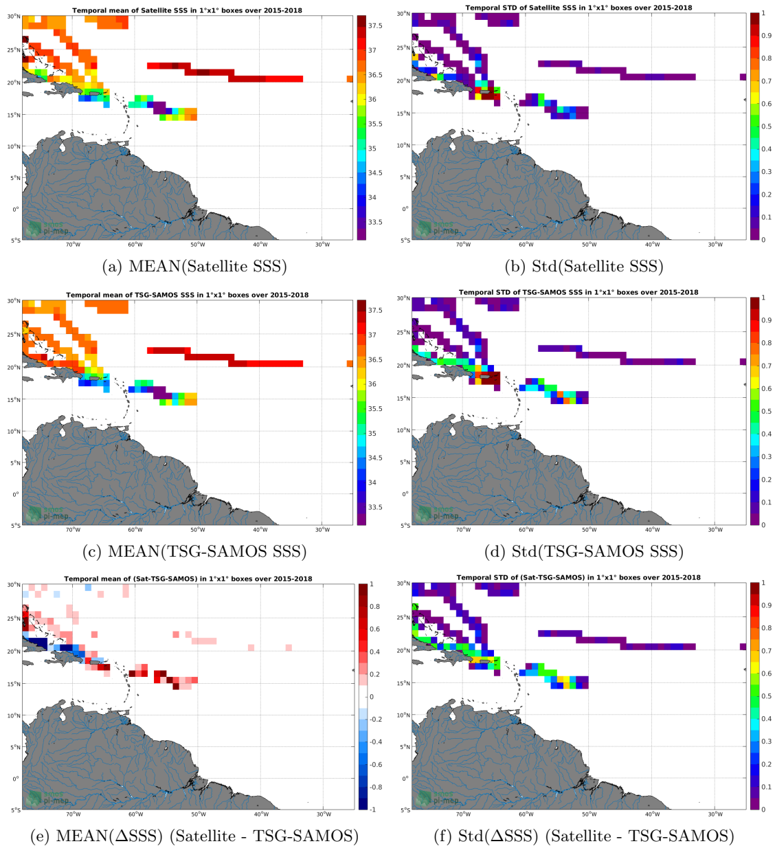
Figure 6: Temporal mean (left) and Std (right) of SSS from SMAP-L3-JPL-V4.2-MONTHLY-60KM (top), TSG-SAMOS (middle), and of \Delta SSS (Satellite - TSG-SAMOS). Only match-up pairs are used to generate these maps.
