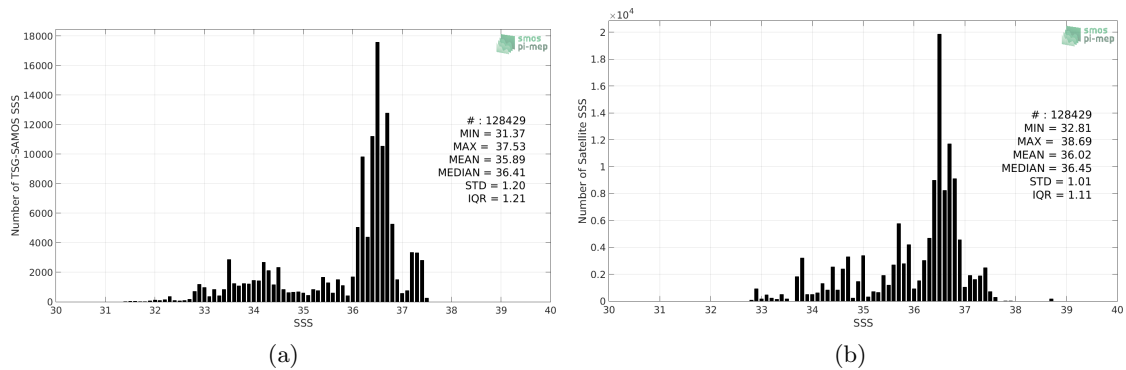
Figure 2: Histograms of SSS from TSG-SAMOS (a) and SMAP-L3-JPL-V4.2-MONTHLY-60KM (b) considering all match-up pairs per bins of 0.1 over the Amazon and Orinoco river plumes Pi-MEP region and for the full satellite product period.
