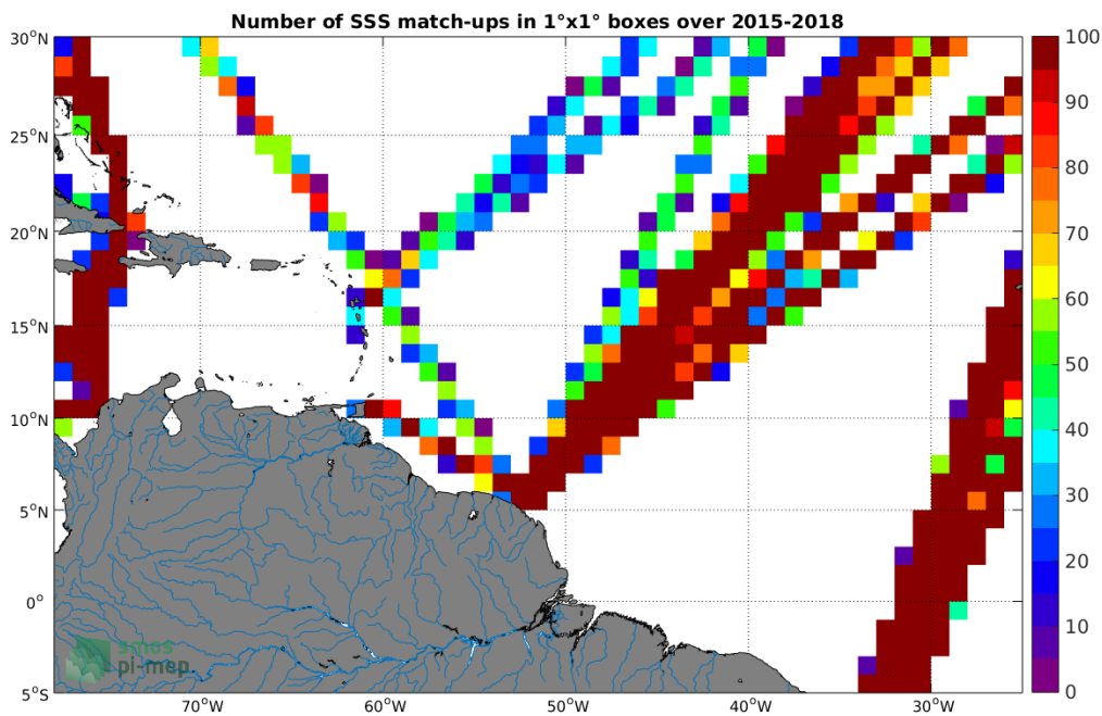
Figure 4: Number of SSS match-ups between TSG-LEGOS-DM SSS and the SMAP-L3-JPL-V4.2-MONTHLY-60KM SSS product for the Amazon and Orinoco river plumes Pi-MEP region over 1^\circ \times 1^\circ boxes and for the full satellite product period.
