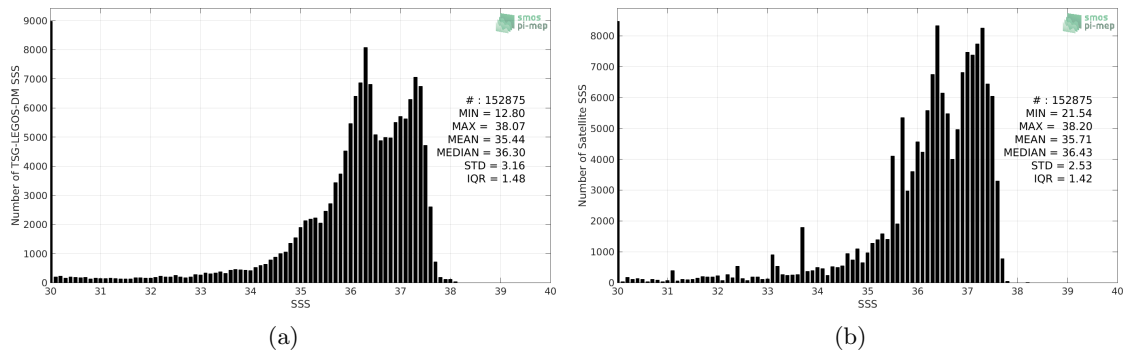
Figure 2: Histograms of SSS from TSG-LEGOS-DM (a) and SMAP-L3-JPL-V4.2-MONTHLY-60KM (b) considering all match-up pairs per bins of 0.1 over the Amazon and Orinoco river plumes Pi-MEP region and for the full satellite product period.
