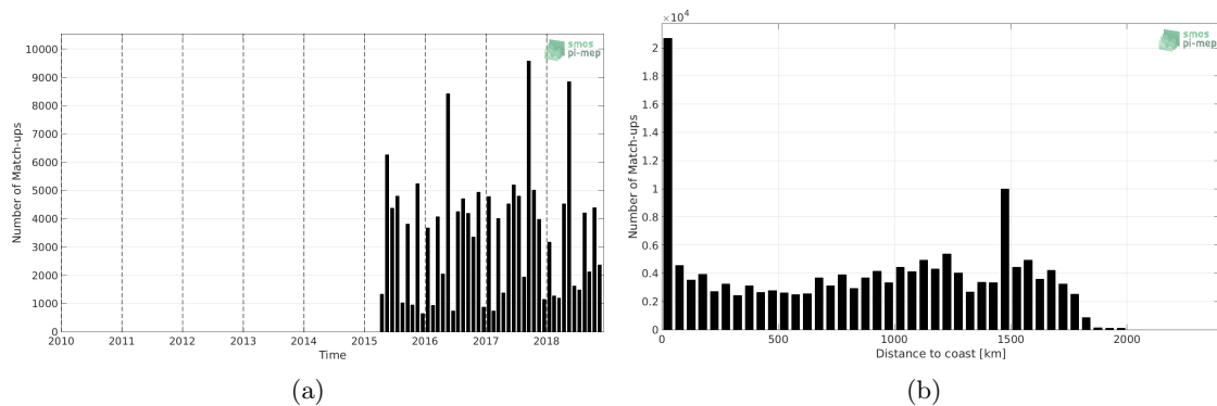
Figure 1: Number of match-ups between TSG-LEGOS-DM and SMAP-L3-JPL-V4.2-MONTHLY-60KM SSS as a function of time (a) and as function of the distance to coast (b) over the Amazon and Orinoco river plumes Pi-MEP region and for the full satellite product period.
