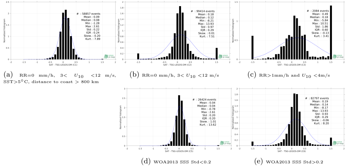
Figure 13: Normalized histogram of \Delta\text{SSS} (SMAP-L3-JPL-V4.2-MONTHLY-60KM - TSG-LEGOS-DM) for 5 different subdatasets corresponding to: RR=0 mm/h, 3 < U_{10} < 12 m/s, SST > 5^\circ\text{C} , distance to coast > 800 km (a), RR=0 mm/h, 3 < U_{10} < 12 m/s (b), RR > 1 mm/h and U_{10} < 4 m/s (c), WOA2013 SSS Std < 0.2 (d), WOA2013 SSS Std > 0.2 (e).
