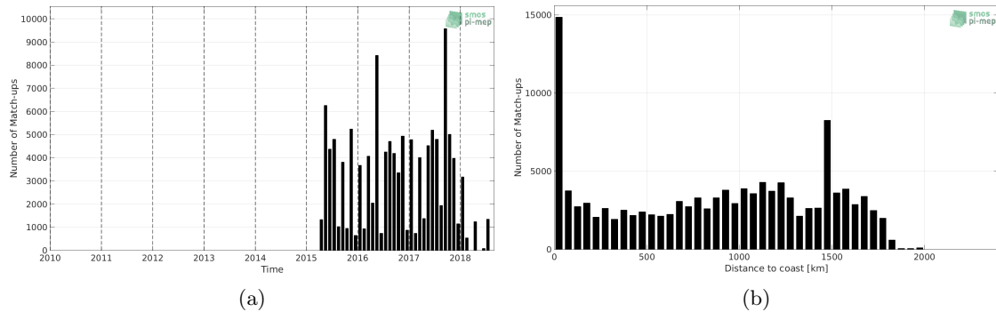
Figure 1: Number of match-ups between TSG-LEGOS-DM and SMAP-L3-JPL-V4.2-MONTHLY-60KM SSS as a function of time (a) and as function of the distance to coast (b) over the Amazon and Orinoco river plumes Pi-MEP region and for the full satellite product period.
