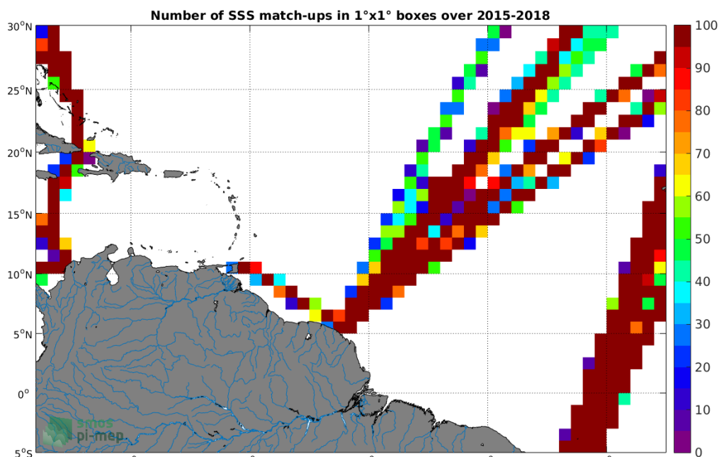
Figure 4: Number of SSS match-ups between TSG-LEGOS-DM SSS and the SMAP-L3-JPL-V4.2-MONTHLY-60KM SSS product for the Amazon and Orinoco river plumes Pi-MEP region over 1°x1° boxes and for the full satellite product period.
