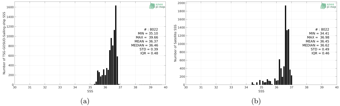
Figure 2: Histograms of SSS from TSG-GOSUD-Sailing-ship (a) and SMAP-L3-JPL-V4.2-MONTHLY-60KM (b) considering all match-up pairs per bins of 0.1 over the Amazon and Orinoco river plumes Pi-MEP region and for the full satellite product period.
