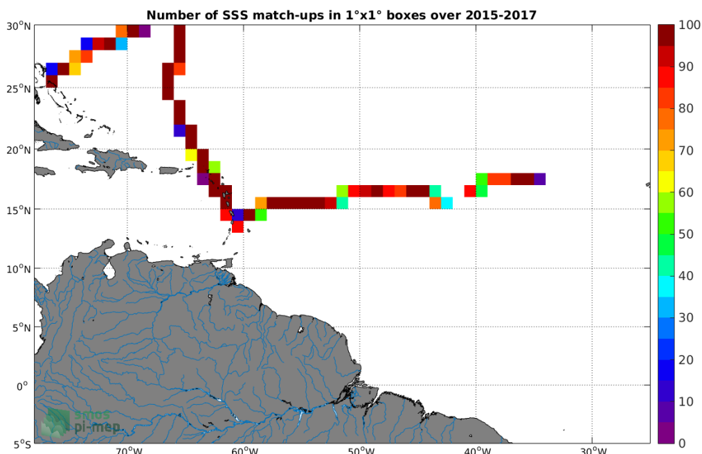
Figure 4: Number of SSS match-ups between TSG-GOSUD-Sailing-ship SSS and the SMAP-L3-JPL-V4.2-MONTHLY-60KM SSS product for the Amazon and Orinoco river plumes Pi-MEP region over 1°x1° boxes and for the full satellite product period.
