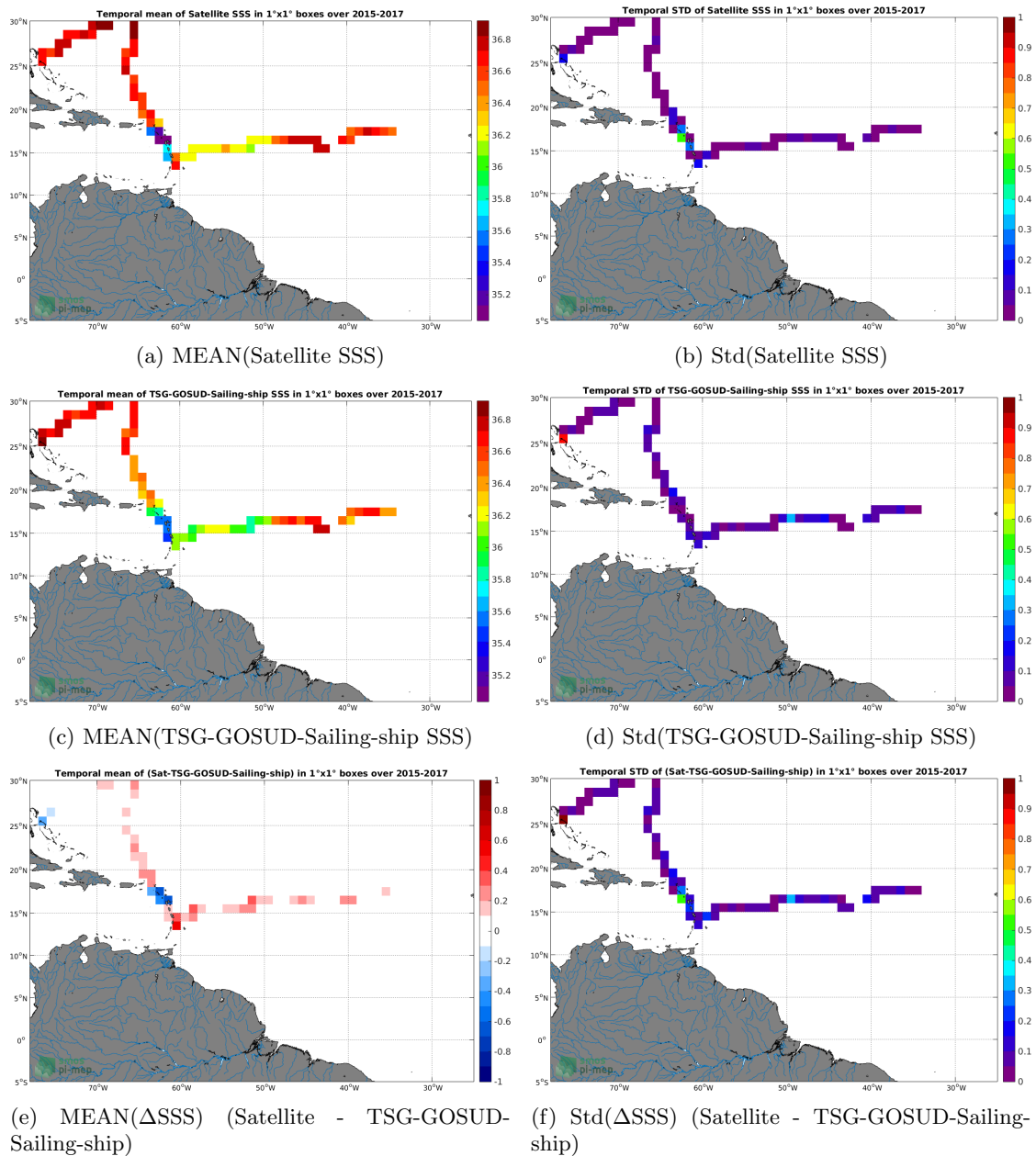
Figure 6: Temporal mean (left) and Std (right) of SSS from SMAP-L3-JPL-V4.2-MONTHLY-60KM (top), TSG-GOSUD-Sailing-ship (middle), and of \Delta SSS (Satellite - TSG-GOSUD-Sailing-ship). Only match-up pairs are used to generate these maps.
