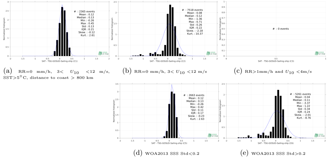
Figure 13: Normalized histogram of \Delta SSS (SMAP-L3-JPL-V4.2-MONTHLY-60KM - TSG-GOSUD-Sailing-ship) for 5 different subdatasets corresponding to: RR=0 mm/h, 3 < U_{10} < 12 m/s, SST>5°C, distance to coast > 800 km (a), RR=0 mm/h, 3 < U_{10} < 12 m/s (b), RR>1mm/h and U_{10} < 4 m/s (c), WOA2013 SSS Std<0.2 (d), WOA2013 SSS Std>0.2 (e).
