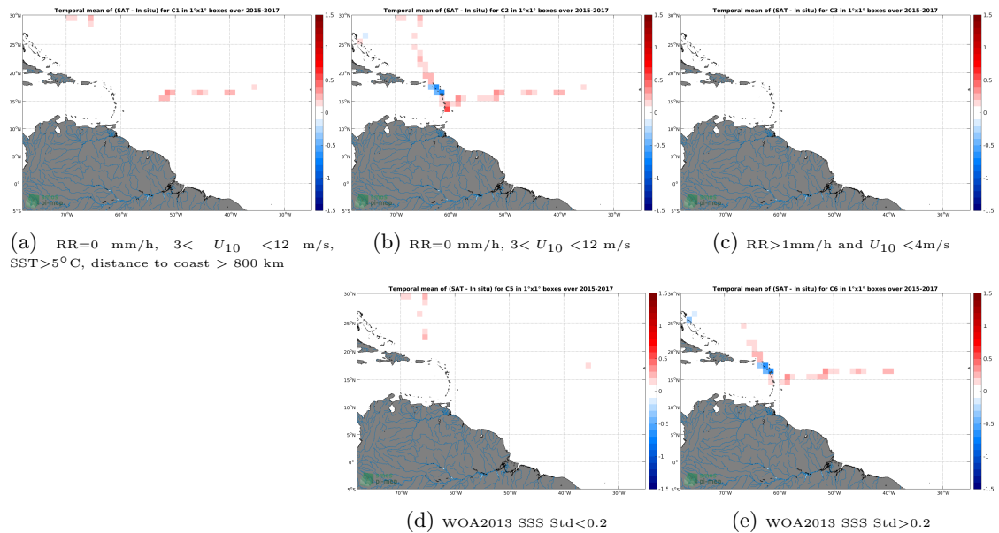
Figure 12: Temporal mean gridded over spatial boxes of size 1^\circ \times 1^\circ of \Delta SSS (SMAP-L3-JPL-V4.2-MONTHLY-60KM - TSG-GOSUD-Sailing-ship) for 5 different subdatasets corresponding to:RR=0 mm/h, 3 < U_{10} < 12 m/s, SST >5^\circ C, distance to coast > 800 km (a), RR=0 mm/h, 3 < U_{10} < 12 m/s (b), RR >1 mm/h and U_{10} < 4 m/s (c), WOA2013 SSS Std <0.2 (d), WOA2013 SSS Std >0.2 (e).
