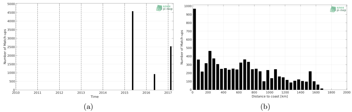
Figure 1: Number of match-ups between TSG-GOSUD-Sailing-ship and SMAP-L3-JPL-V4.2-MONTHLY-60KM SSS as a function of time (a) and as function of the distance to coast (b) over the Amazon and Orinoco river plumes Pi-MEP region and for the full satellite product period.
