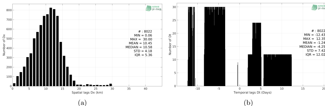
Figure 5: Histograms of the spatial (a) and temporal (b) lags between the time of the TSG-GOSUD-Sailing-ship measurements and the date of the corresponding SMAP-L3-JPL-V4.2-MONTHLY-60KM SSS product.
