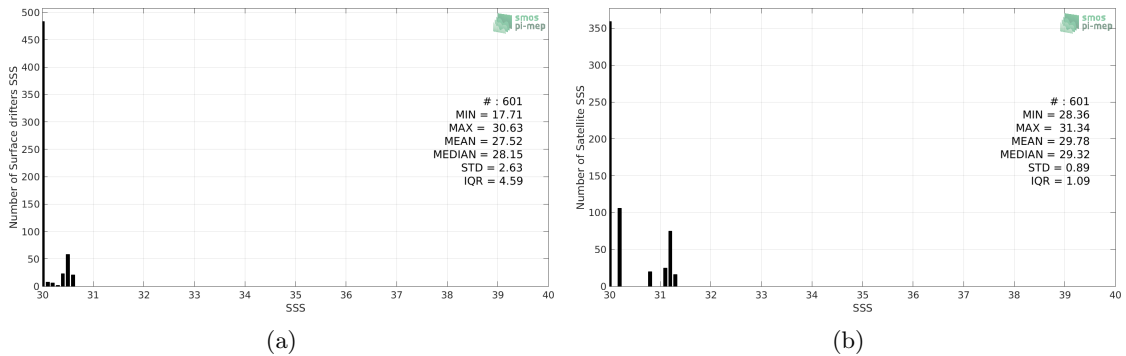
Figure 2: Histograms of SSS from Surface drifters (a) and SMAP-L3-JPL-V4.2-MONTHLY-60KM (b) considering all match-up pairs per bins of 0.1 over the Amazon and Orinoco river plumes Pi-MEP region and for the full satellite product period.
