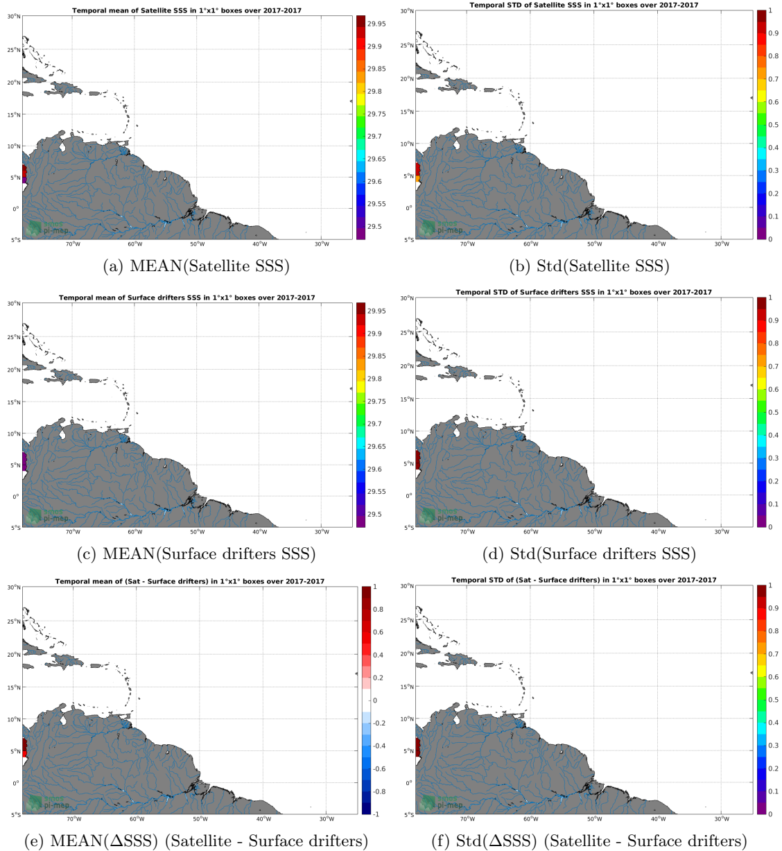
Figure 5: Temporal mean (left) and Std (right) of SSS from SMAP-L3-JPL-V4.2-MONTHLY-60KM (top), Surface drifters (middle), and of \Delta SSS (Satellite - Surface drifters). Only match-up pairs are used to generate these maps.
