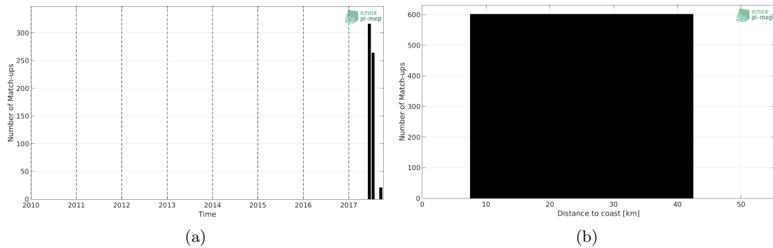
Figure 1: Number of match-ups between Surface drifters and SMAP-L3-JPL-V4.2-MONTHLY-60KM SSS as a function of time (a) and as function of the distance to coast (b) over the Amazon and Orinoco river plumes Pi-MEP region and for the full satellite product period.
