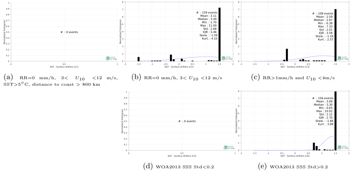
Figure 12: Normalized histogram of \Delta SSS (SMAP-L3-JPL-V4.2-MONTHLY-60KM - Surface drifters) for 5 different subdatasets corresponding to: RR=0 mm/h, 3 < U_{10} < 12 m/s, SST > 5°C, distance to coast > 800 km (a), RR=0 mm/h, 3 < U_{10} < 12 m/s (b), RR > 1mm/h and U_{10} < 4 m/s (c), WOA2013 SSS Std < 0.2 (d), WOA2013 SSS Std > 0.2 (e).
