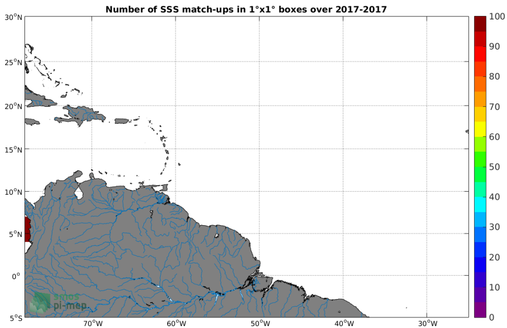
Figure 3: Number of SSS match-ups between Surface drifters SSS and the SMAP-L3-JPL-V4.2-MONTHLY-60KM SSS product for the Amazon and Orinoco river plumes Pi-MEP region over 1°x1° boxes and for the full satellite product period.
