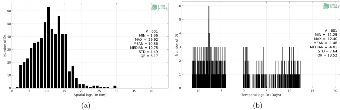
Figure 4: Histograms of the spatial (a) and temporal (b) lags between the time of the Surface drifters measurements and the date of the corresponding SMAP-L3-JPL-V4.2-MONTHLY-60KM SSS product.
