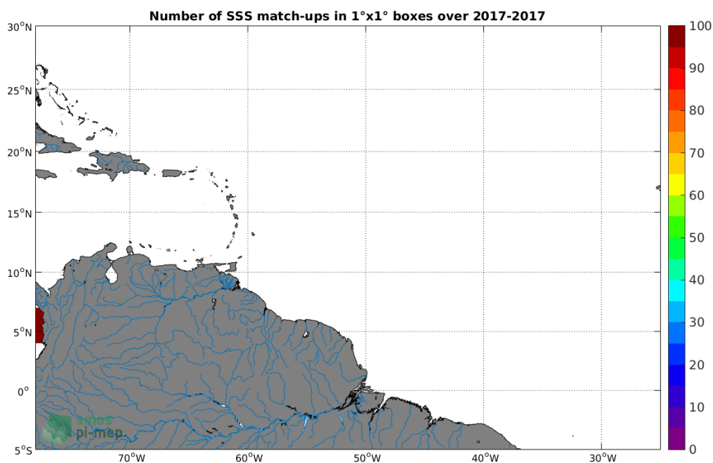
Figure 3: Number of SSS match-ups between Surface drifters SSS and the SMAP-L3-JPL-V4.2-MONTHLY-60KM SSS product for the Amazon and Orinoco river plumes Pi-MEP region over 1^{\circ} \times 1^{\circ} boxes and for the full satellite product period.
