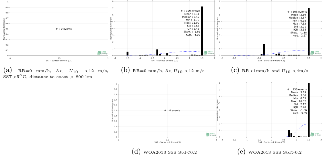
Figure 12: Normalized histogram of \Delta\text{SSS} (SMAP-L3-JPL-V4.2-MONTHLY-60KM - Surface drifters) for 5 different subdatasets corresponding to: RR=0 mm/h, 3 < U_{10} < 12 m/s, SST > 5^\circ\text{C} , distance to coast > 800 km (a), RR=0 mm/h, 3 < U_{10} < 12 m/s (b), RR > 1\text{mm/h} and U_{10} < 4\text{m/s} (c), WOA2013 SSS Std < 0.2 (d), WOA2013 SSS Std > 0.2 (e).
