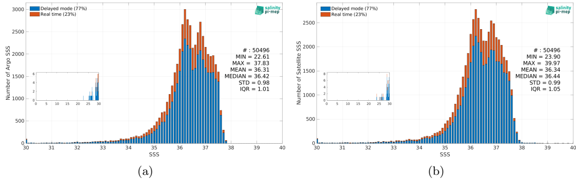
Figure 3: Histograms of SSS from Argo (a) and SMAP SSS L2-AVERAGED v6 (RSS) (b) considering all match-up pairs per bins of 0.1 over the Amazon and Orinoco river plumes Pi-MEP region and for the full satellite product period.
