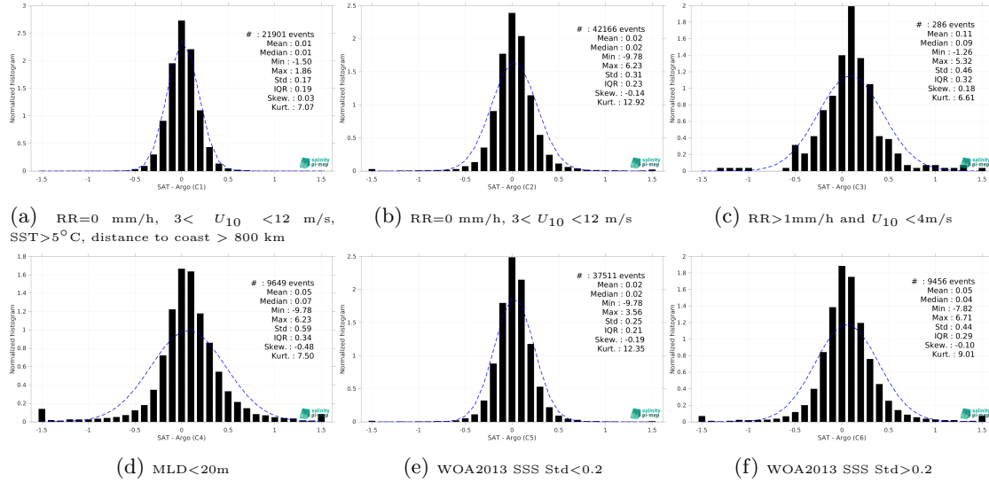
Figure 15: Normalized histogram of \Delta\text{SSS} (SMAP SSS L2-AVERAGED v6 (RSS) - Argo) for 6 different subdatasets corresponding to: RR=0 mm/h, 3 < U_{10} < 12 m/s, SST>5°C, distance to coast > 800 km (a), RR=0 mm/h, 3 < U_{10} < 12 m/s (b), RR>1mm/h and U_{10} < 4 m/s (c), MLD<20m (d), WOA2013 SSS Std<0.2 (e), WOA2013 SSS Std>0.2 (f).
