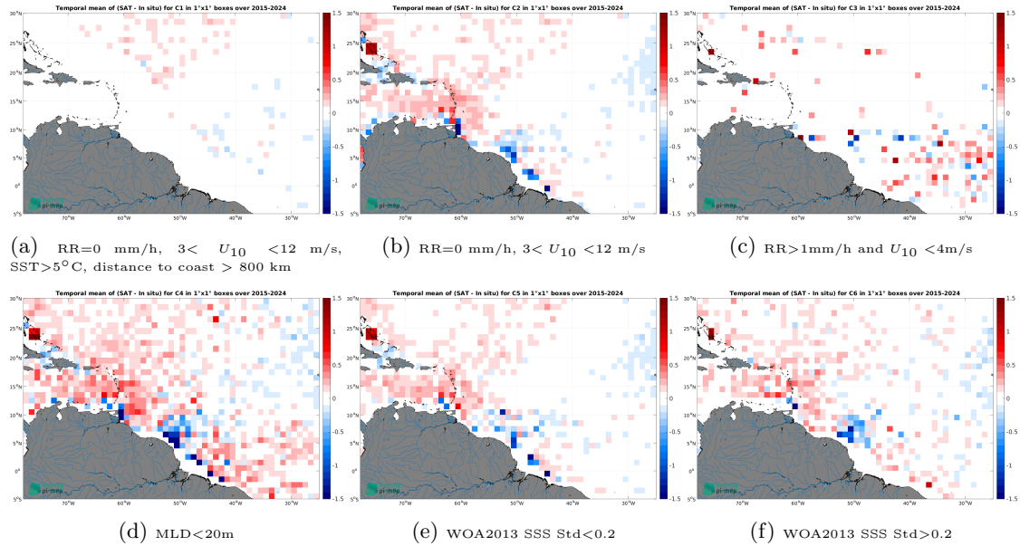
Figure 14: Temporal mean gridded over spatial boxes of size 1^\circ \times 1^\circ of \Delta SSS (SMAP SSS L2-AVERAGED v6 (RSS) - Argo) for 6 different subdatasets corresponding to: RR=0 mm/h, 3 < U_{10} < 12 m/s, SST > 5^\circ C , distance to coast > 800 km (a), RR=0 mm/h, 3 < U_{10} < 12 m/s (b), RR > 1 mm/h and U_{10} < 4 m/s (c), MLD < 20 m (d), WOA2013 SSS Std < 0.2 (e), WOA2013 SSS Std > 0.2 (f).
