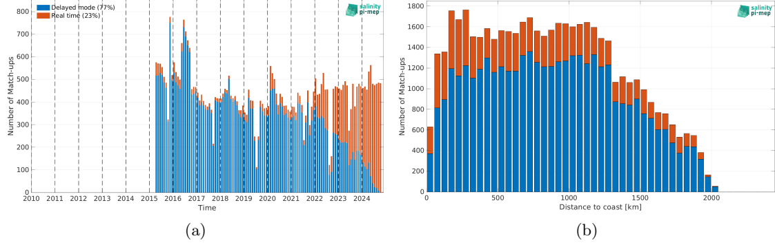
Figure 2: Number of match-ups between Argo and SMAP SSS L2-AVERAGED v6 (RSS) SSS as a function of time (a) and as function of the distance to coast (b) over the Amazon and Orinoco river plumes Pi-MEP region and for the full satellite product period.
