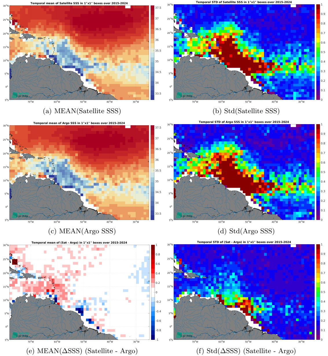
Figure 7: Temporal mean (left) and Std (right) of SSS from SMAP SSS L2-AVERAGED v6 (RSS) (top), Argo (middle), and of \Delta SSS (Satellite - Argo). Only match-up pairs are used to generate these maps.
