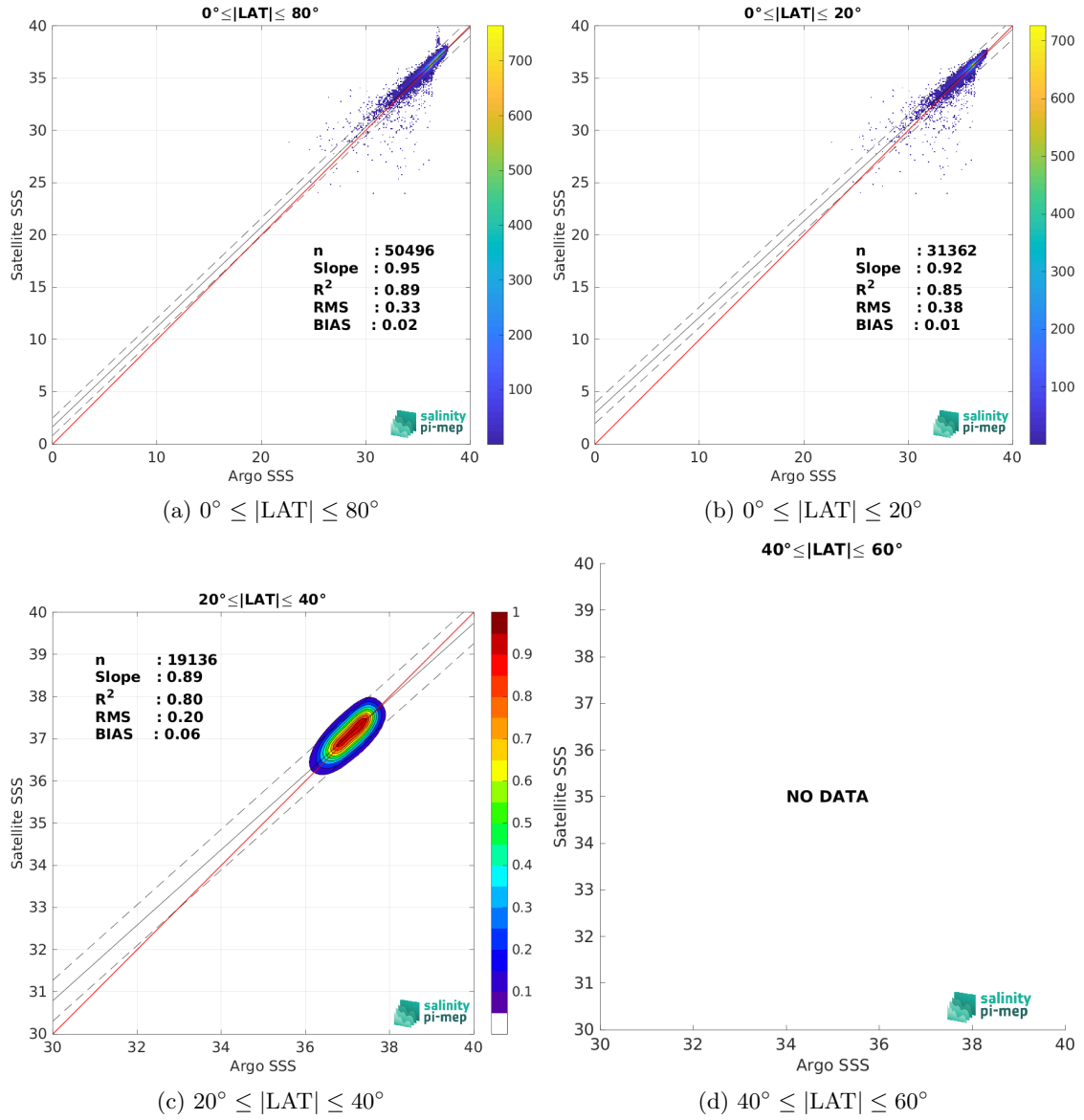
Figure 10: Contour maps of the concentration of SMAP SSS L2-AVERAGED v6 (RSS) SSS (y-axis) versus Argo SSS (x-axis) at match-up pairs for different latitude bands. For each plot, the red line shows x=y . The black thin and dashed lines indicate a linear fit through the data cloud and the \pm 95\% confidence levels, respectively. The number match-up pairs n , the slope and R^2 coefficient of the linear fit, the root mean square (RMS) and the mean bias between satellite and in situ data are indicated for each latitude band in each plots.
