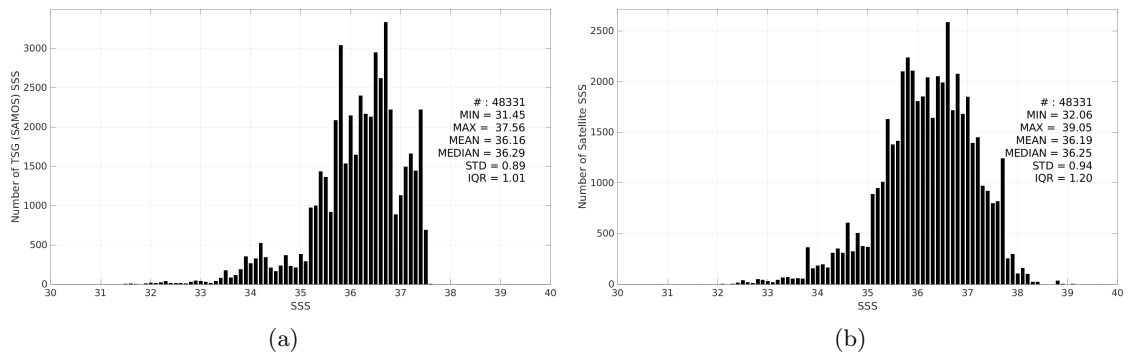
Figure 3: Histograms of SSS from TSG (SAMOS) (a) and SMAP SSS L2 v6 (RSS) (b) considering all match-up pairs per bins of 0.1 over the Amazon and Orinoco river plumes Pi-MEP region and for the full satellite product period.
