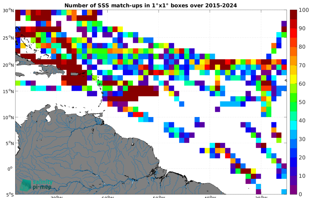
Figure 5: Number of SSS match-ups between TSG (SAMOS) SSS and the SMAP SSS L2 v6 (RSS) SSS product for the Amazon and Orinoco river plumes Pi-MEP region over 1^\circ \times 1^\circ boxes and for the full satellite product period.
