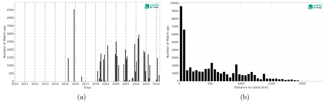
Figure 2: Number of match-ups between TSG (SAMOS) and SMAP SSS L2 v6 (RSS) SSS as a function of time (a) and as function of the distance to coast (b) over the Amazon and Orinoco river plumes Pi-MEP region and for the full satellite product period.
