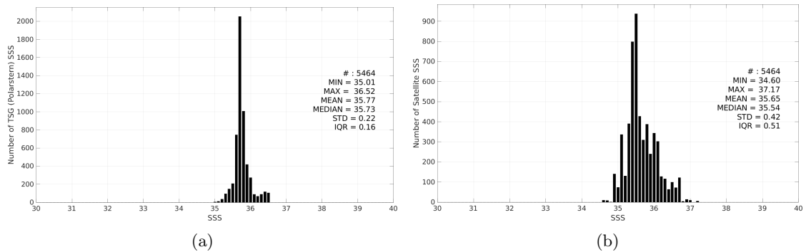
Figure 3: Histograms of SSS from TSG (Polarstern) (a) and SMAP SSS L2 v6 (RSS) (b) considering all match-up pairs per bins of 0.1 over the Amazon and Orinoco river plumes Pi-MEP region and for the full satellite product period.
