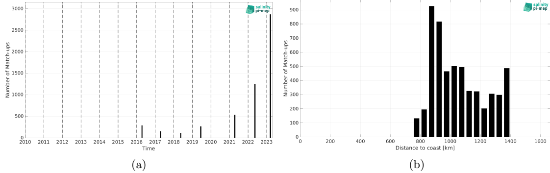
Figure 2: Number of match-ups between TSG (Polarstern) and SMAP SSS L2 v6 (RSS) SSS as a function of time (a) and as function of the distance to coast (b) over the Amazon and Orinoco river plumes Pi-MEP region and for the full satellite product period.
