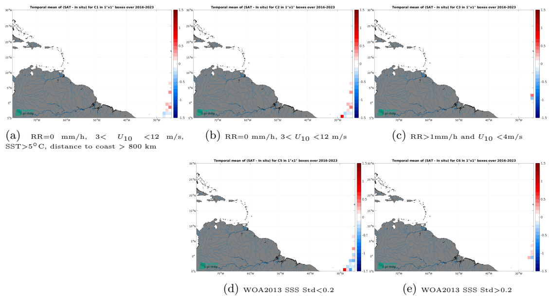
Figure 14: Temporal mean gridded over spatial boxes of size 1^\circ \times 1^\circ of \Delta SSS (SMAP SSS L2 v6 (RSS) - TSG (Polarstern)) for 5 different subdatasets corresponding to:RR=0 mm/h, 3 < U_{10} < 12 m/s, SST >5^\circ\text{C} , distance to coast > 800 km (a), RR=0 mm/h, 3 < U_{10} < 12 m/s (b), RR >1 mm/h and U_{10} < 4 m/s (c), WOA2013 SSS Std <0.2 (d), WOA2013 SSS Std >0.2 (e).
