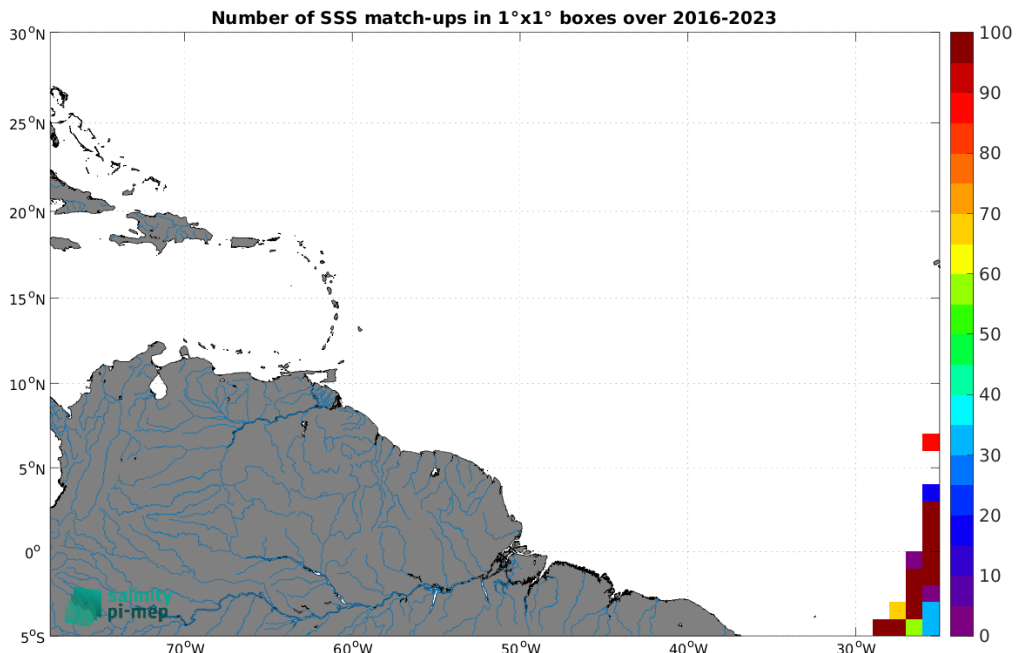
Figure 5: Number of SSS match-ups between TSG (Polarstern) SSS and the SMAP SSS L2 v6 (RSS) SSS product for the Amazon and Orinoco river plumes Pi-MEP region over 1^\circ \times 1^\circ boxes and for the full satellite product period.
