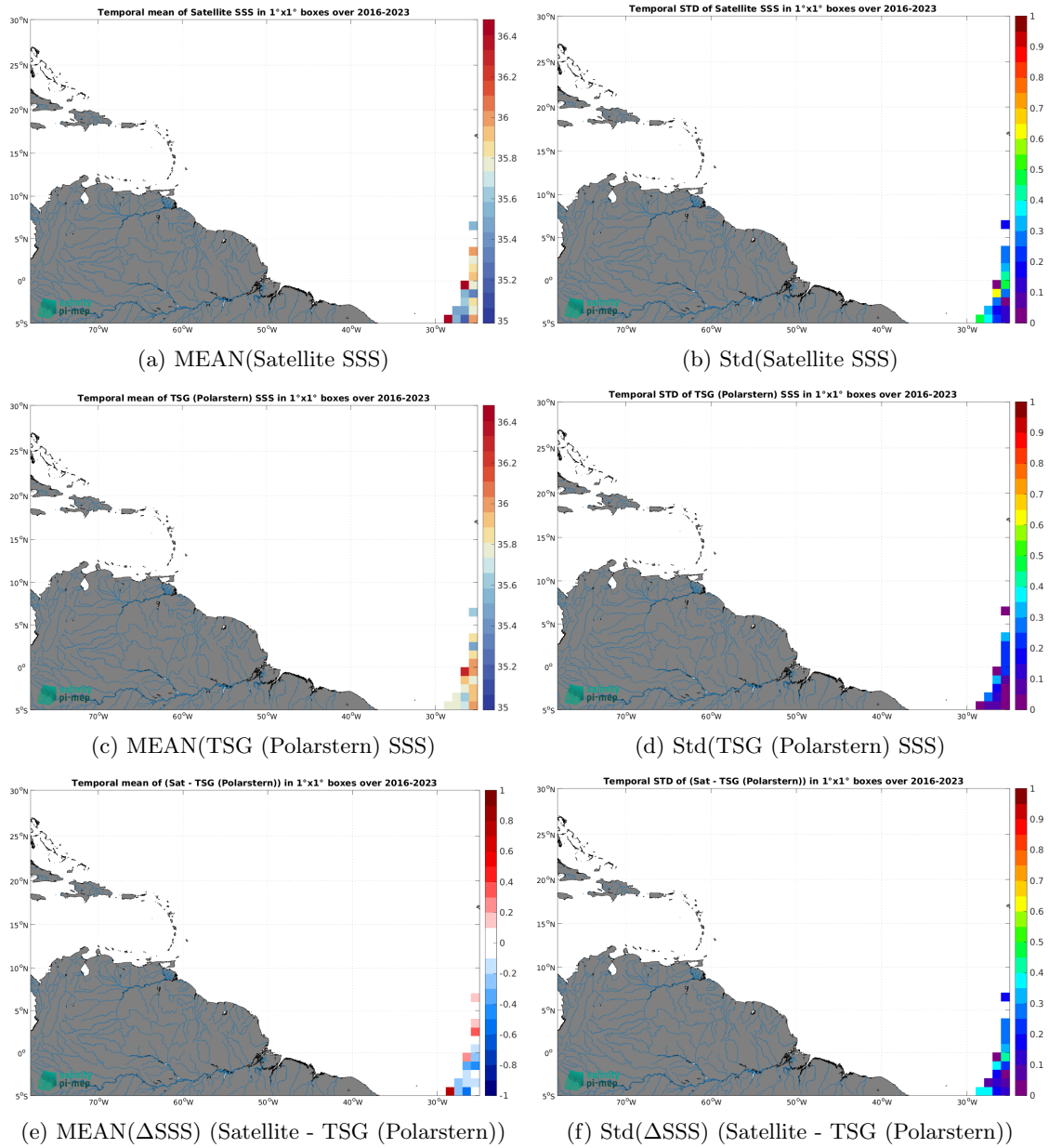
Figure 7: Temporal mean (left) and Std (right) of SSS from SMAP SSS L2 v6 (RSS) (top), TSG (Polarstern) (middle), and of \Delta SSS (Satellite - TSG (Polarstern)). Only match-up pairs are used to generate these maps.
