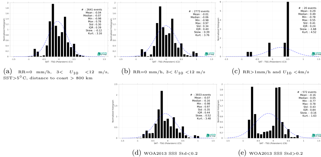
Figure 15: Normalized histogram of \Delta SSS (SMAP SSS L2 v6 (RSS) - TSG (Polarstern)) for 5 different subdatasets corresponding to: RR=0 mm/h, 3 < U_{10} < 12 m/s, SST > 5°C, distance to coast > 800 km (a), RR=0 mm/h, 3 < U_{10} < 12 m/s (b), RR > 1mm/h and U_{10} < 4 m/s (c), WOA2013 SSS Std < 0.2 (d), WOA2013 SSS Std > 0.2 (e).
