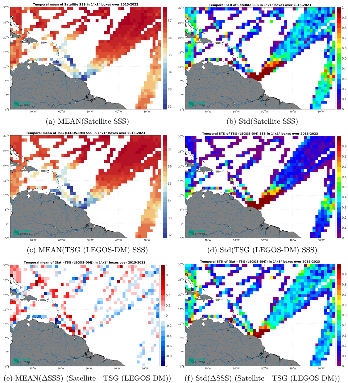
Figure 7: Temporal mean (left) and Std (right) of SSS from SMAP SSS L2 v6 (RSS) (top), TSG (LEGOS-DM) (middle), and of \Delta SSS (Satellite - TSG (LEGOS-DM)). Only match-up pairs are used to generate these maps.
