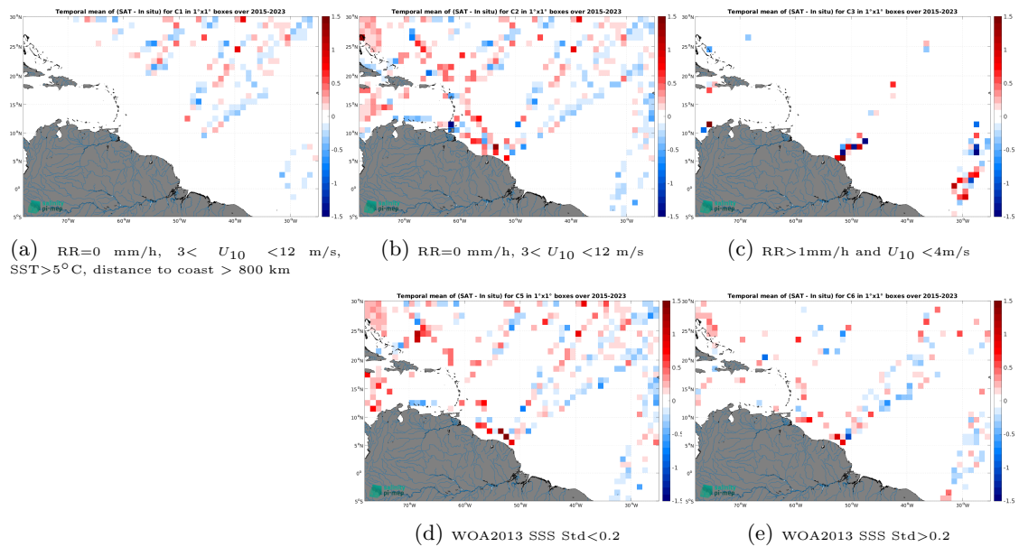
Figure 14: Temporal mean gridded over spatial boxes of size 1^\circ \times 1^\circ of \Delta\text{SSS} (SMAP SSS L2 v6 (RSS) - TSG (LEGOS-DM)) for 5 different subdatasets corresponding to:RR=0 mm/h, 3 < U_{10} < 12 m/s, SST >5^\circ\text{C} , distance to coast > 800 km (a), RR=0 mm/h, 3 < U_{10} < 12 m/s (b), RR >1 mm/h and U_{10} < 4 m/s (c), WOA2013 SSS Std <0.2 (d), WOA2013 SSS Std >0.2 (e).
