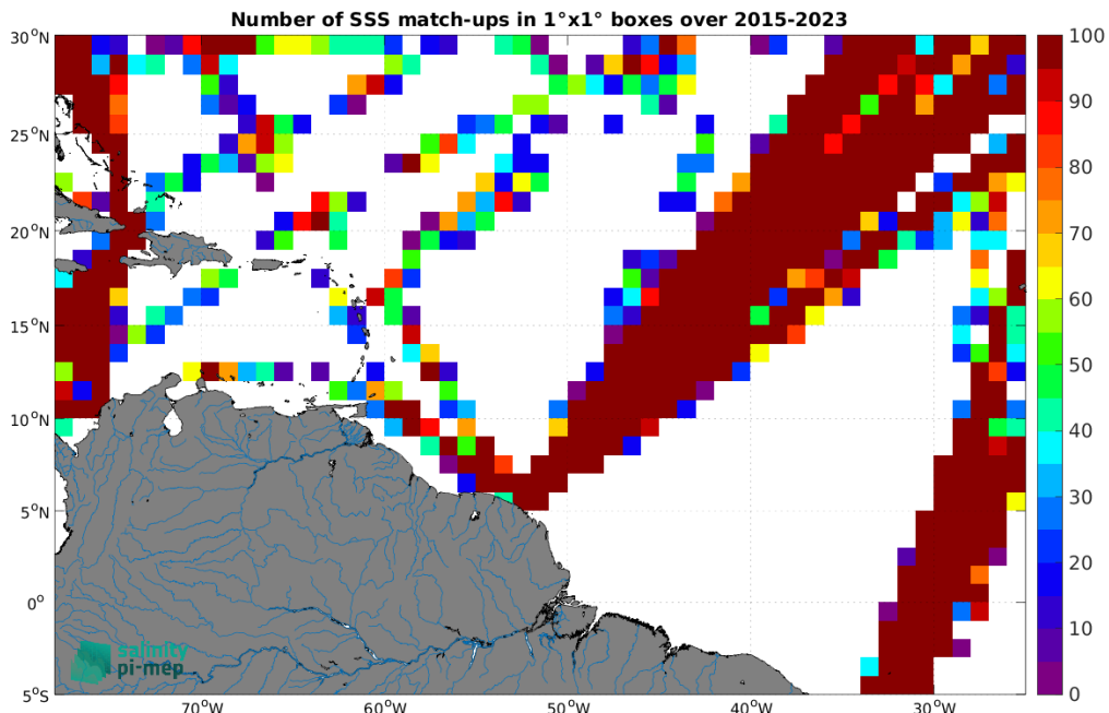
Figure 5: Number of SSS match-ups between TSG (LEGOS-DM) SSS and the SMAP SSS L2 v6 (RSS) SSS product for the Amazon and Orinoco river plumes Pi-MEP region over 1^\circ \times 1^\circ boxes and for the full satellite product period.
