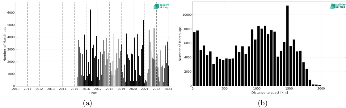
Figure 2: Number of match-ups between TSG (LEGOS-DM) and SMAP SSS L2 v6 (RSS) SSS as a function of time (a) and as function of the distance to coast (b) over the Amazon and Orinoco river plumes Pi-MEP region and for the full satellite product period.
