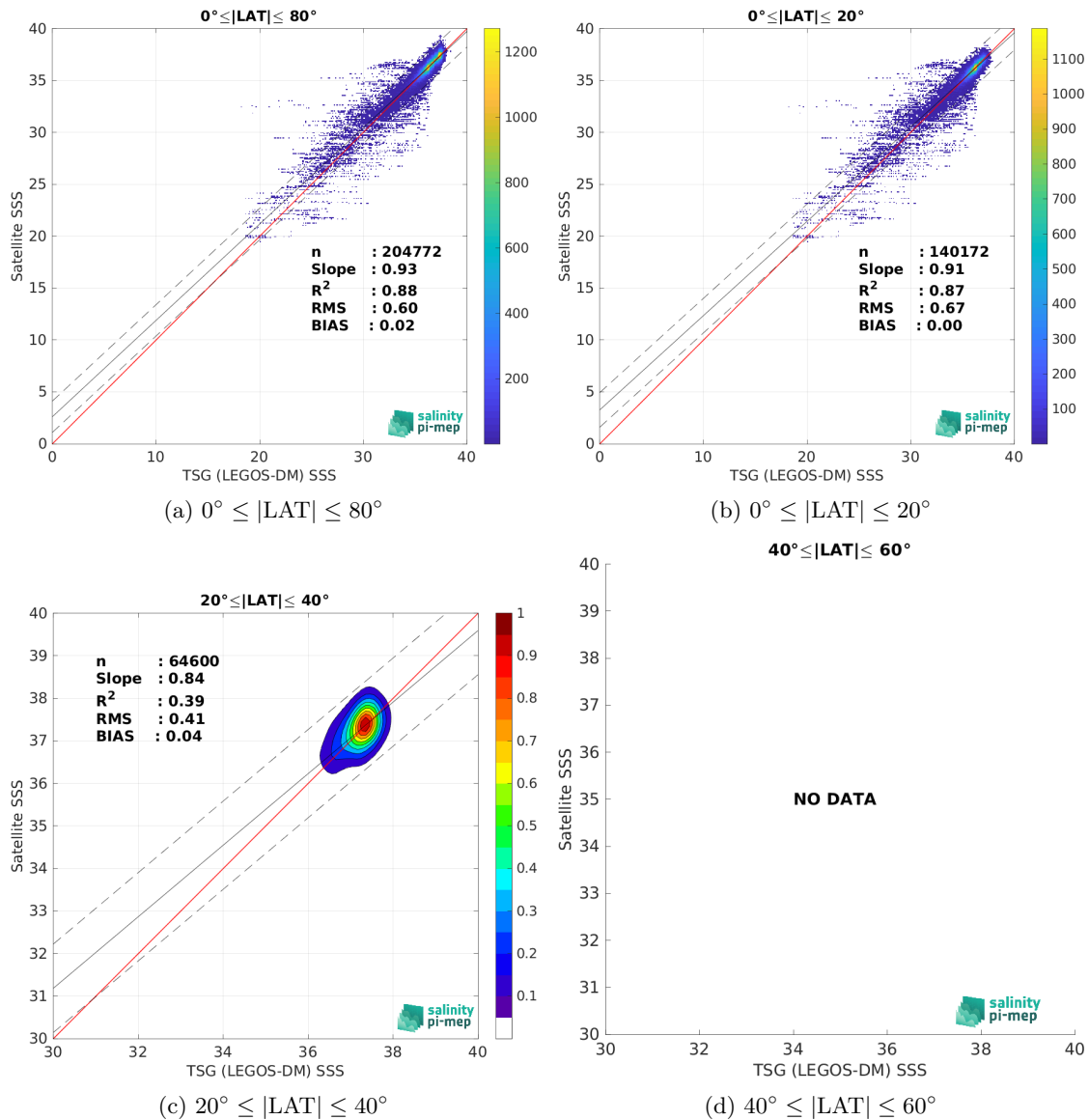
Figure 10: Contour maps of the concentration of SMAP SSS L2 v6 (RSS) SSS (y-axis) versus TSG (LEGOS-DM) SSS (x-axis) at match-up pairs for different latitude bands. For each plot, the red line shows x=y . The black thin and dashed lines indicate a linear fit through the data cloud and the \pm 95\% confidence levels, respectively. The number match-up pairs n , the slope and R^2 coefficient of the linear fit, the root mean square (RMS) and the mean bias between satellite and in situ data are indicated for each latitude band in each plots.
