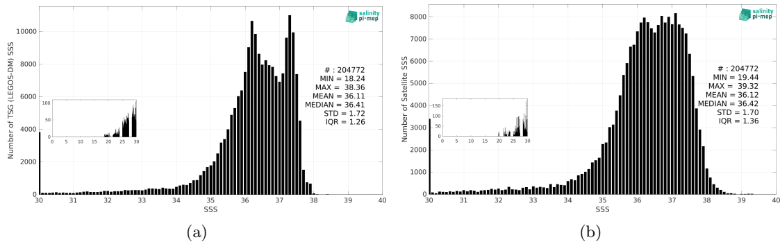
Figure 3: Histograms of SSS from TSG (LEGOS-DM) (a) and SMAP SSS L2 v6 (RSS) (b) considering all match-up pairs per bins of 0.1 over the Amazon and Orinoco river plumes Pi-MEP region and for the full satellite product period.
