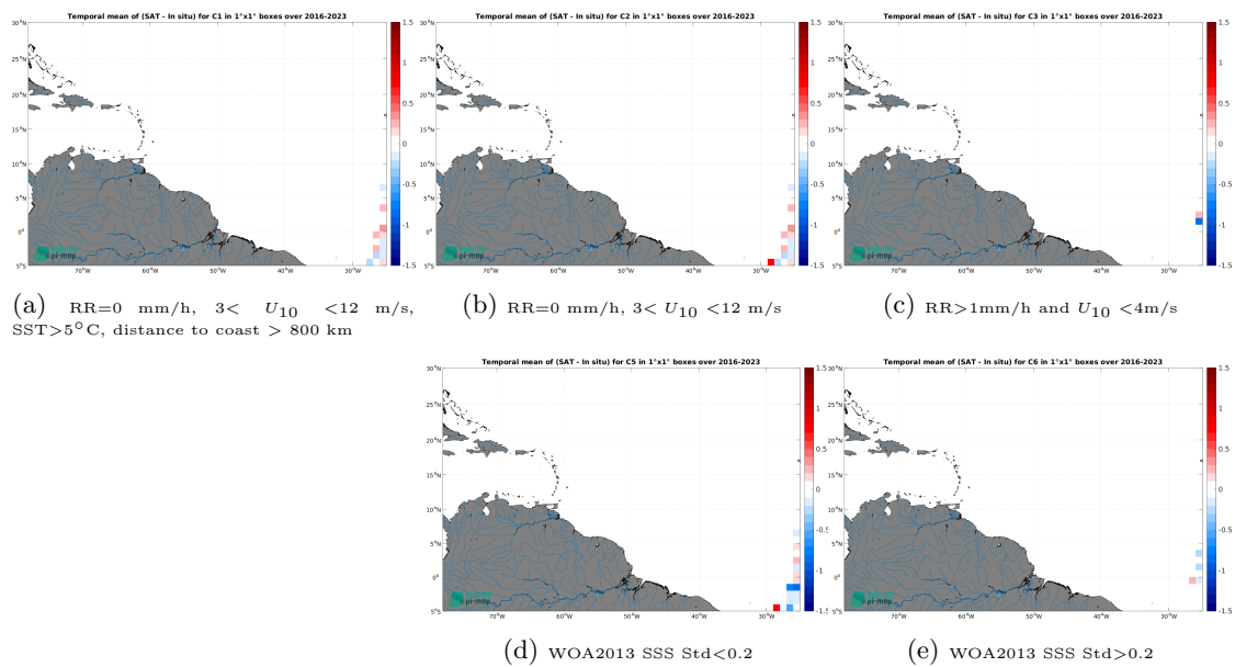
Figure 14: Temporal mean gridded over spatial boxes of size 1^\circ \times 1^\circ of \Delta SSS (SMAP SSS L2 v6 - 40 km (RSS) - TSG (Polarstern)) for 5 different subdatasets corresponding to:RR=0 mm/h, 3 < U_{10} < 12 m/s, SST >5^\circ\text{C} , distance to coast > 800 km (a), RR=0 mm/h, 3 < U_{10} < 12 m/s (b), RR >1 mm/h and U_{10} < 4 m/s (c), WOA2013 SSS Std <0.2 (d), WOA2013 SSS Std >0.2 (e).
