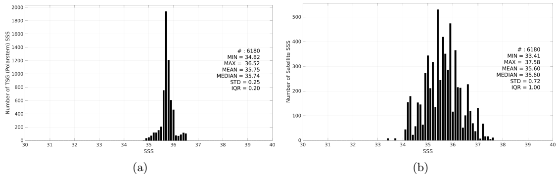
Figure 3: Histograms of SSS from TSG (Polarstern) (a) and SMAP SSS L2 v6 - 40 km (RSS) (b) considering all match-up pairs per bins of 0.1 over the Amazon and Orinoco river plumes Pi-MEP region and for the full satellite product period.
