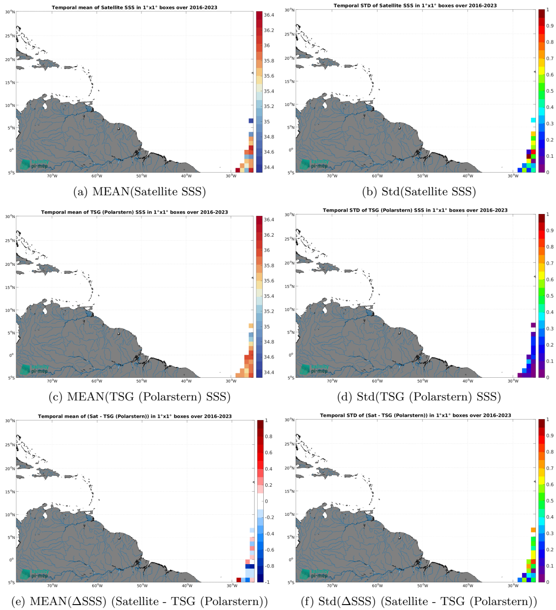
Figure 7: Temporal mean (left) and Std (right) of SSS from SMAP SSS L2 v6 - 40 km (RSS) (top), TSG (Polarstern) (middle), and of \Delta SSS (Satellite - TSG (Polarstern)). Only match-up pairs are used to generate these maps.
